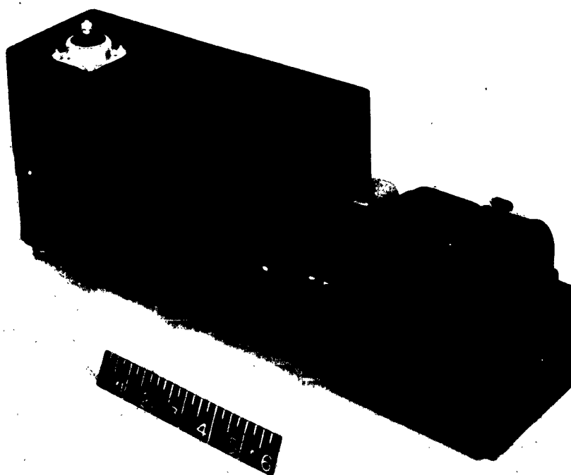
Figure 4. Thyatron Chassis
