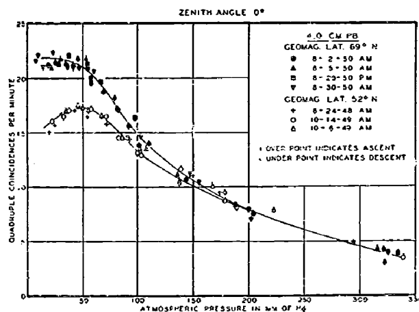
FIG. 4. Intensity vs altitude curves, obtained with coincidence-counter trains containing 4 cm of Pb, for cosmic rays arriving vertically at \lambda = 52^\circ N and \lambda = 69^\circ N. The maximum disappears at the more northern station.
