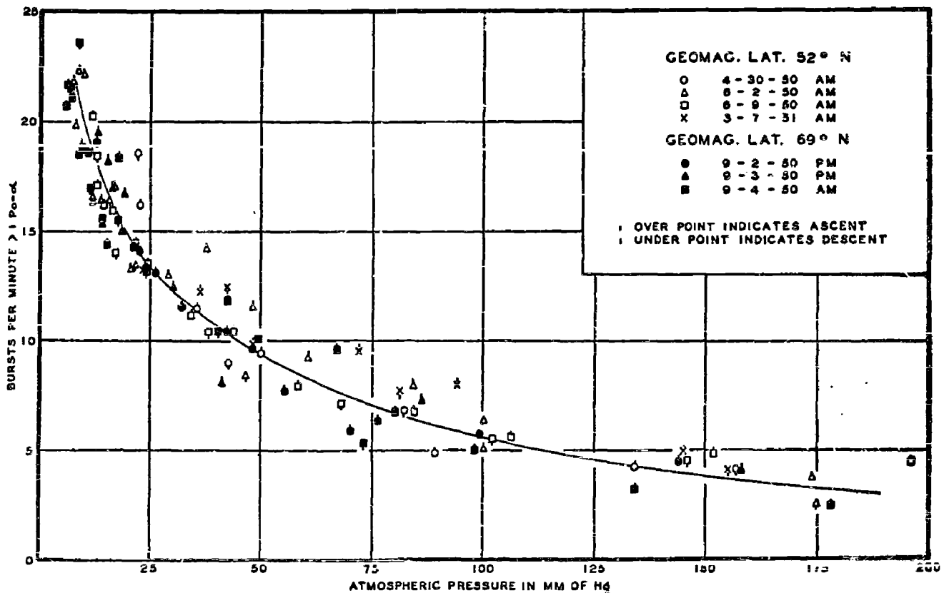
FIG. 6. Dependence of burst-rate upon altitude, as measured by ionization chambers biased to record events > 1.0 Po- \alpha . No variation with latitude north of \lambda = 52^\circ is revealed.
