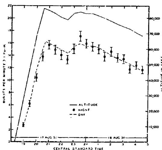
FIG. 1. Altitude vs time curve (solid line) for night flight at geomagnetic latitude 55^\circ\text{N} and counting rates (solid circles) obtained with ionization chamber biased to record bursts \geq 1 \text{ Po}-\alpha . Counting rates averaged from four daytime flights (dashed curve) at corresponding altitudes show no significant deviations from night rates.
