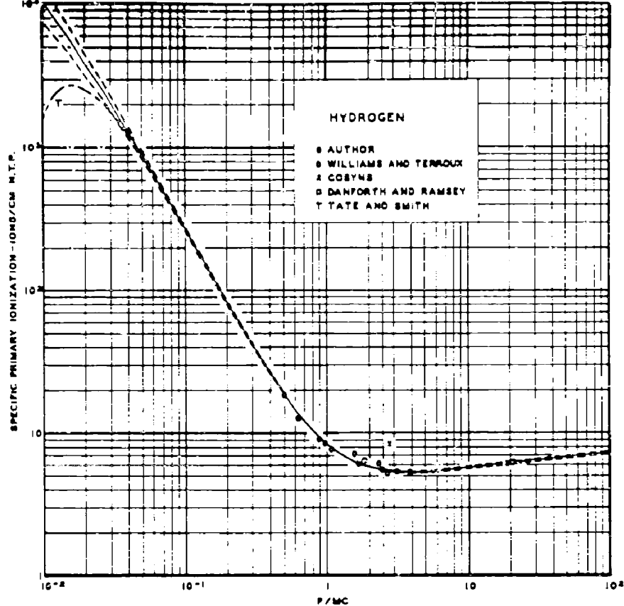
Fig. 3. - Composite plot of the present hydrogen data together with the results of Williams and Terroux 1) , Tate and Smith 3) , Danforth and Ramsey 4) , and Cosyns 5,6) . Curves — and - - - are theoretical.
