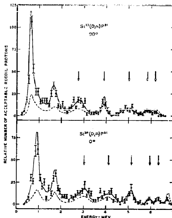
FIG. 3. Recoil protons of the neutrons emitted in the reaction \text{Si}^{30}(d,n)\text{P}^{31} .
