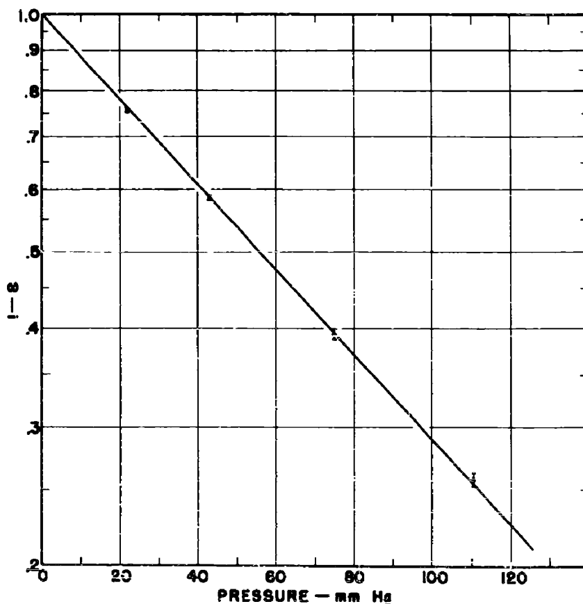
Fig. 2. - Variation of the quantity (1-E) as a function of the pressure of H_2 contained in counter C_1 . (.855 Mev. \beta -rays)
