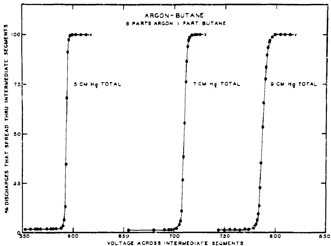
Figure 2 - Probability of discharge spread in Argon-Butane
