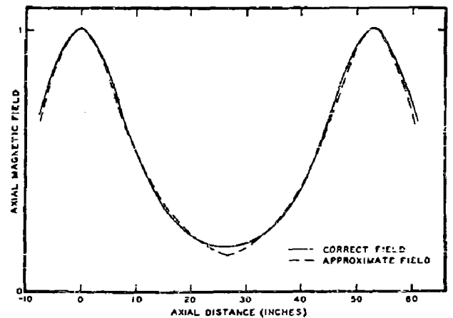
FIG. 2. Axial magnetic fields. (a) From -\infty < x < 2.5 , h = 1/(1+x^2) , from 2.5 < x < \infty , h = 1/[1+(x-2.5)^2] . (b) Magnetic field, normalized to unity at x=0 , calculated for the coils shown in Fig. 1 using equations in Deutsch, Elliott, and Evans, Rev. Sci. Instr. 15, 178 (1944). The coil separation is set at 5a , to coincide with (a). For the best fit with the coils shown in Fig. 1, the scale factor a was taken to be 10.60 in.
