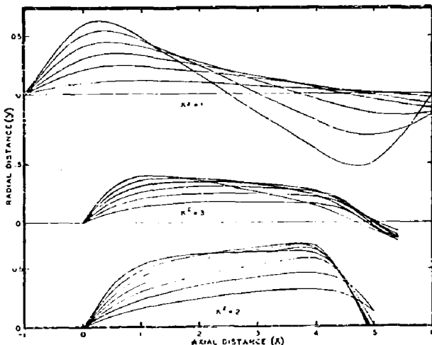
FIG. 3. Complete trajectories in the double bell-shaped axial magnetic field for k^2=2 and k^2=3 each with x_1=0 and for k^2=1 with x_1=-1.030 .
