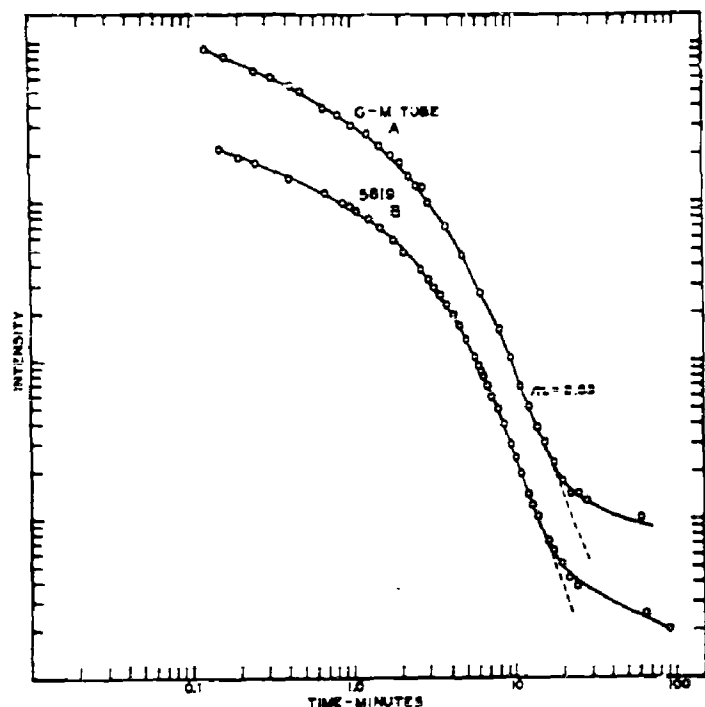
Figure 1 - Phosphorescent decay curves of \text{NaCl} + 1/2\% \text{AgCl} (polycrystalline melt) irradiated for five seconds with ultra violet light from a germicidal lamp. a. Curve A gives the decay of the lower band (2500 Å), curve B that of the upper band (4000 Å).
