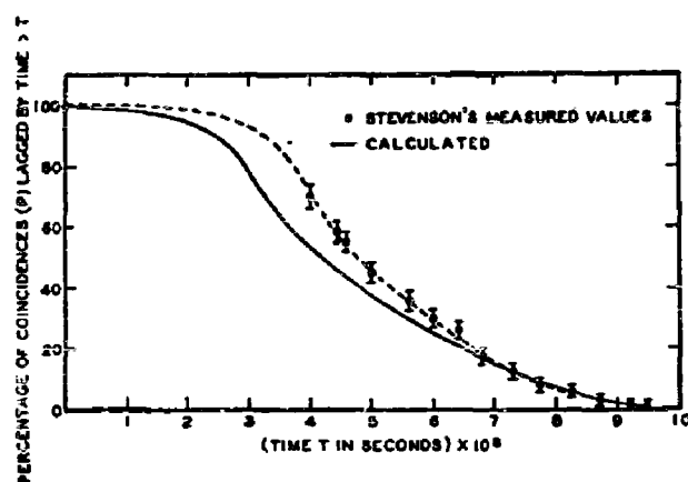
Fig. 2. Solid line calculated from P = S[1 - e^{-2\alpha k_1(r-t)}] - T[1 - e^{-2\alpha k_1(r-t)}] , where S = \epsilon a k_1 e^{-\epsilon a k_1 t} , T = \epsilon a k_1 e^{-2\epsilon a k_1 t} , \epsilon = specific ionization at atmospheric pressure; \alpha = p/p_0 where p = total pressure of gas, p_0 = atmospheric pressure; \epsilon a k_1 = average number of ions per beta-particle; v = constant velocity of 7.8 \times 10^8 cm per sec; and r = radius of counter.
