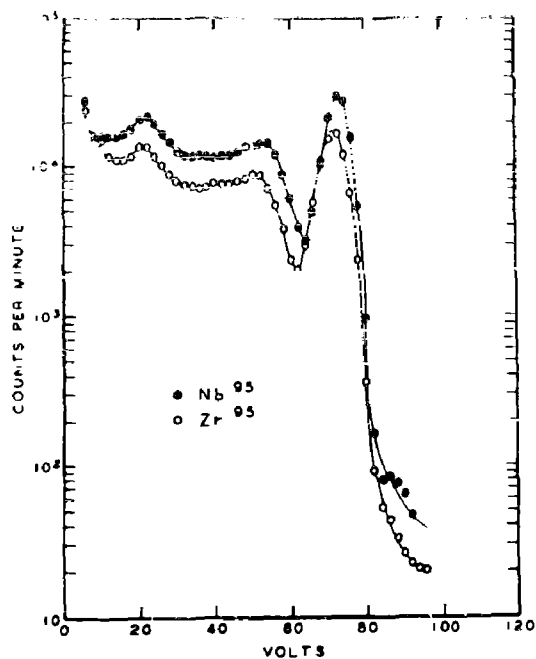
Fig. 2 Pulse height distribution of gamma rays from \text{Zr}^{95} and \text{Nb}^{95} on NaI - Tl.
