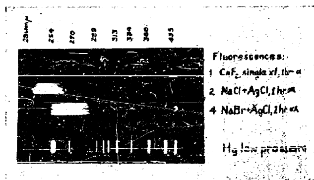
FIG. 1. Ultraviolet emission of alphas on \text{CaF}_2 , \text{NaCl-Ag} , and \text{NaBr-Ag} . This is an actual photographic reproduction of the exposed plates.
