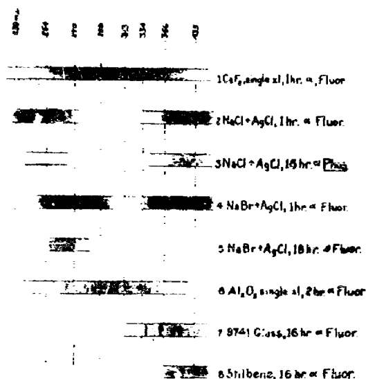
Spectrograms (drawn) of Scintillating Crystals
