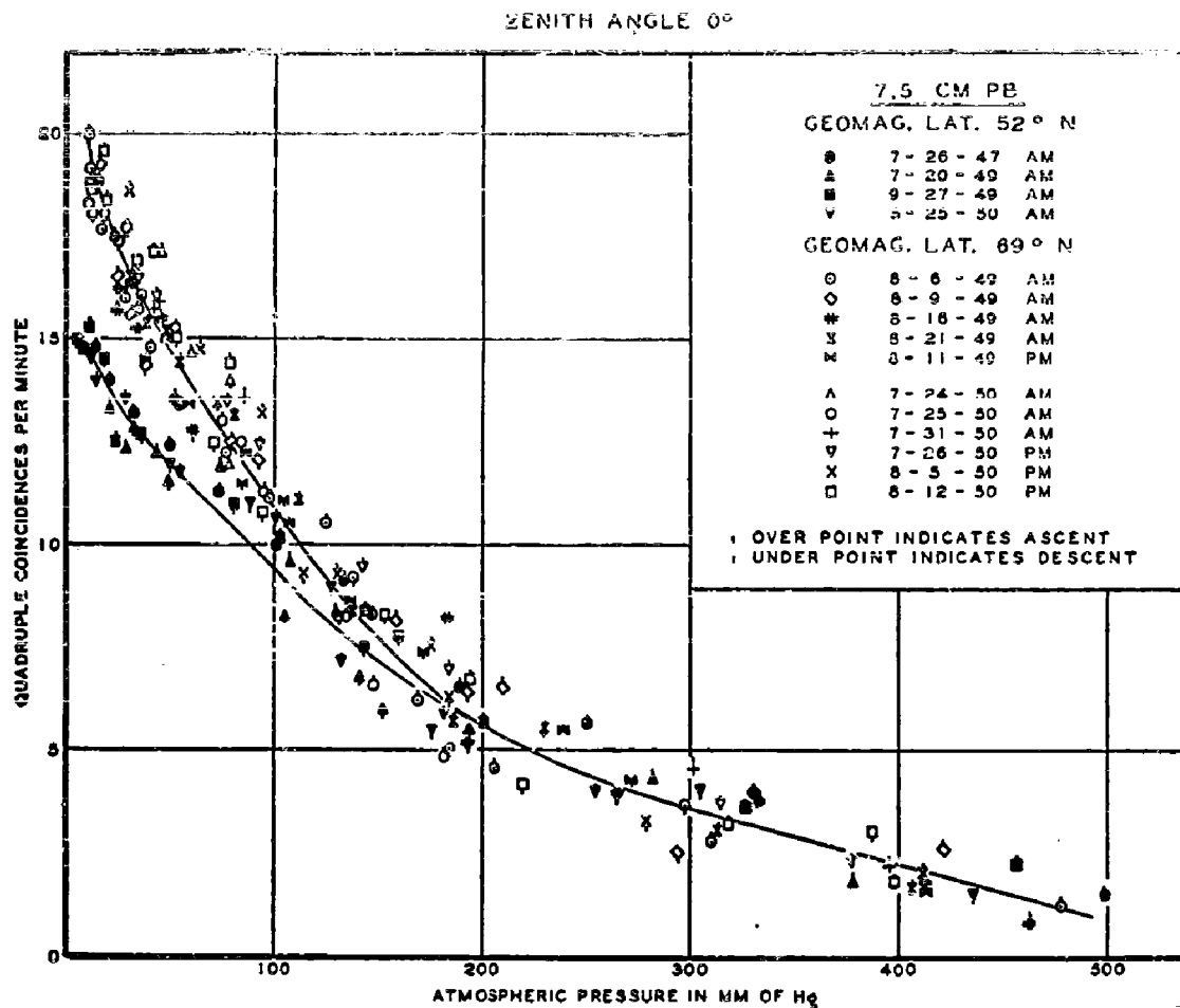
FIG. 3. Intensity vs altitude curves for cosmic rays arriving vertically, and penetrating 7.5 cm of Pb at \lambda = 52^\circ N (Swarthmore, Pennsylvania) and \lambda = 69^\circ N (Fort Churchill, Manitoba). Note the absence of detectable diurnal or temporal variations.
