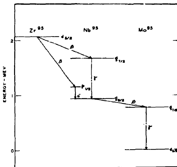
Fig. 4 Disintegration Scheme for \text{Zr}^{95} and \text{Nb}^{95} .
