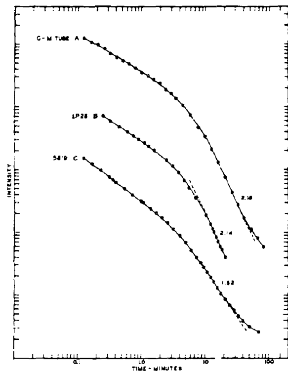
Figure 3 - Bartol polycrystalline mass irradiated by alpha particles. The ultraviolet band, predominant in the LP28 and detected alone in the Geiger, decays with the steeper slope.
