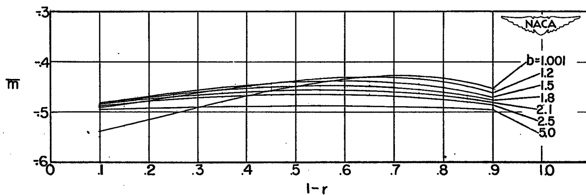
(b) \bar{m} for F-functions.
