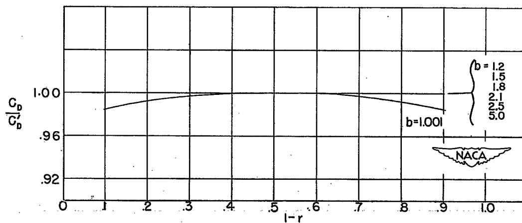
(b) C_D/C_D' for F-functions.
