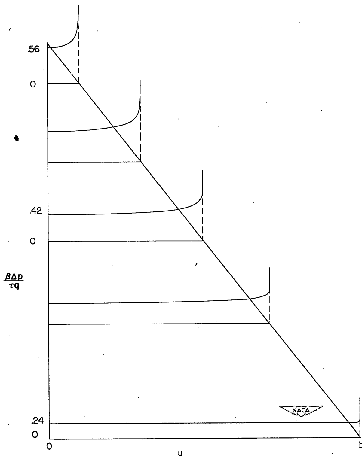
(a) Subsonic leading edge; b = 0.2 , r = 0.5 , and \bar{m} = -\frac{1}{2} .
