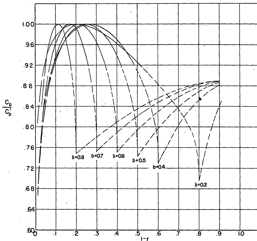
(a) C_D/C_D' for G- and H-functions.
