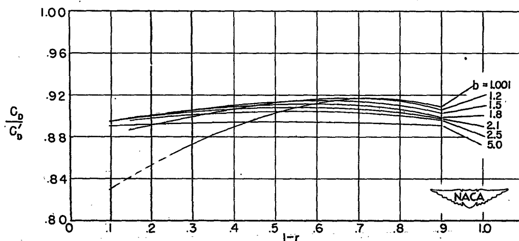
(b) C_D/C_D' for F-functions.
