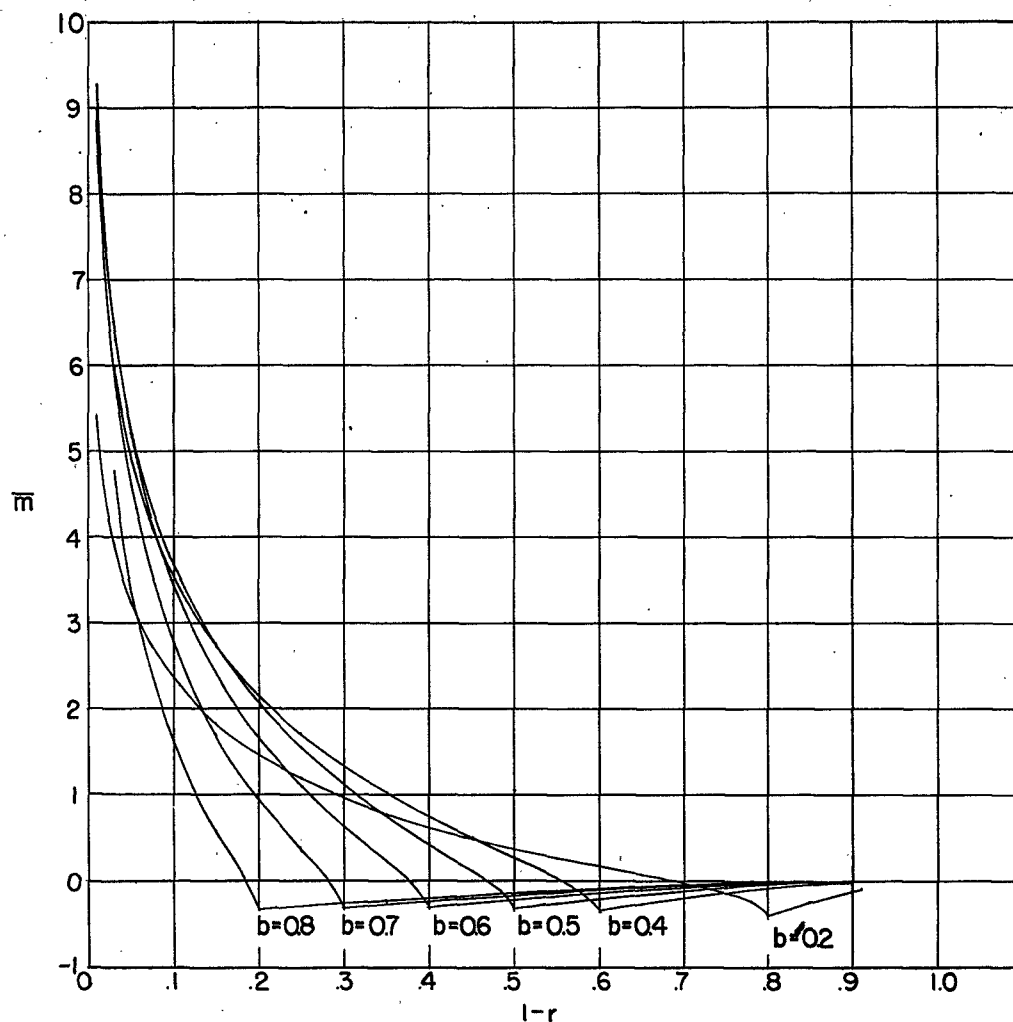
(a) \bar{m} for G- and H-functions.
