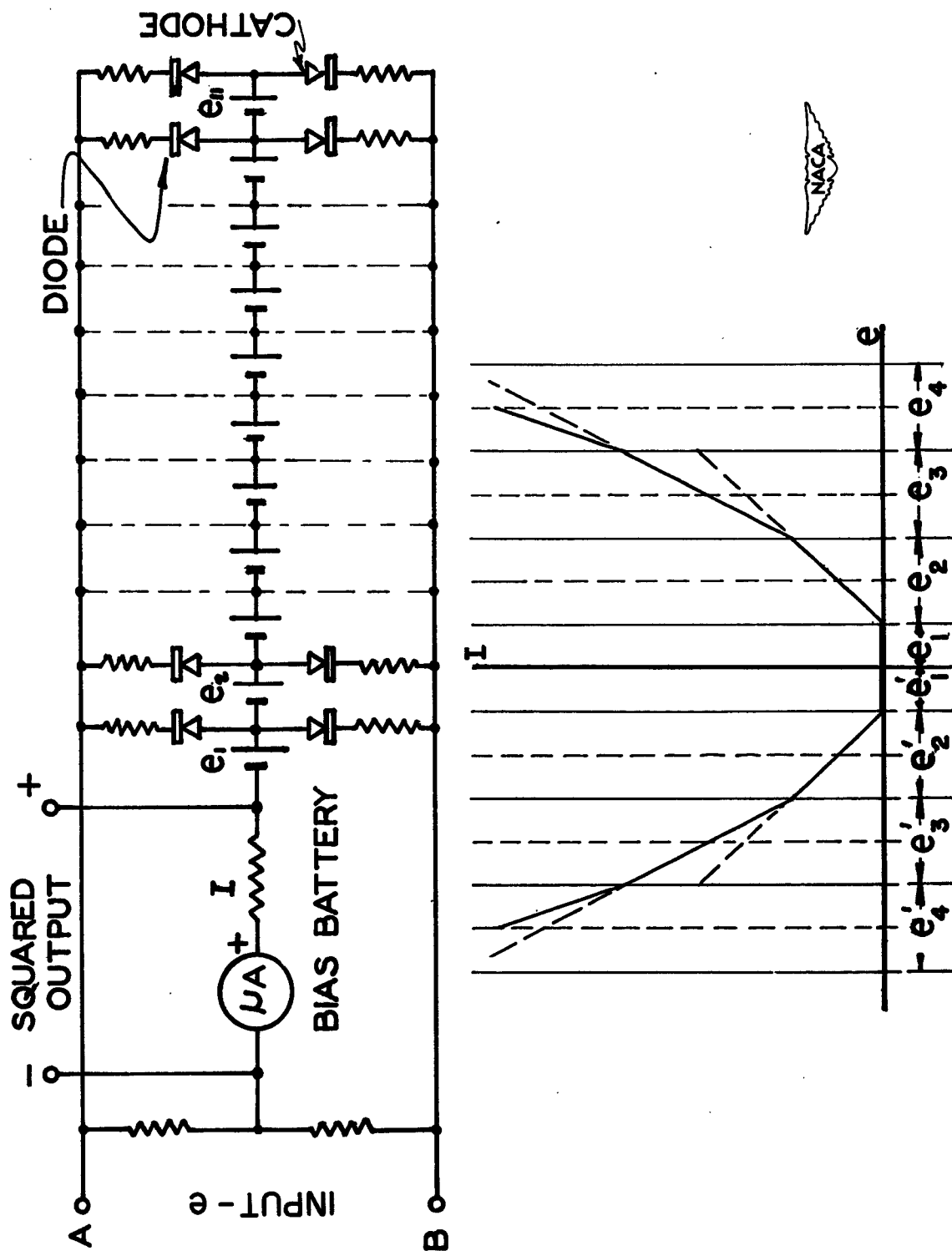
Figure 39.- Biased-diode square-law detector.
