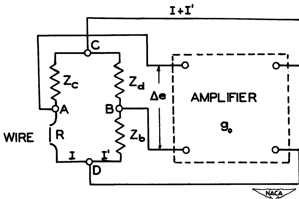
Figure 18.- Constant-temperature feedback system.
