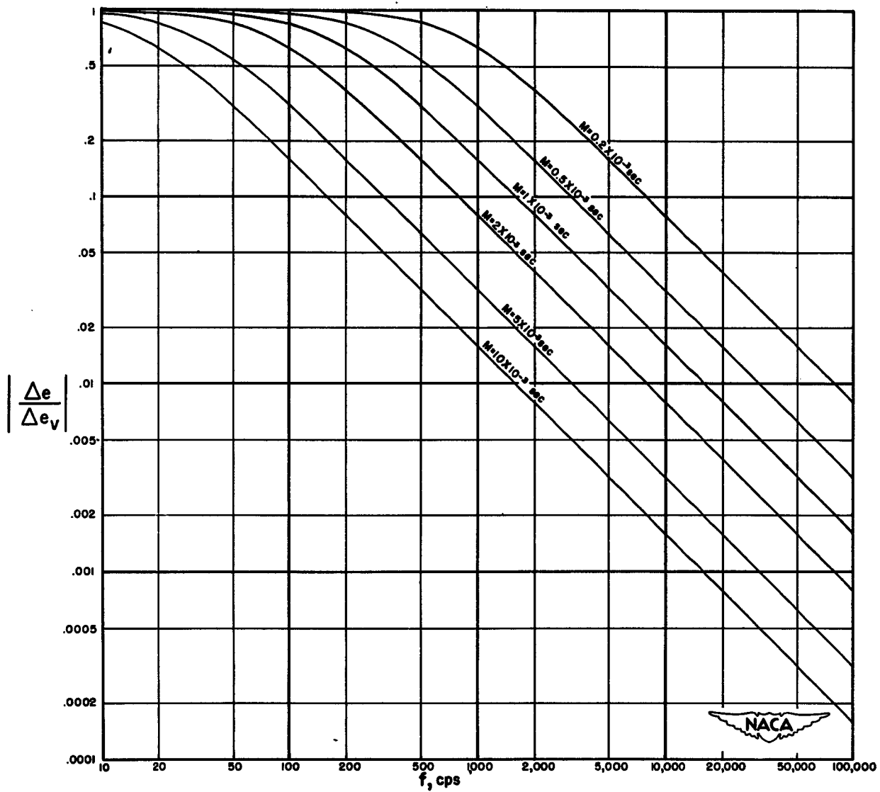
Figure 5.- Frequency response of uncompensated hot-wire.
