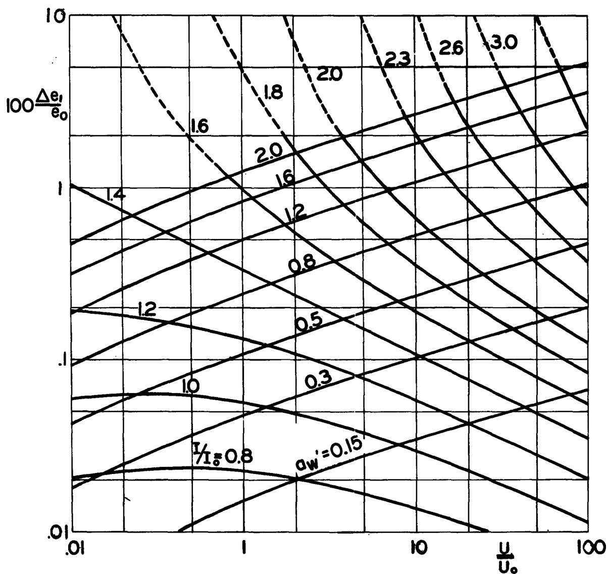
Figure 3.- Nondimensional hot-wire sensitivity in low-speed flow.
