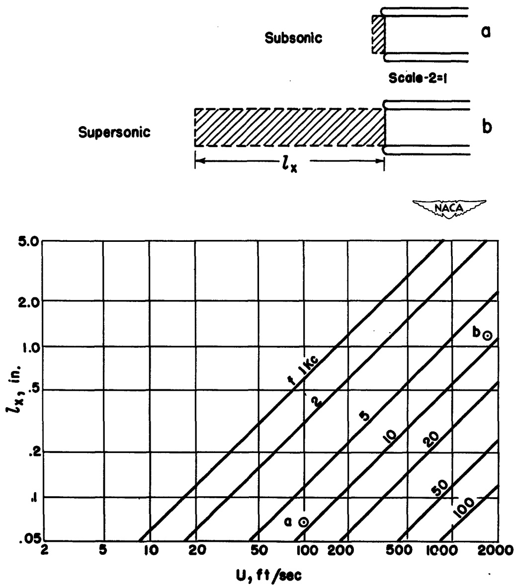
Figure 1.- Resolution length of hot-wire anemometer at various speeds.
