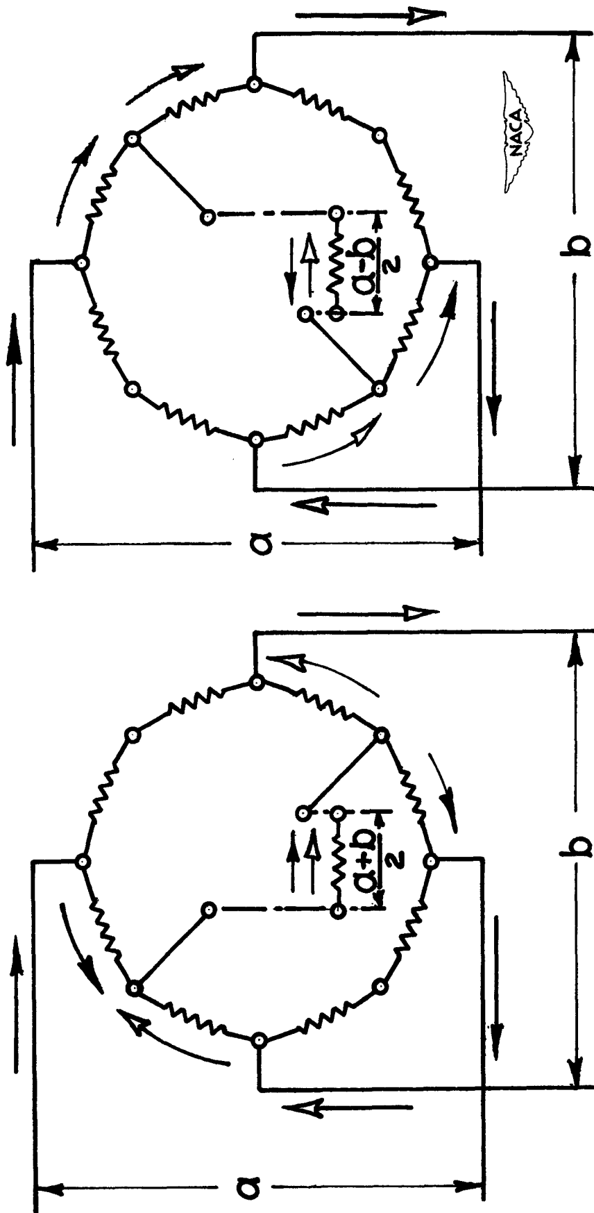
Figure 36.- Sum-difference circuit.
