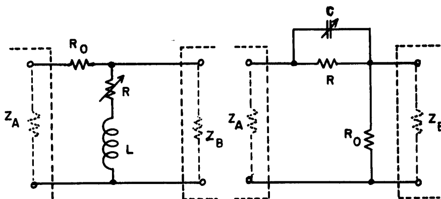
(a) Inductance resistance. (b) Capacitance resistance.
