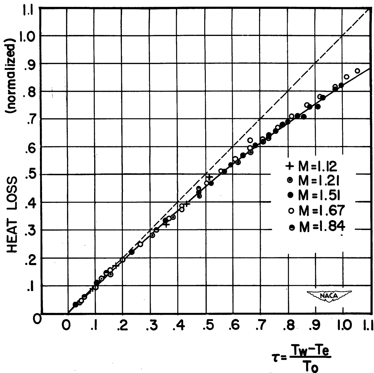
Figure 6.- Heat loss of hot-wire as function of wire temperature in supersonic flow.
