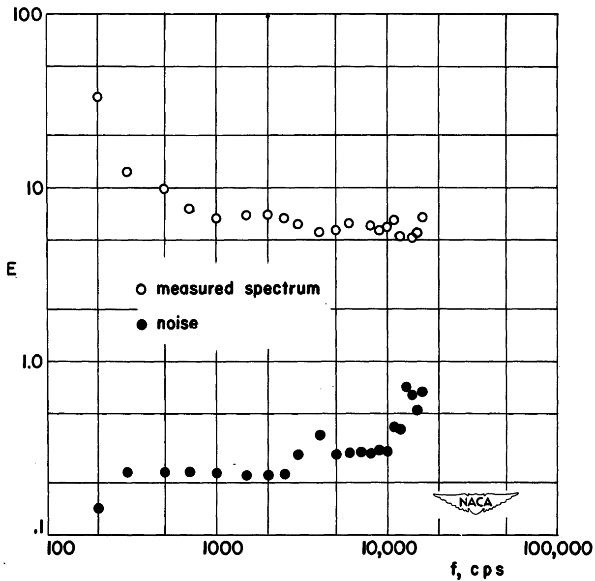
Figure 51.- Energy spectrum of fluctuations in supersonic flow.
