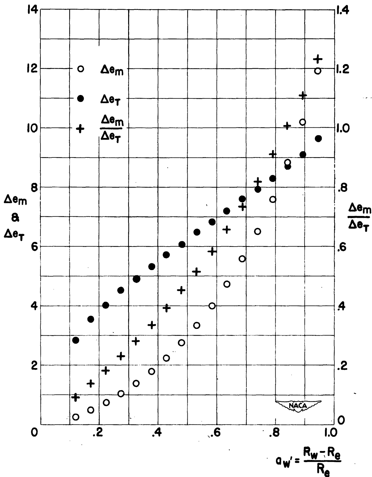
Figure 8.- Variation of fluctuation sensitivities with wire temperature in supersonic flow. Tungsten wire with 0.0015-inch diameter was used. Flow conditions: M = 1.73 , T_0 = 293^\circ \text{K} , and pressure at stagnation temperature was 40 centimeters of mercury.
