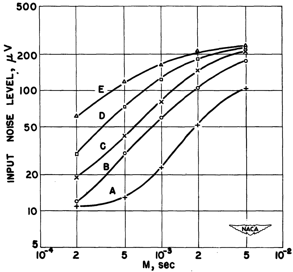
Figure 25.- Noise level of compensating amplifier.
