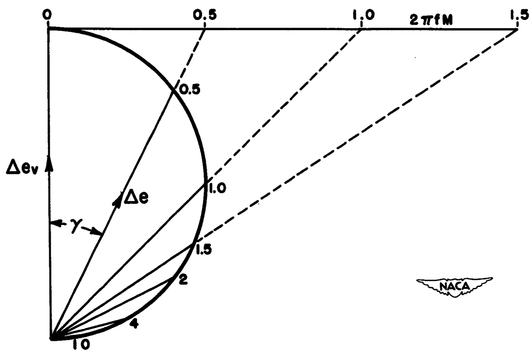
Figure 4.- Vector diagram of hot-wire thermal lag. \left| \frac{\Delta e}{\Delta e_v} \right| = \frac{1}{\sqrt{1 + (2\pi fM)^2}}; \gamma = \tan^{-1} 2\pi fM.
