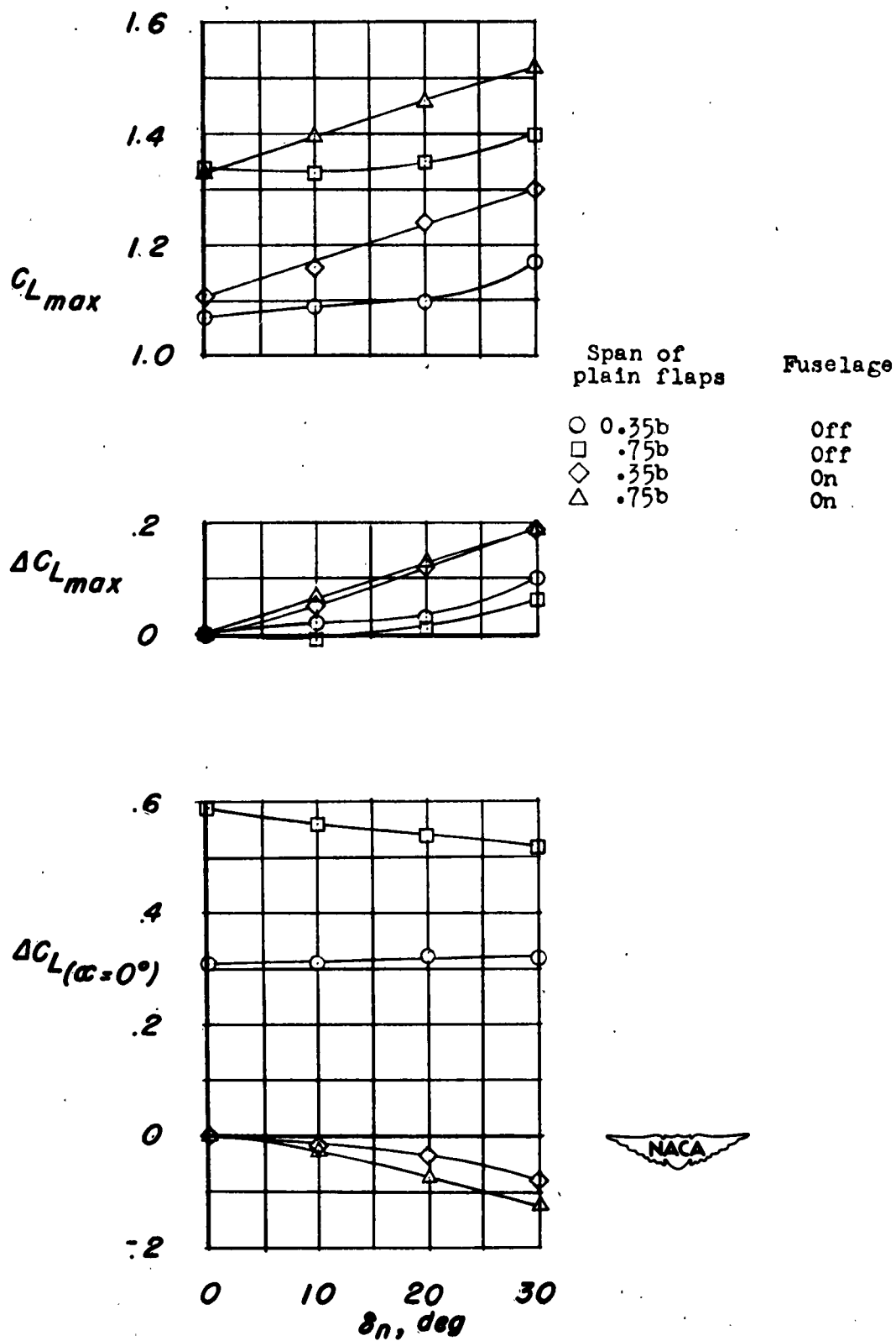
(c) Effect of drooped-nose flaps with plain flaps deflected 50^\circ .
