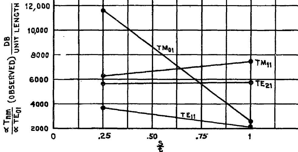
FIG 4b- \frac{\alpha T_{nm}}{\alpha TE_{01}} \text{ (OBSERVED) } \frac{\text{DB}}{\text{UNIT LENGTH}} VS \frac{s}{t} FOR SPACED RING LINE
