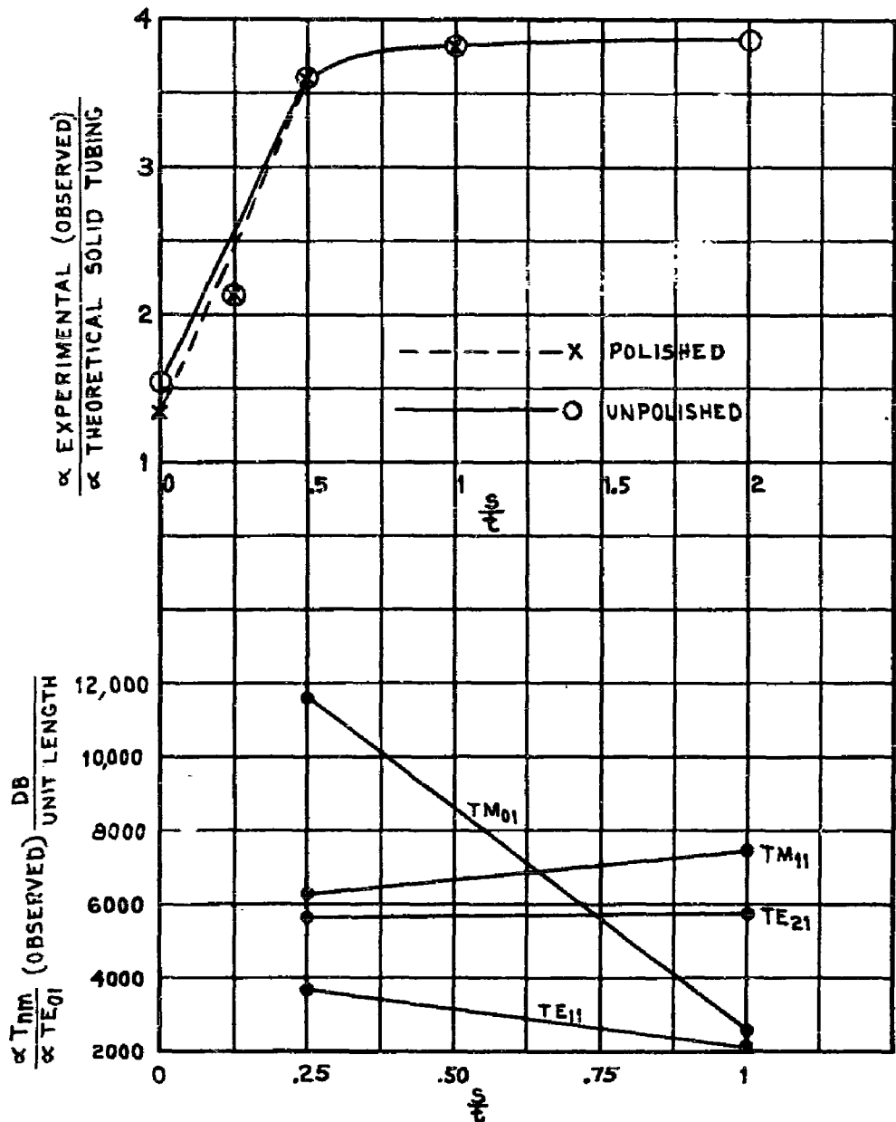
FIG 4b- \frac{\alpha T_{nm}}{\alpha TE_{01}} \text{ (OBSERVED) } \frac{\text{DB}}{\text{UNIT LENGTH}} VS \frac{s}{t} FOR SPACED RING LINE
