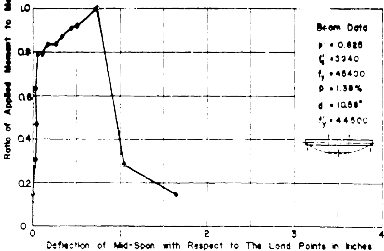
APP. FIG. 154 MOMENT RATIO VS. PURE MOMENT DEFORMATIONS FOR BEAM NQ C2W
