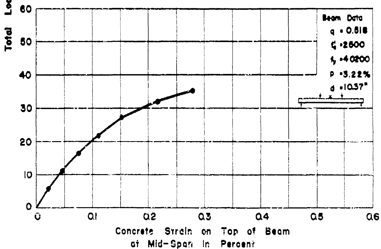
APP. FIG. 73 LOAD-STRAIN CURVES FOR BEAM NO. 15L
