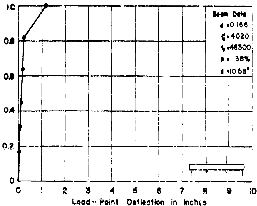
APP. FIG. III LOAD-RATIO VS. DEFLECTION FOR BEAM NO. T2Mb
