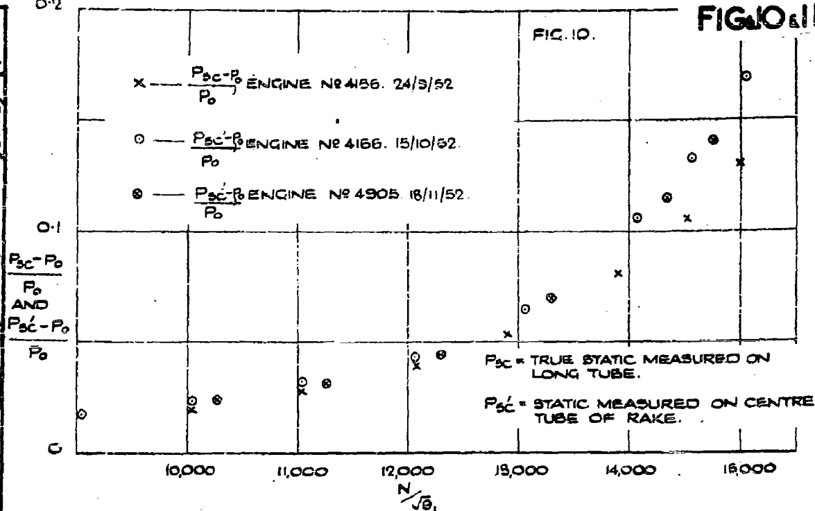
RAKE AND LONG TUBE GROUND RUN STATIC MEASUREMENTS.
