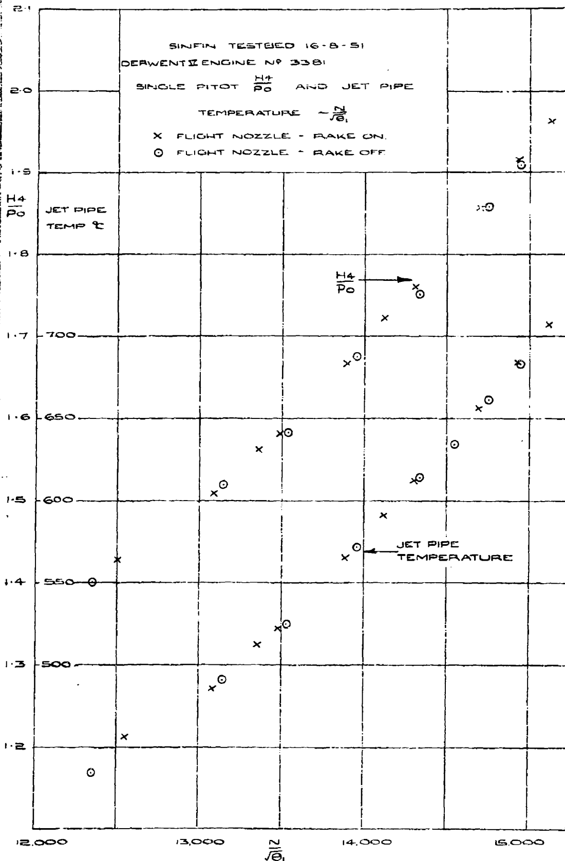
EFFECT OF PRESENCE OF PITOT RAKE ON JET PIPE TEMPERATURE & SINGLE PITOT. TEST BED RESULTS.
