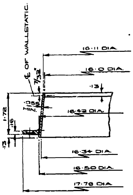
SCRAP SECTION - FINAL NOZZLE
