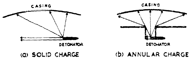
DIAGRAM SHOWING DIRECTIONS NORMAL TO DETONATION WAVE
