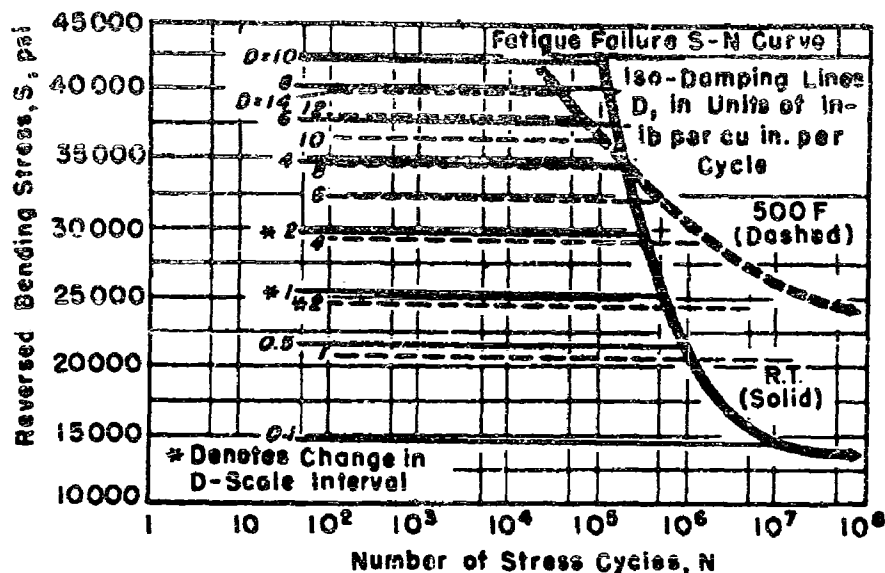
FIG. 18.—S-N-D Diagram Relating Stress, Number of Cycles, and Iso-Damping Contour Lines for TP-1-3 (Material H A ) at Room Temperature and 500 F.
