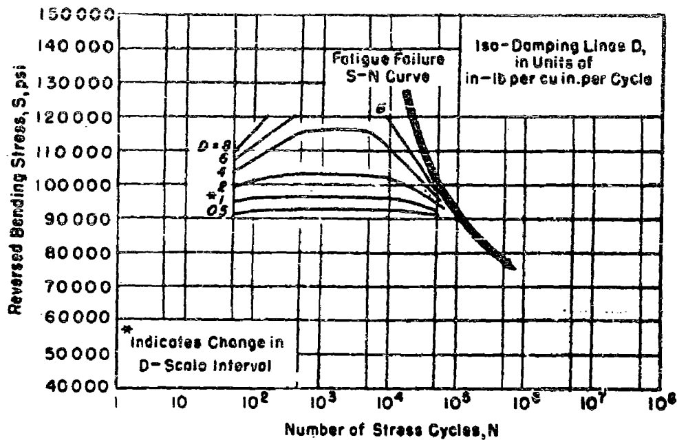
FIG. 20.—S-N-D Diagram Relating Stress, Number of Cycles, and Iso-Damping Contour Lines for Inconel X (Material E) at Room Temperature Obtained Using Type Y Specimens (Test Length 3\frac{1}{2} in., Average Diameter 0.428 in.).
