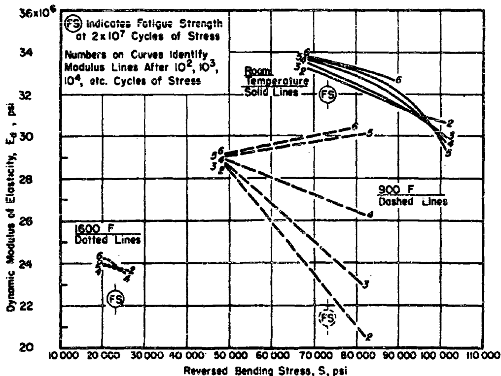
FIG. 8.— E_d - S - N Diagram Showing the Effect of Several Numbers of Sustained Reverse Stress Cycles on the Relationship Between Dynamic Modulus of Elasticity and Stress Magnitude for S-816 Alloy (Material D) at Room Temperature, 900 F, and 1600 F.
