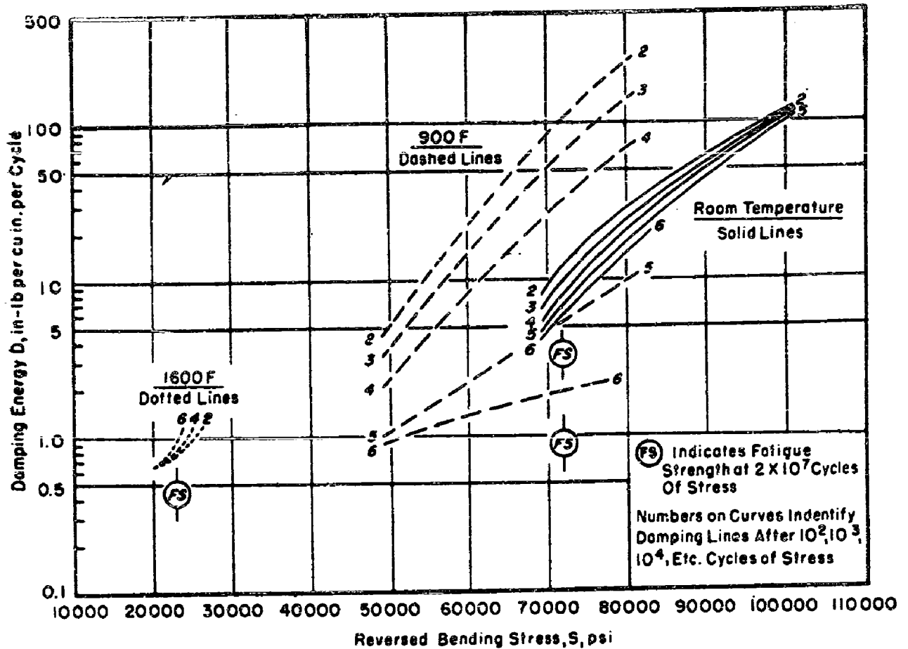
FIG. 5.— D-S-N Diagram Showing the Effects of Several Numbers of Sustained Reversed Stress Cycles on the Relationship Between Damping Energy and Stress Magnitude for S-816 Alloy (Material D) at Room Temperature, 900 F, and 1600 F.
