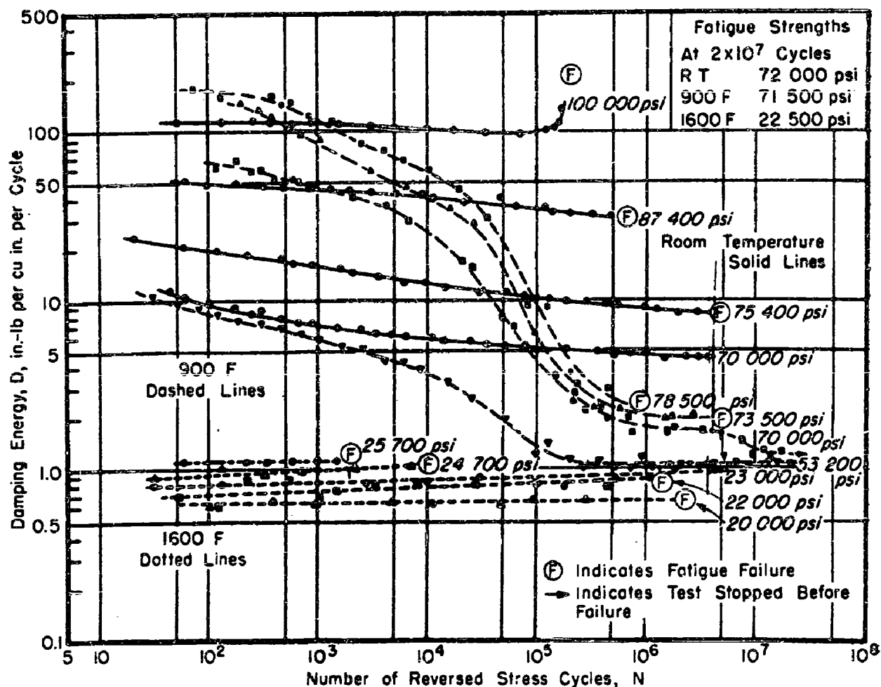
FIG. 4.— D - N - S Diagram Showing the Effects of Several Magnitudes of Sustained Reversed Stress on the Relationship Between Damping Energy and Number of Cycles for S-816 Alloy (Material D) at Room Temperature, 900 F, and 1600 F.
