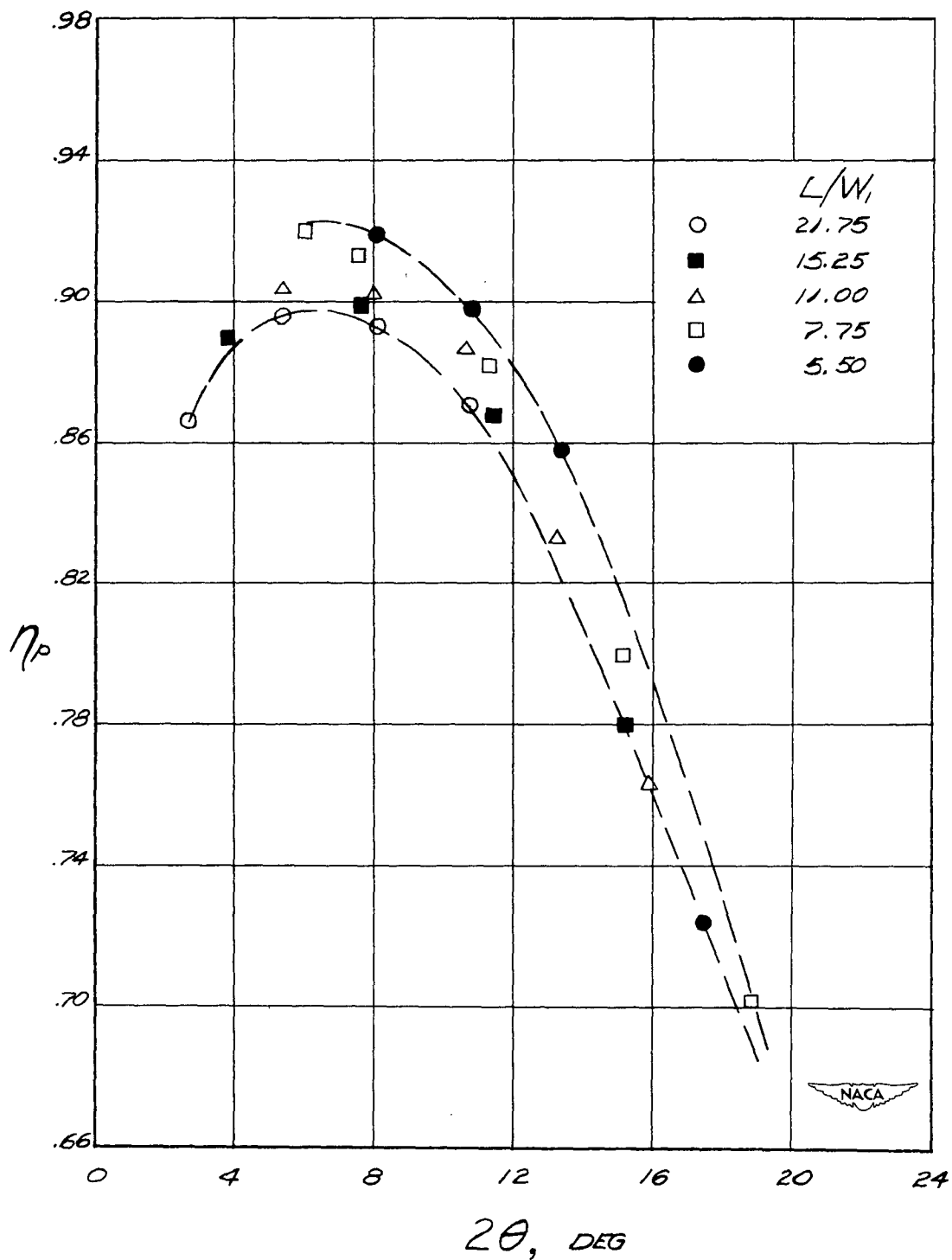
Figure 15.- Variation of pressure efficiency with divergence angle.
