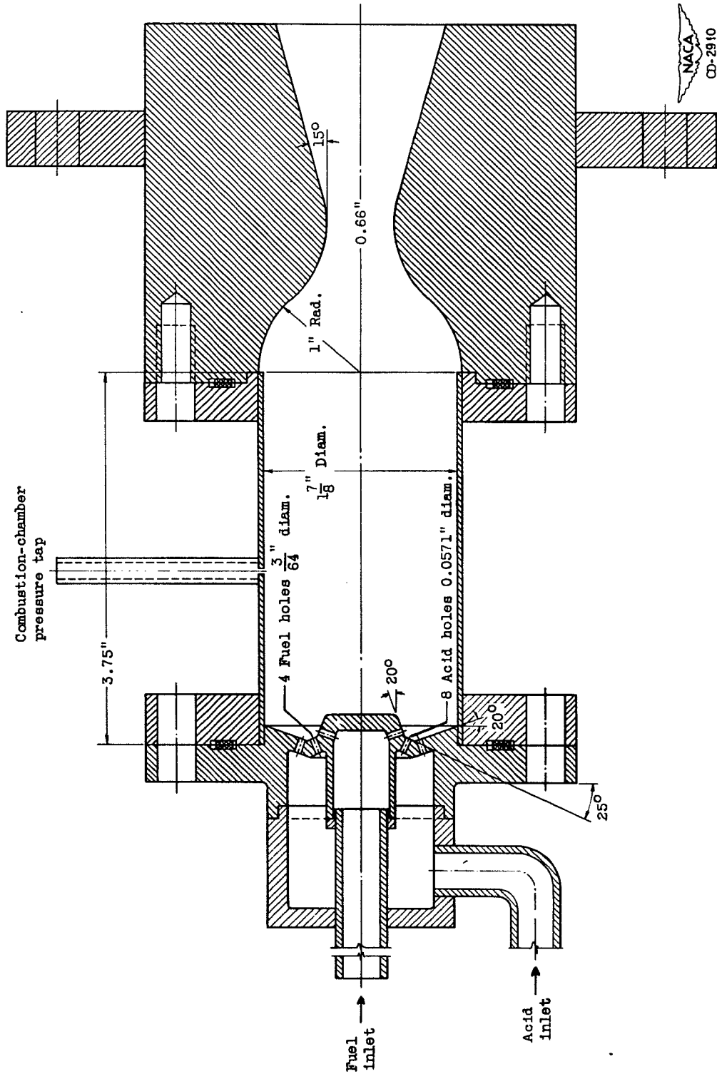
Figure 1. - Rocket motor assembly showing combustion chamber and injector. Nominal thrust, 200 pounds; characteristic length, approximately 30 inches.
