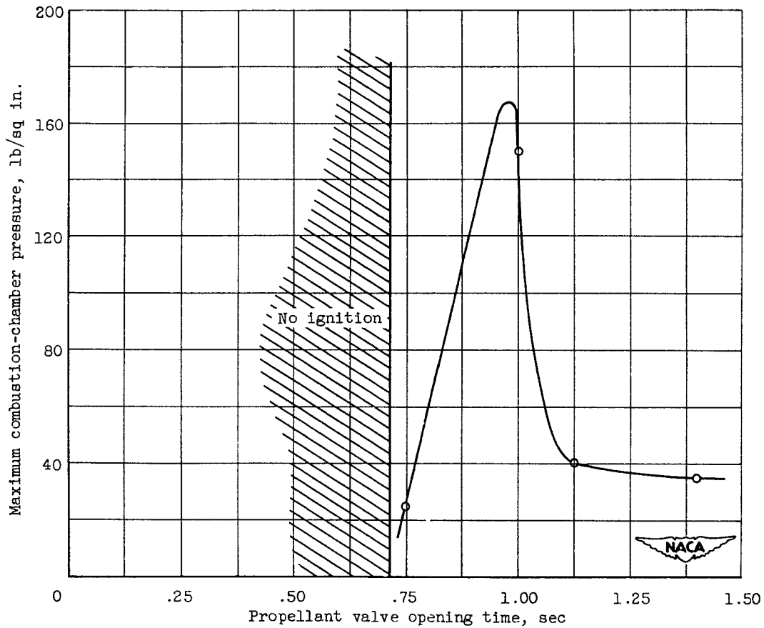
Figure 8. - Effect of propellant valve opening time on maximum combustion-chamber pressure recorded during combustion of 15 cubic inches of 70 percent triethylamine, 30 percent orthotoluidine igniter fuel with RFNA 1. Temperature, -65^{\circ} F.
