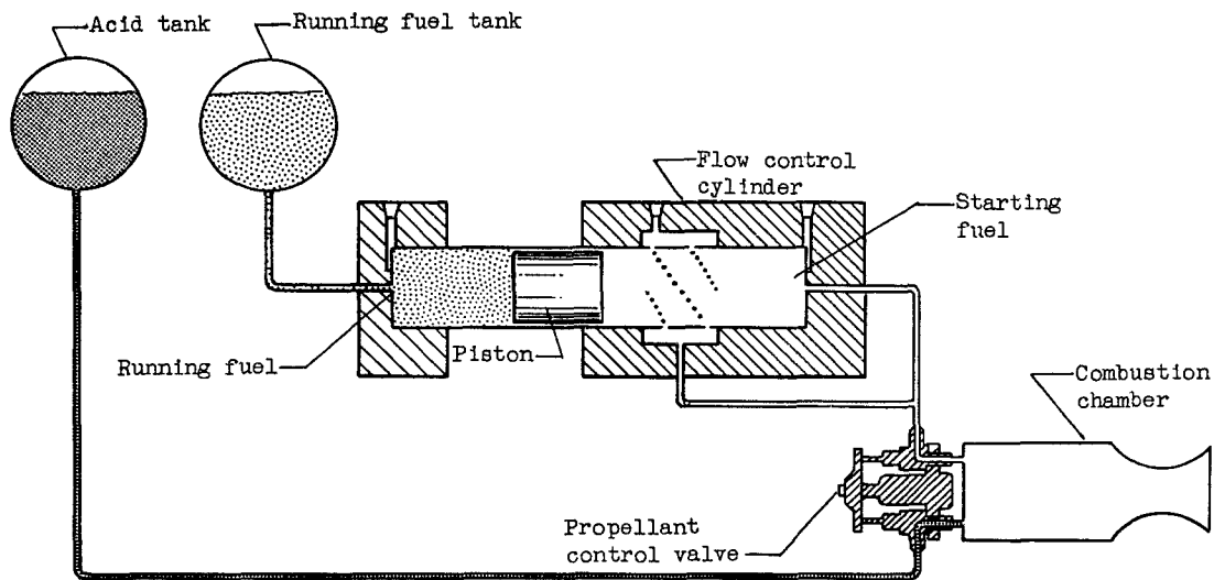
(a) Rocket motor propellant system.
