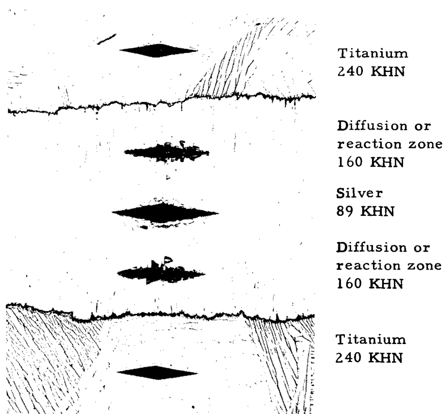
FIGURE 6. PHOTOMICROGRAPH OF A JOINT BETWEEN TITANIUM BRAZED WITH SILVER
