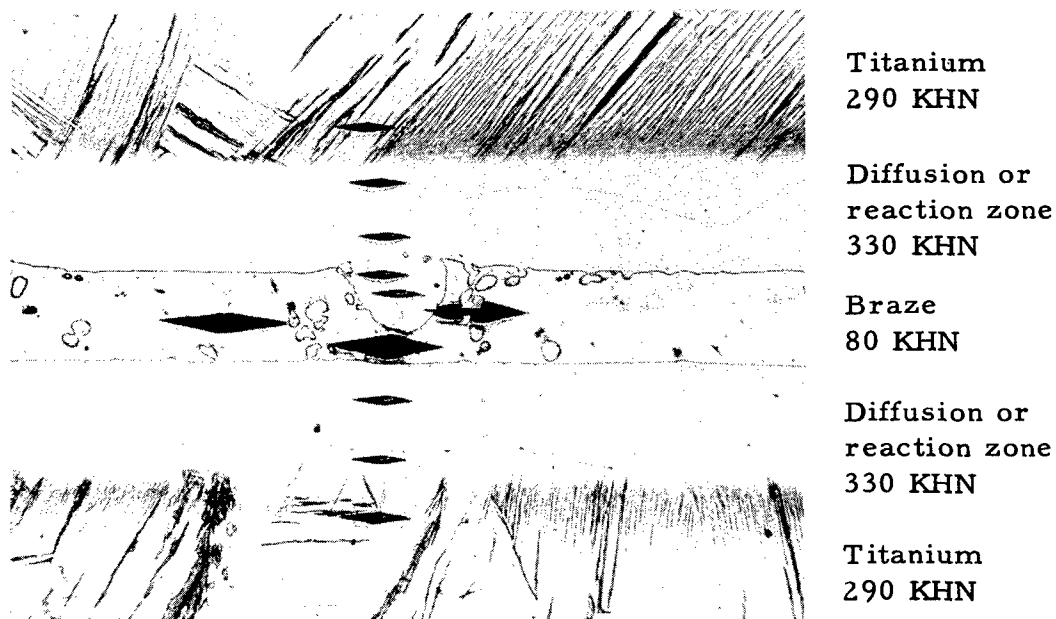
FIGURE 4. PHOTOMICROGRAPH OF JOINT BETWEEN TITANIUM BRAZED WITH AN ALLOY OF 85 PER CENT SILVER AND 15 PER CENT MANGANESE SHOWING KNOOP HARDNESS READINGS WITH A 25-GRAM LOAD
