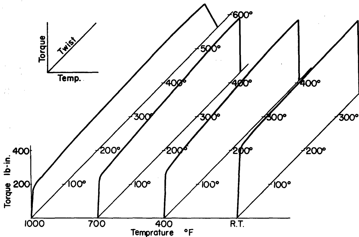
Fig.72 Torque - Twist Curves for Fourth Speed Torsion Tests of RC-130-B Titanium Alloy at Four Temperatures.
