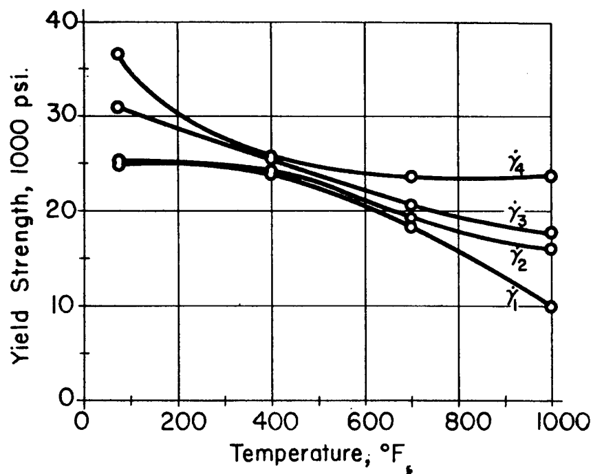
Fig. 16 Effect of Temperature on the Shearing Yield Strength of SAE 1018 Steel in Torsion.
