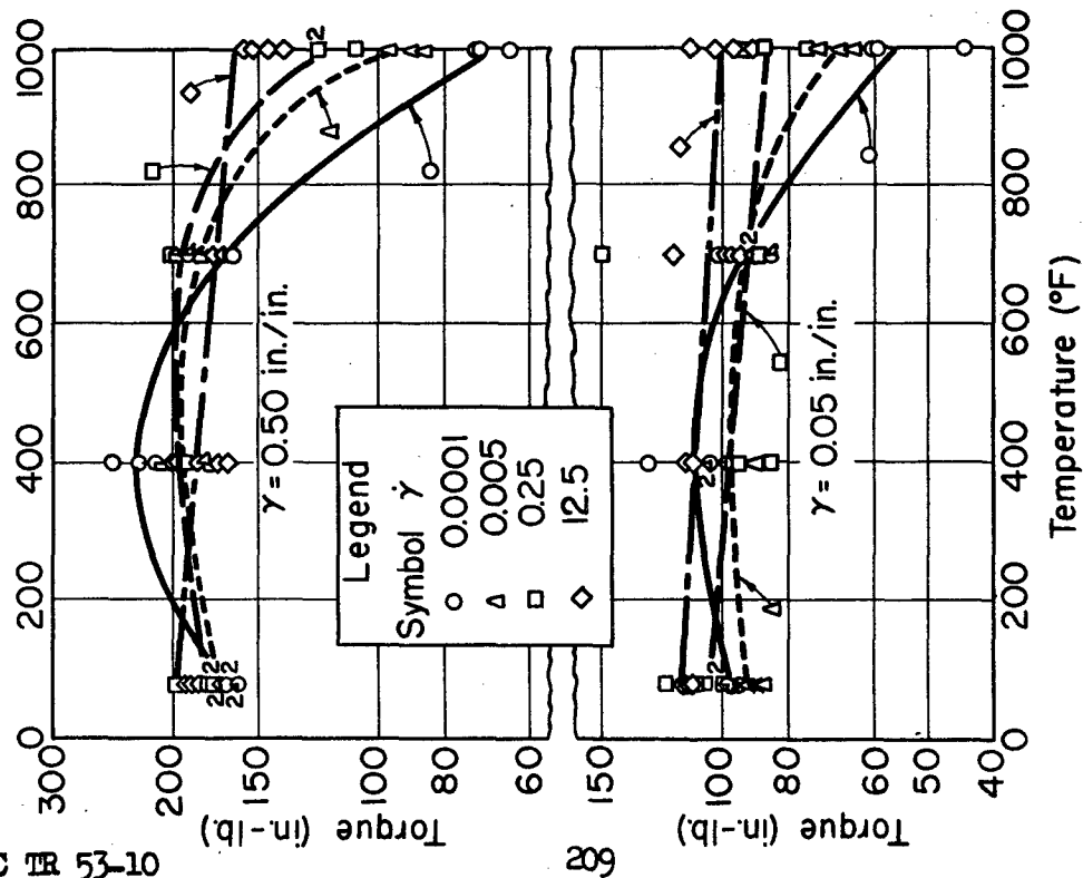
Fig.85 Effect of Temperature on the Torque at Constant Shearing Strain in Torsion Tests of SAE 1018 Steel.
