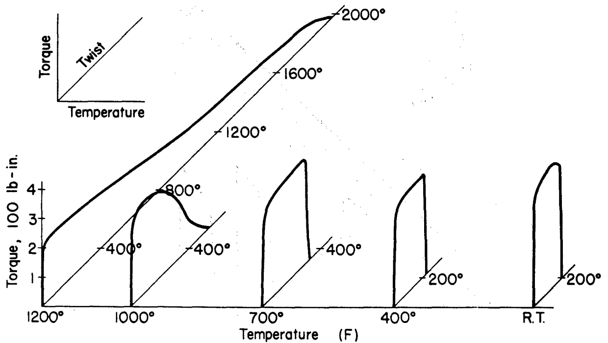
Fig.67 Torque - Twist Curves for Fourth Speed Torsion Tests of SAE 4340 Steel at Five Temperatures.
