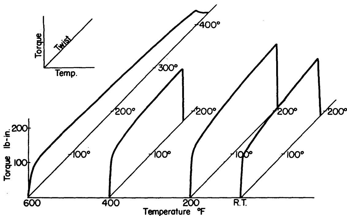
Fig.68 Torque-Twist Curves for Fourth Speed Torsion Tests of 24S-T Aluminum Alloy at Four Temperatures.
