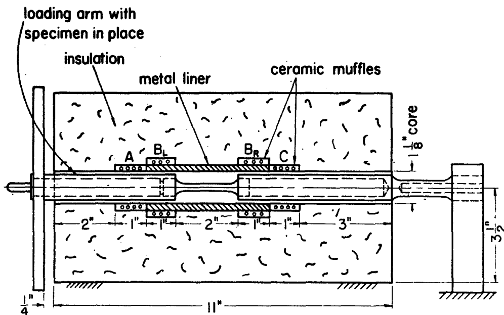
Fig.8 Sectional View of the Electric Furnace for Elevated Temperature Torsion Tests.
