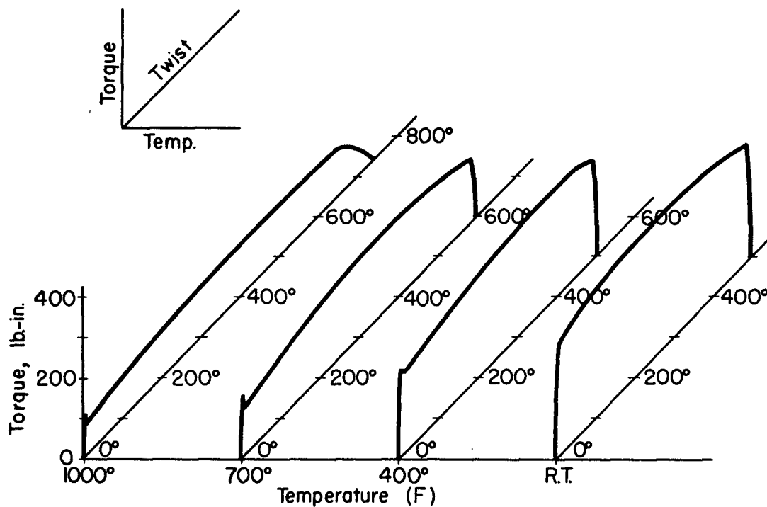
Fig.71 Torque-Twist Curves for Fourth Speed Torsion Tests of RC-70 Titanium at Four Temperatures.
