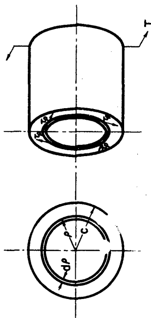
Fig.99 Shearing Stresses in Torsion of a Round Bar
