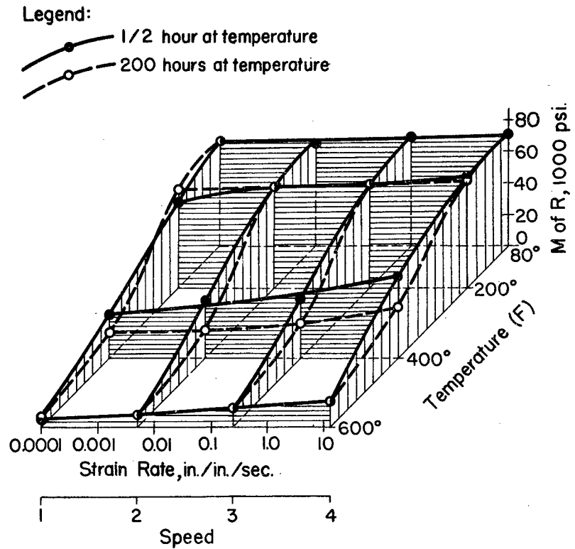
Fig.37 Combined Effects of Rate of Strain and Temperature on the Modulus of Rupture of 75S-T Aluminum Alloy in Torsion.
