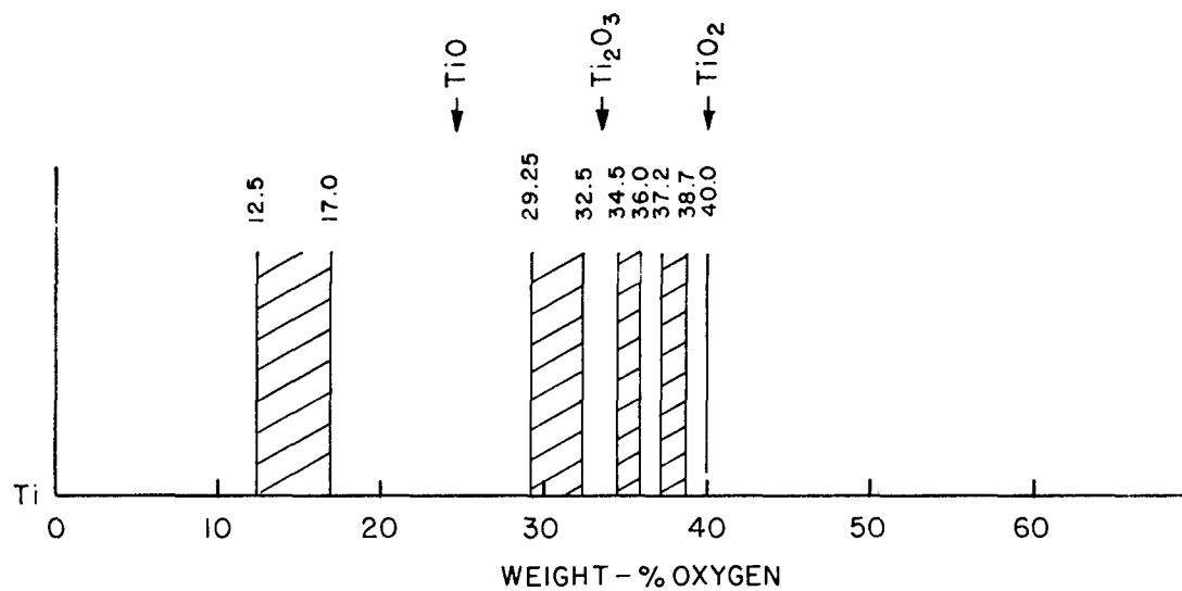
Fig. 61 - phases and Phase Ranges in the System Titanium-Oxygen (Ehrlich)
