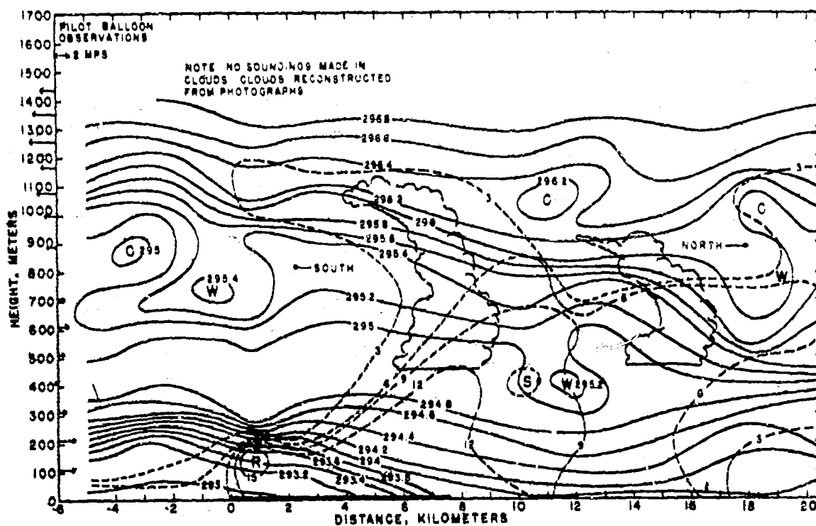
FIG. 20. Approximately north-south cross section constructed from the airplane soundings 1315-1435 EST, August 14, 1950 (Case 4) showing isopleths of potential temperature and turbulence index. The notation and units are the same as for the previous cross sections. C stands for potentially cool air and W for potentially warm. R stands for relatively rough air, S for relatively smooth. The clouds are not drawn in to scale, nor are they located exactly, but merely sketched to indicate the shape and vertical extent of the larger ones.
