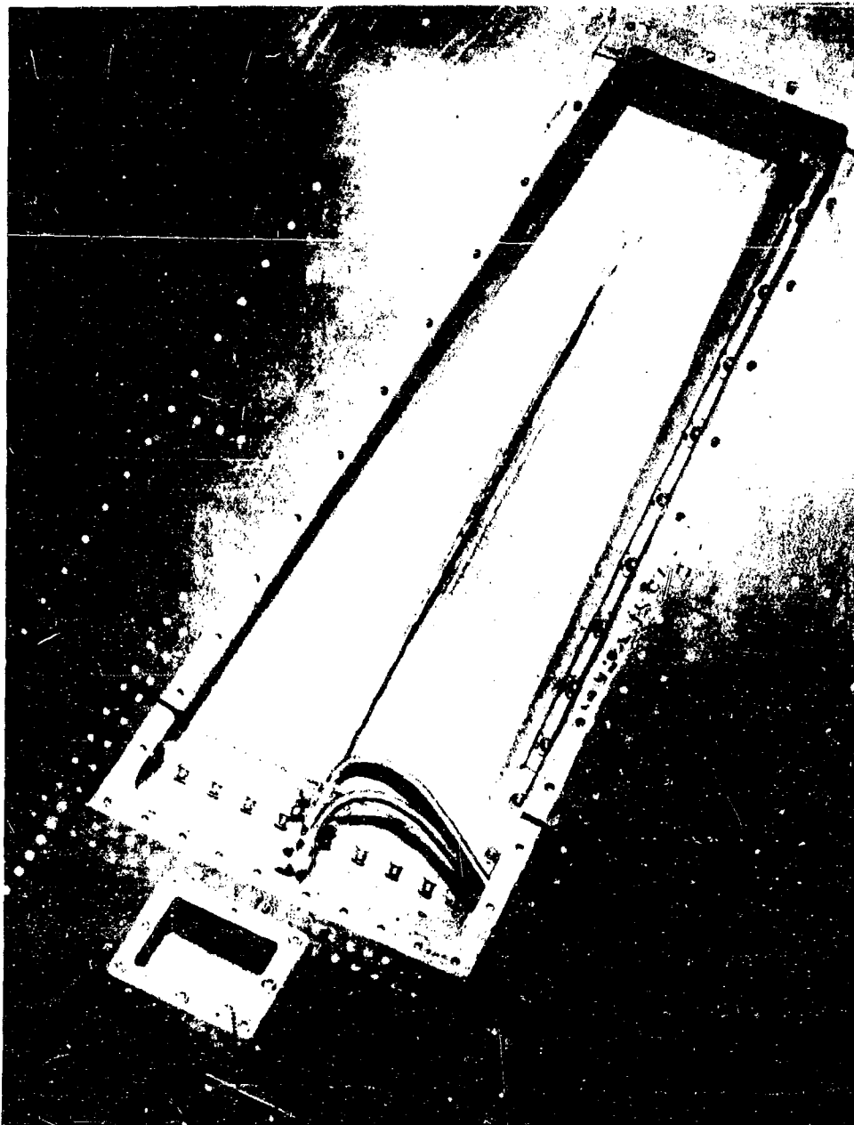
INSTALLATION OF ANTENNA CAVITY AND ONE ANTENNA PANEL FOR EXPERIMENTAL PURPOSES IN F-86 AIRCRAFT Fig. 16
