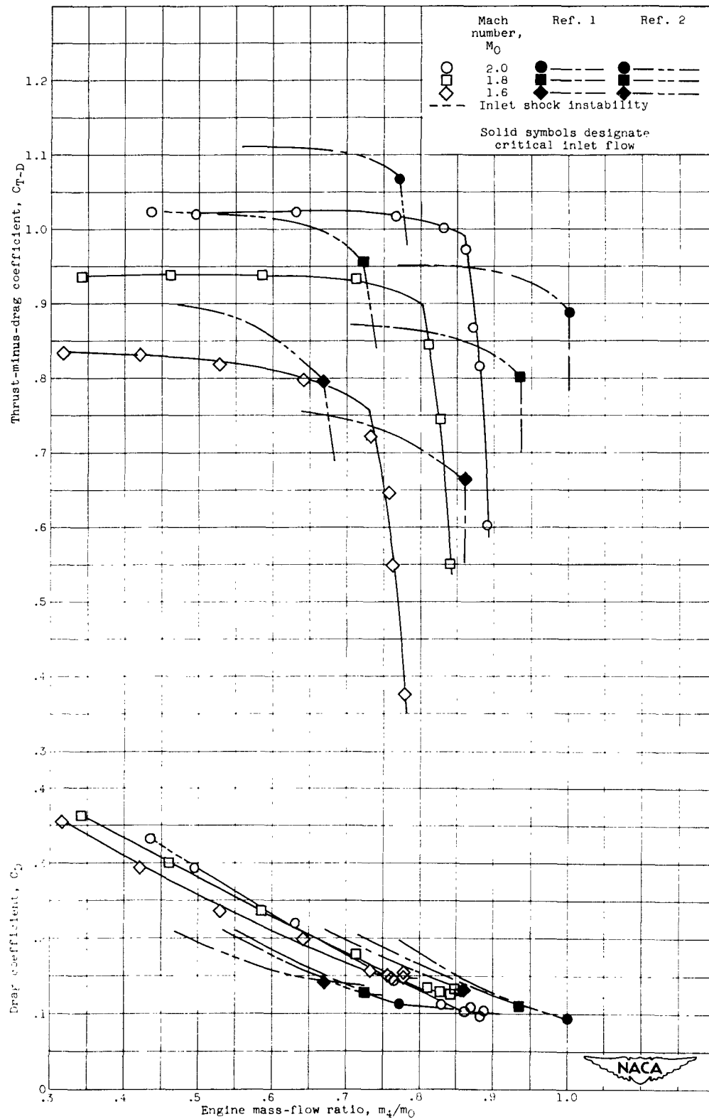
Figure 9. - Concluded. Variation of inlet characteristics and force coefficients with mass-flow ratio at zero nominal angle of attack for range of Mach numbers. Model with bypass on bottom.
