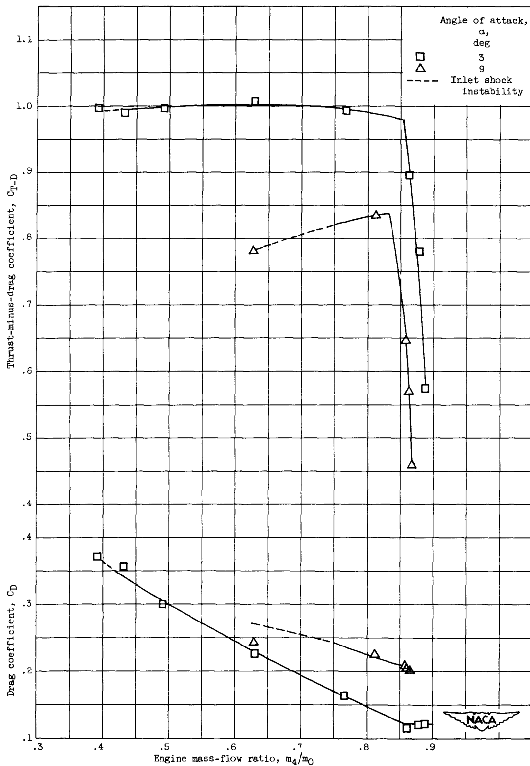
Figure 11. - Concluded. Variation of inlet characteristics and force coefficients with mass-flow ratio at nominal angles of attack of 3^\circ and 9^\circ for Mach number of 2.0. Model with bypass on bottom.
