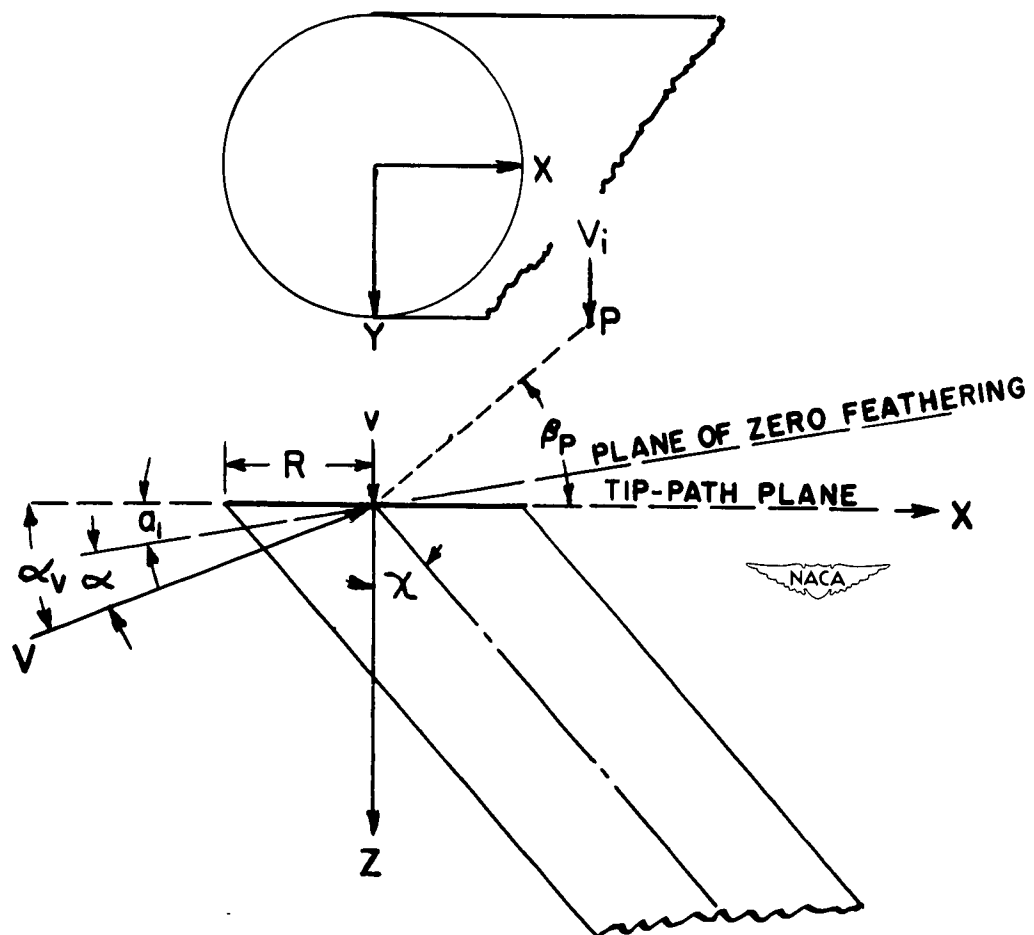
Figure 2.- Geometry of wake.
