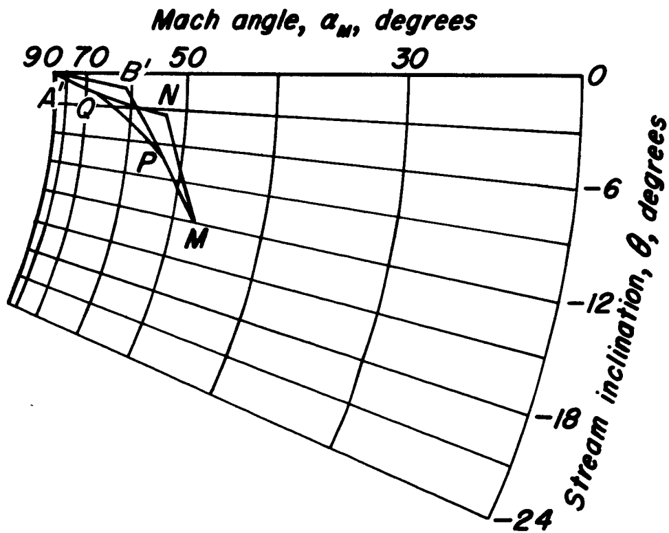
(b) Hodograph plane.
