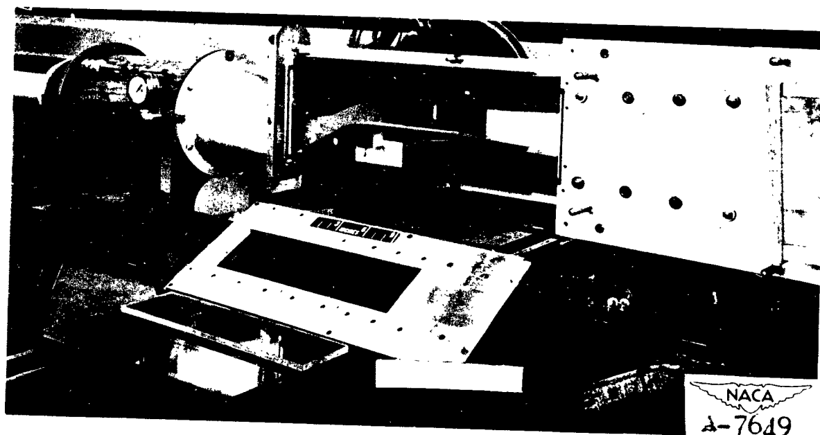
(b) Model nozzle with side plates and windows removed. Figure 8.— The 1-1/2-by 1-1/2-inch asymmetric adjustable nozzle.
