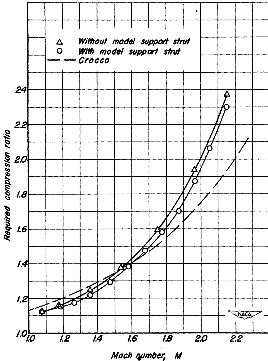
Figure 11.— Compression ratio required for 1\frac{1}{2} \times 1\frac{1}{2} -inch asymmetric adjustable nozzle (atmospheric exit).
