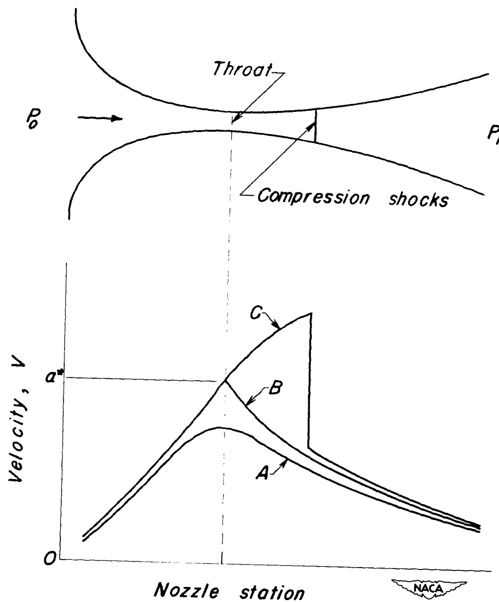
Figure 1. - Compressible flow through a convergent-divergent nozzle.
