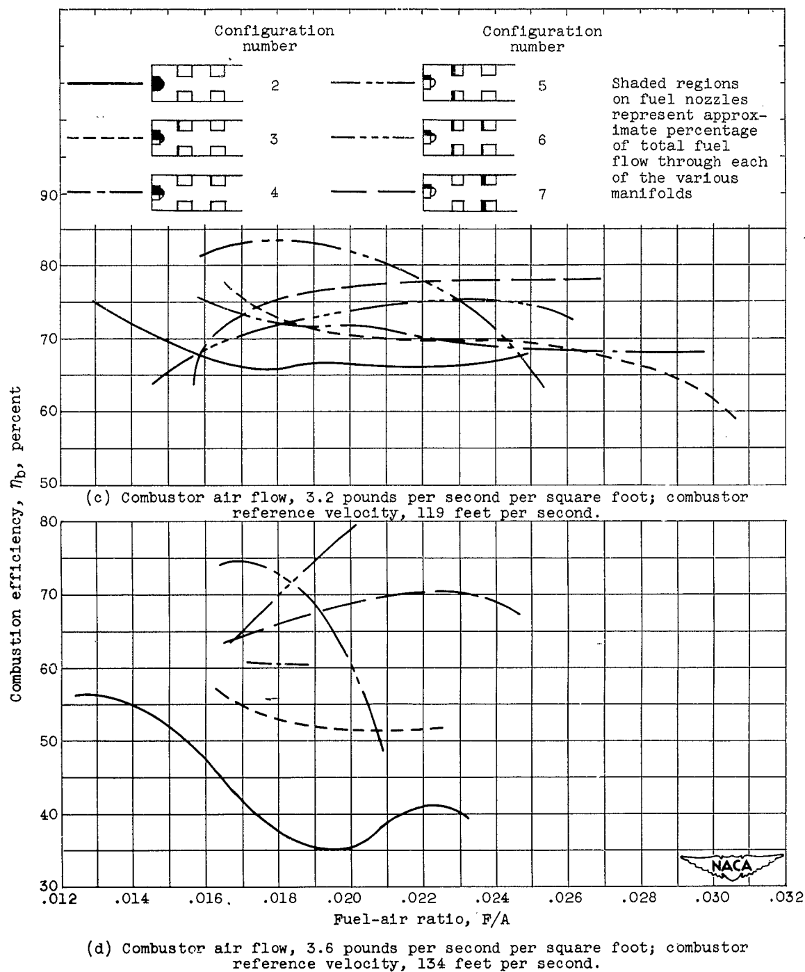
Figure 8. - Concluded. Variation of combustion efficiency with fuel loading for various fuel-injection configurations. Combustor-inlet pressure, 15 inches mercury absolute; inlet temperature, 80° F. All configurations are represented for 3.0-gallon fuel nozzles in number one manifold (see fig. 5).
