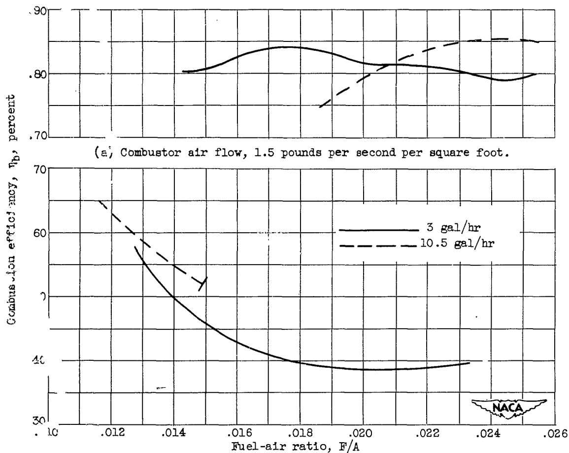
Figure 7. - Variation of combustion efficiency with fuel-air ratio for two fuel-injection nozzle sizes. Combustor-inlet pressure, 15 inches of mercury absolute; inlet temperature, 80° F.
