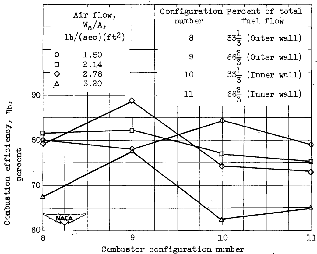
Figure 9. - Variation in combustion efficiency for unsymmetrical fuel introduction for various air flows. Combustor-inlet pressure, 15 inches mercury absolute; inlet temperature, 540° R.
