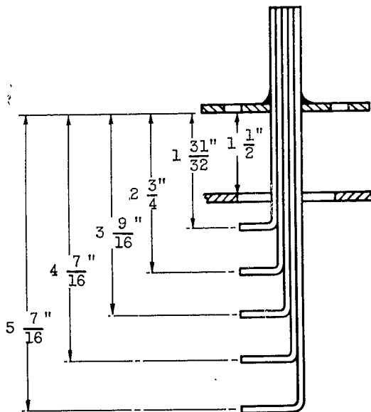
(a) Outlet total-pressure rake.
