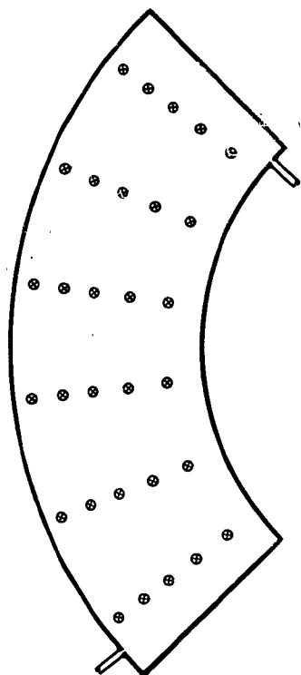
(b) Outlet thermocouples (chromel-alumel) in plane at station 2.
