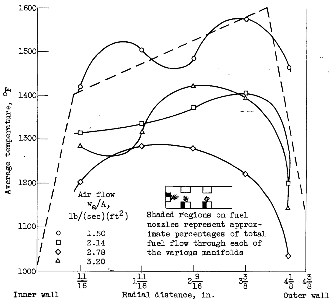
Figure 10. - Concluded. Radial temperature distribution of exhaust gas for various air flows. Fuel-air ratio, 0.0235 to 0.0275 (average of 4 rakes). Dashed curve represents approximate desired profile.
