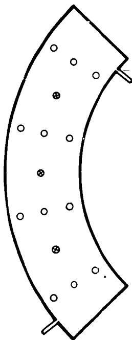
(c) Inlet thermocouples (iron-constantan) and inlet total-pressure rakes in plane at station 1.
