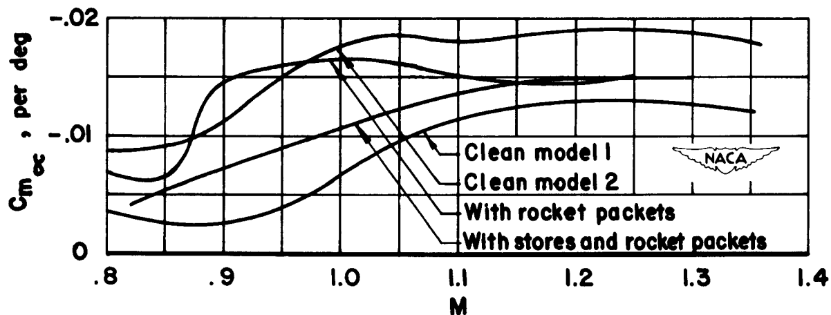
Figure 19.- Longitudinal stability. Center of gravity of clean model 2 located at 0.099\bar{c} ; center of gravity of other three models at about 0.17\bar{c} (see table I).
