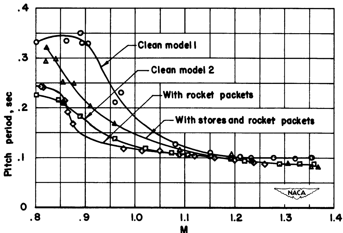
Figure 18.- Pitch period.
