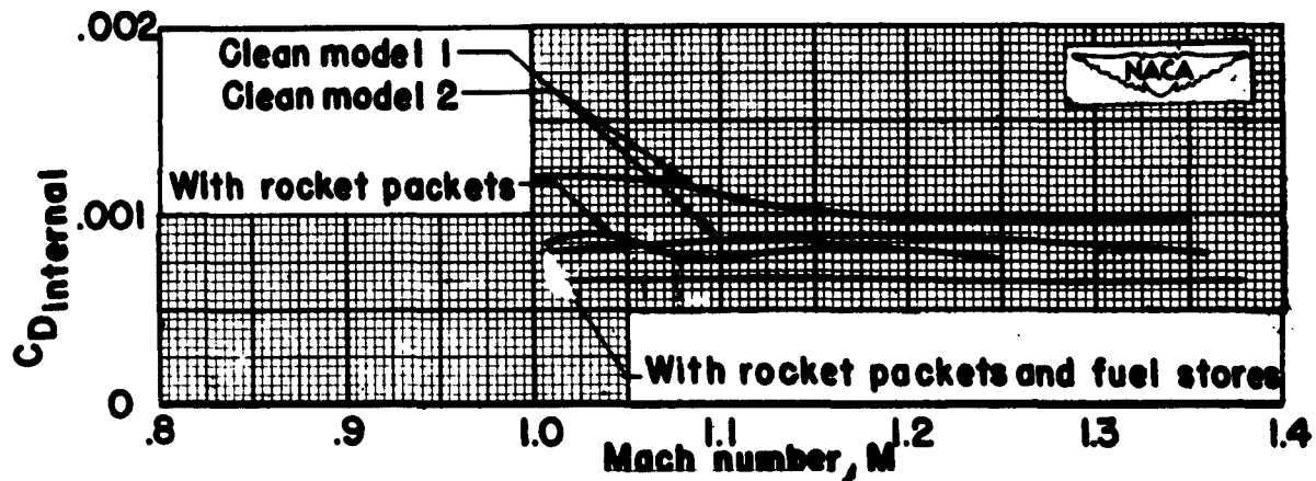
Figure 14.- Internal drag.
