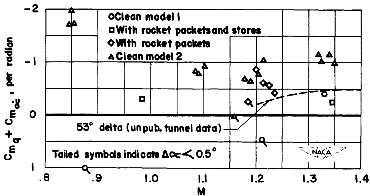
Figure 24.- Pitch-damping parameter.
