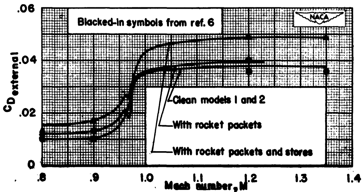
Figure 16.- External drag.
