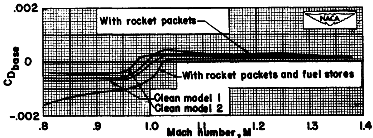
Figure 15.- Base drag (choking cup).
