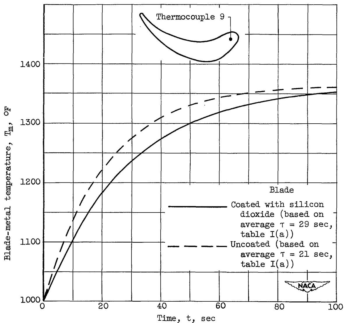
Figure 5. - Comparison of calculated stator-blade time-temperature relations for uncoated blade and blade coated with silicon dioxide. Curves calculated with experimental time constants in equation (4); blade-metal initial temperature, 1000^{\circ}\text{F} ; blade-metal final temperature, 1365^{\circ}\text{F} .
