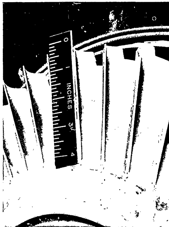
(c) Blades after 2\frac{1}{2} hours of operation.
