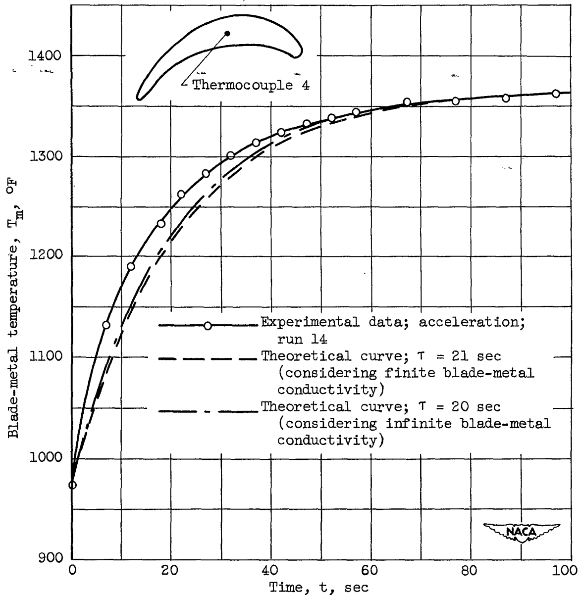
Figure 6. - Comparison of experimental and theoretical time-temperature relations at midchord, midthickness of uncoated rotor blade. Blade-metal initial temperature, 972^{\circ}\text{F} ; blade-metal final temperature, 1365^{\circ}\text{F} .
