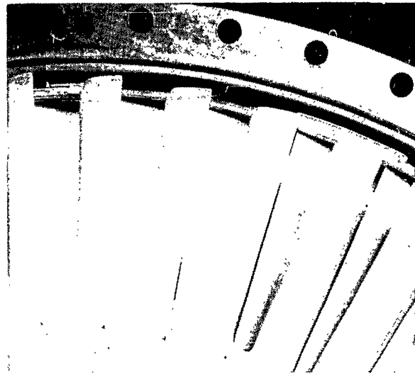
(b) Blades after 1 hour of operation.
