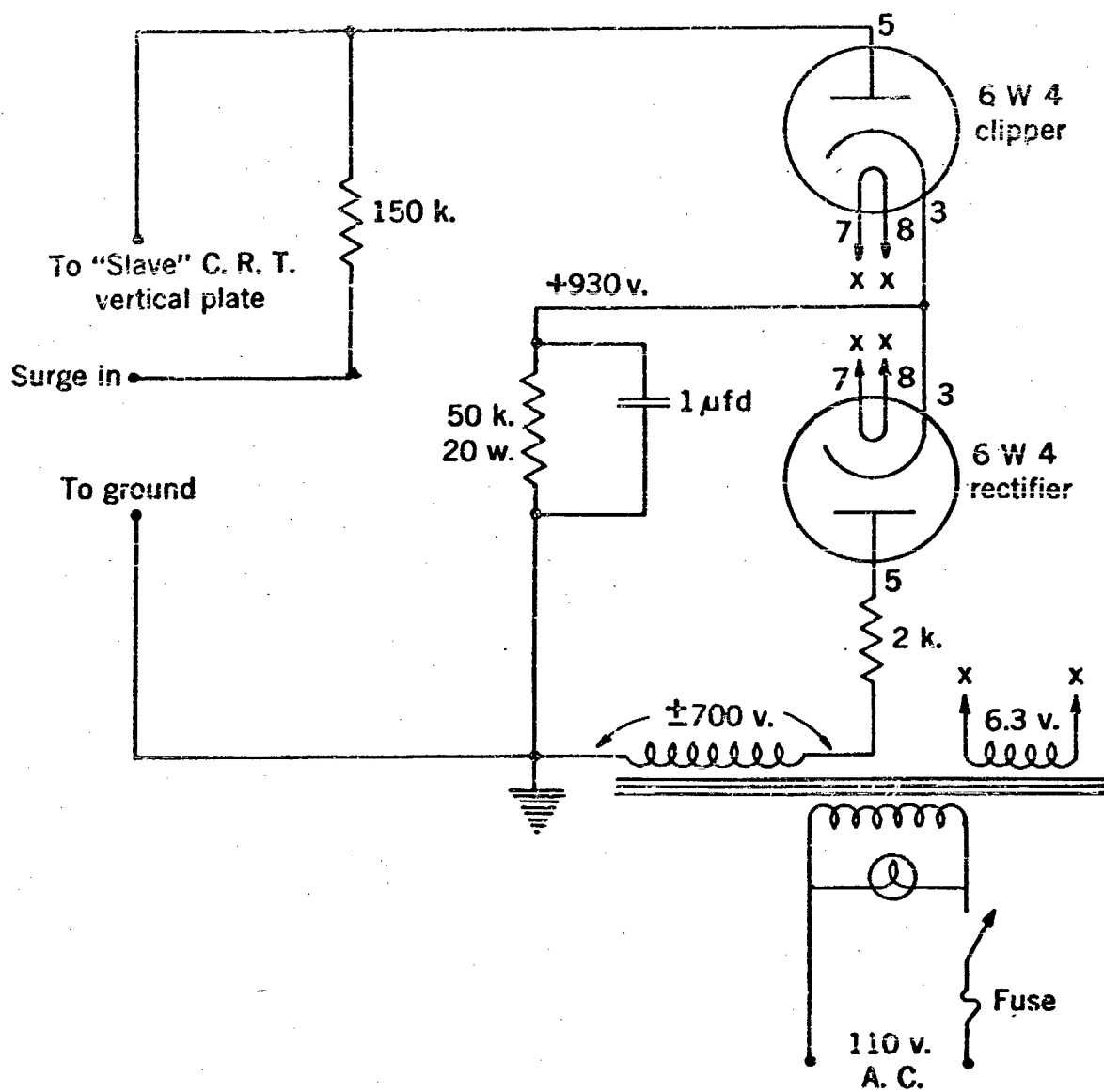
Figure 43.—Circuit diagram of the surge clipper.
