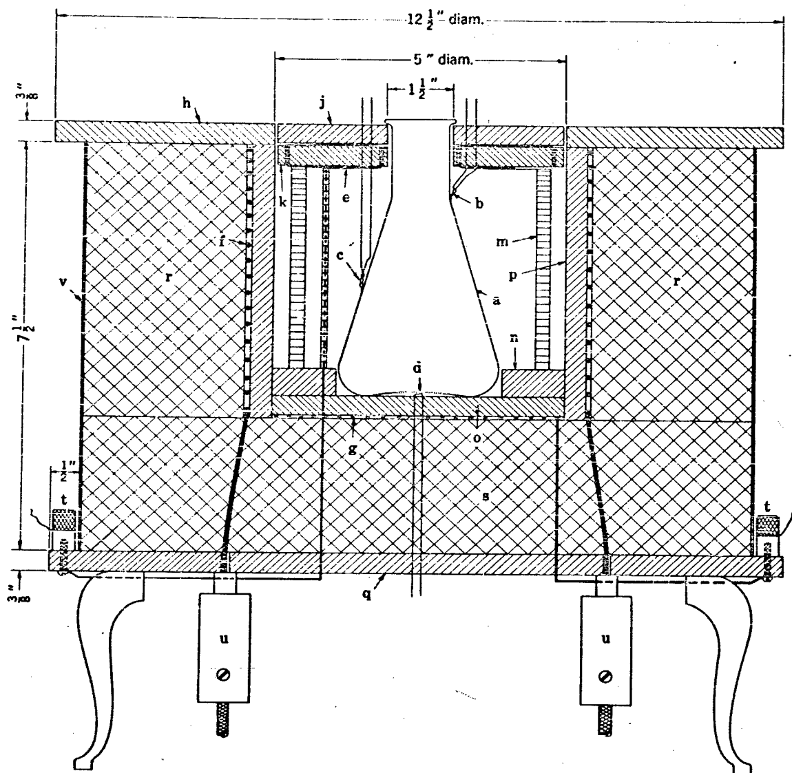
Figure 25. - Detailed drawing of the I-8 ignition temperature apparatus.
