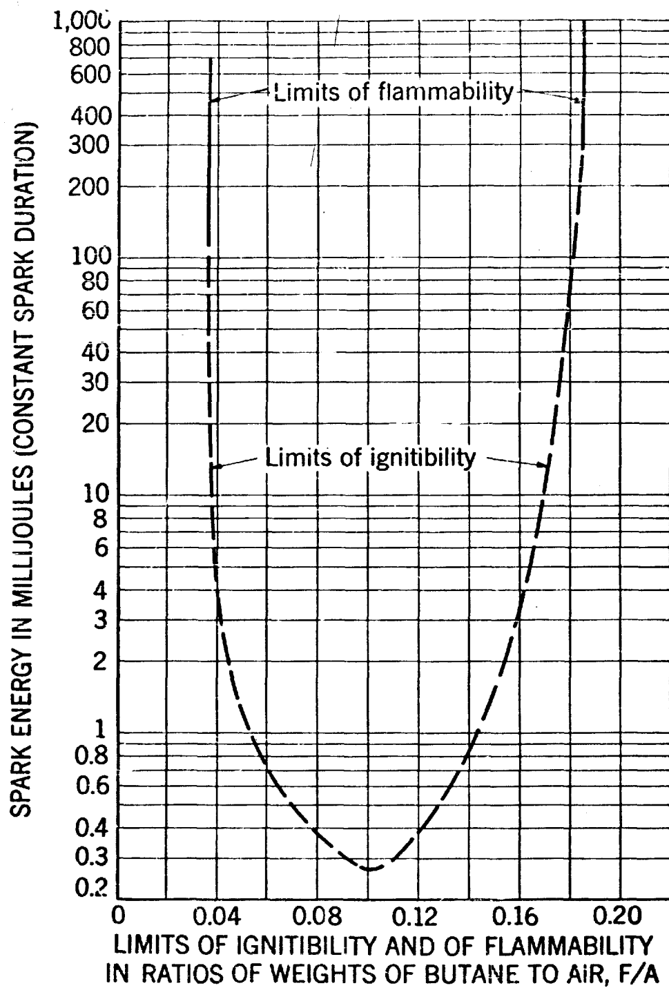
Figure 3. - Ignitability curve for butane-air mixtures at one atmosphere and 78° F.
