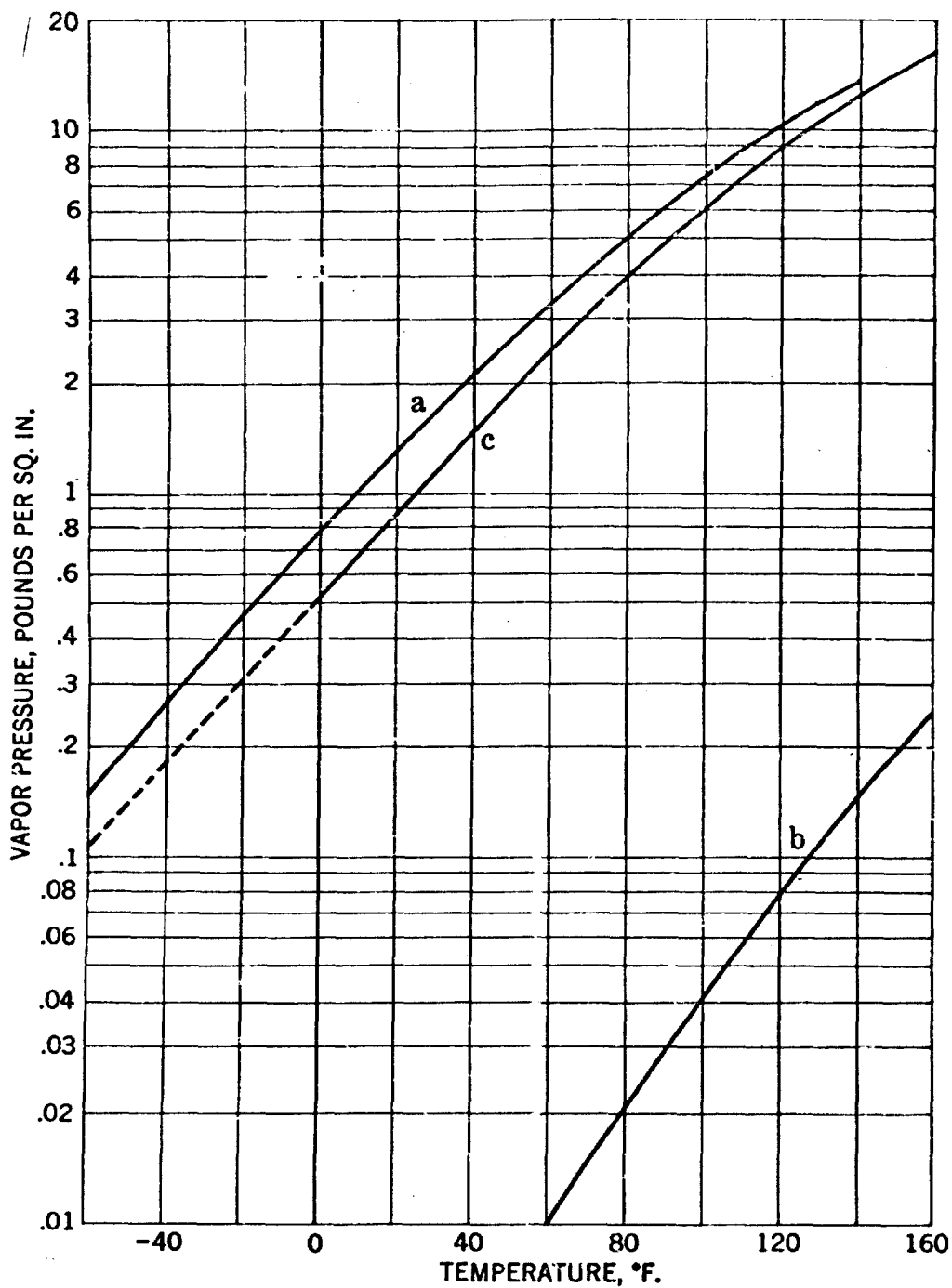
Figure 2.—Reid vapor pressure curves for (a) aviation gasoline grades 100/130 and 115/145, (b) aviation jet fuel grade JP-1 and (c) aviation jet fuel grade JP-3.
