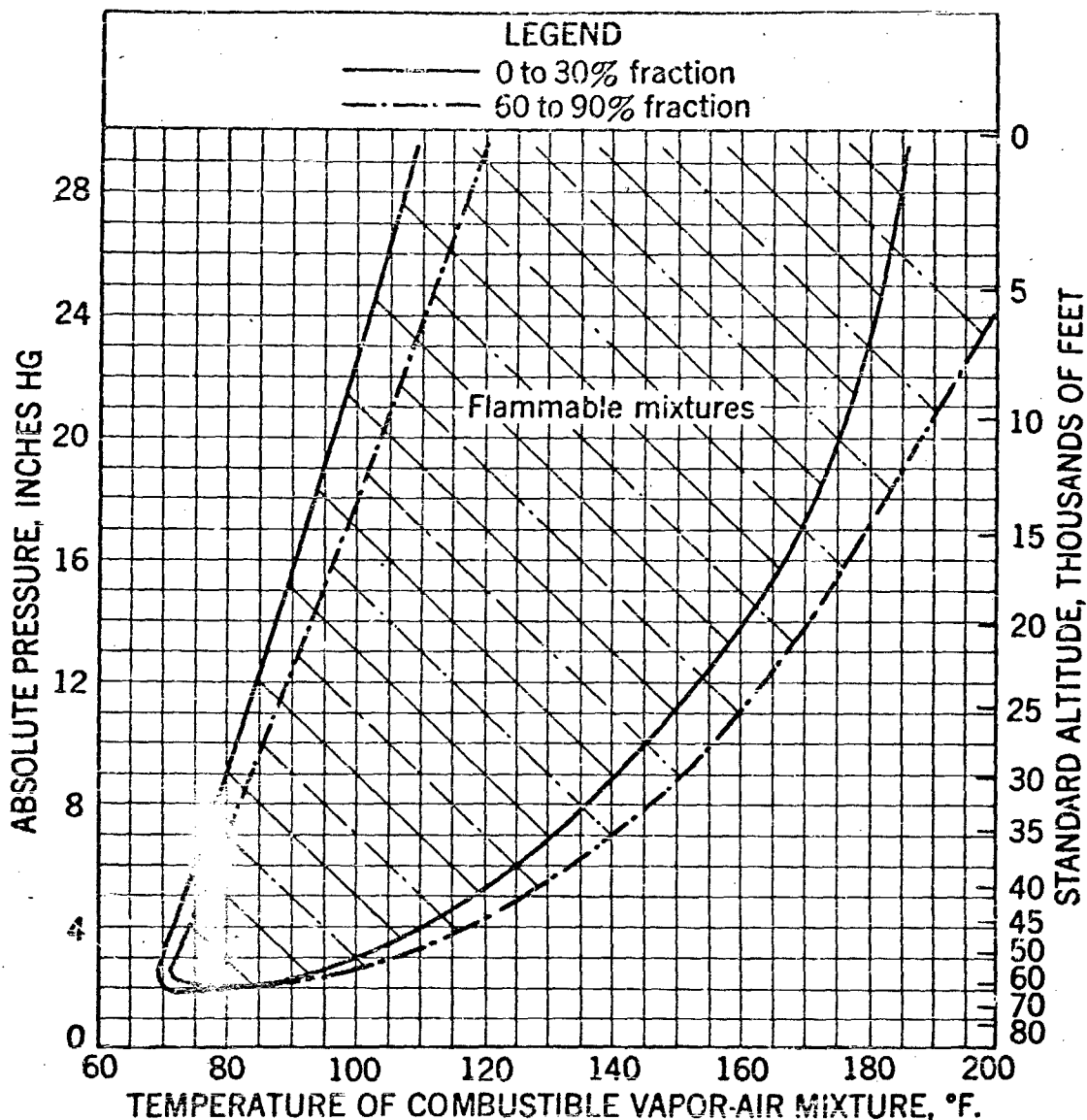
Figure 13 - Equilibrium concentration limits of flammability of the 0 to 30% and 60 to 90% fractions of aviation jet fuel grade JP-1 vapor-air mixtures over the temperature range 60 to 200° F. (the 0 to 30 and 60 to 90% fractions of this fuel were distilled under the temperature and pressure conditions of each test).
