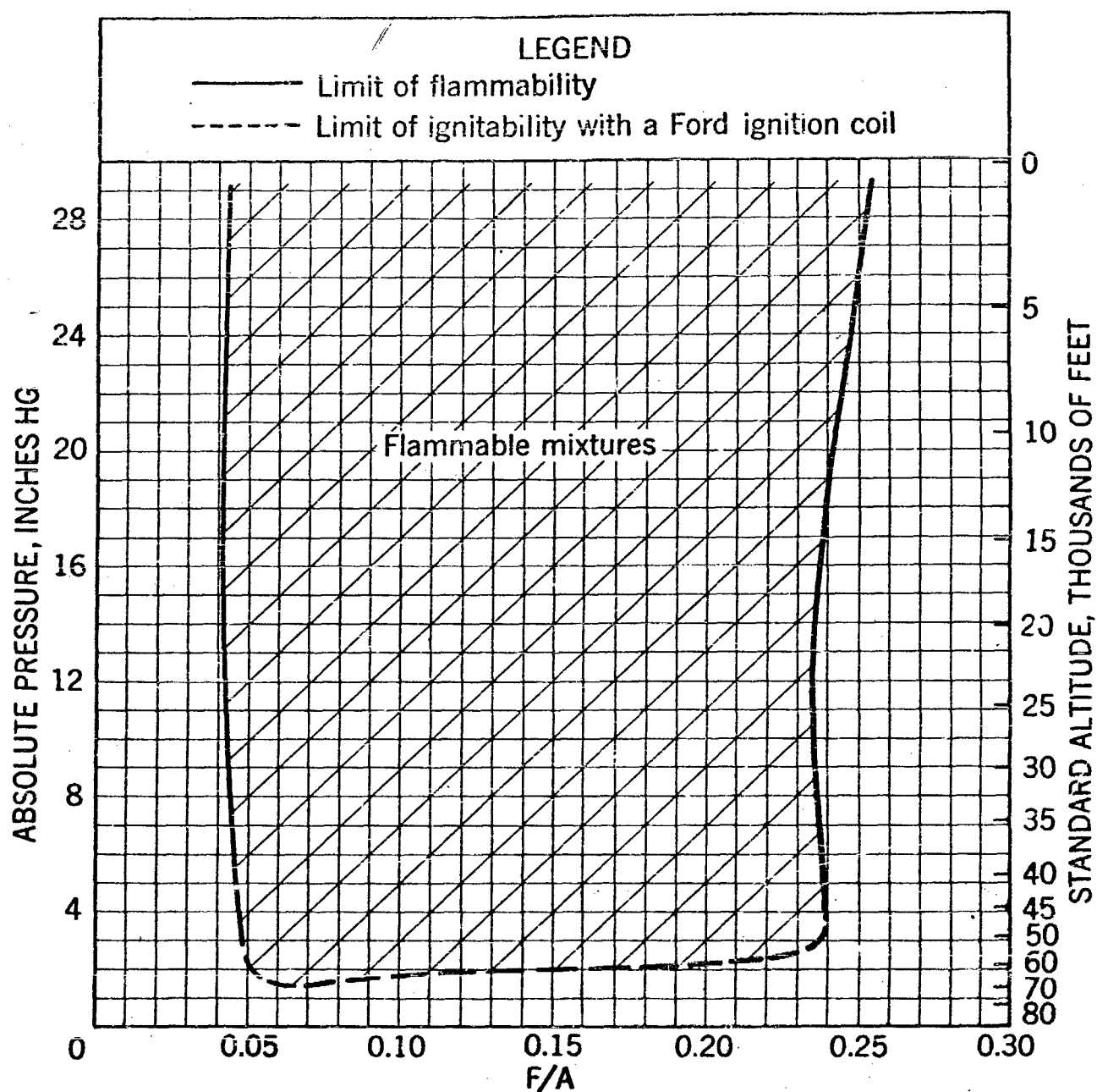
Figure 9b. - Concentration limits of flammability for aviation gasoline grade 115/145 vapor-air mixtures at 78 \pm 2^\circ\text{F} . (curve obtained from figure 9a taking average molecular weight of this fuel to be 100).
