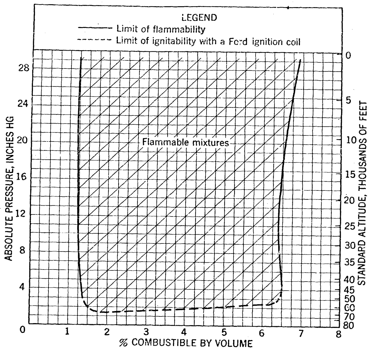
Figure 9a. - Concentration limits of flammability for aviation gasoline grade 115/145 vapor-air mixtures at 78 \pm 2^\circ \text{F} .
