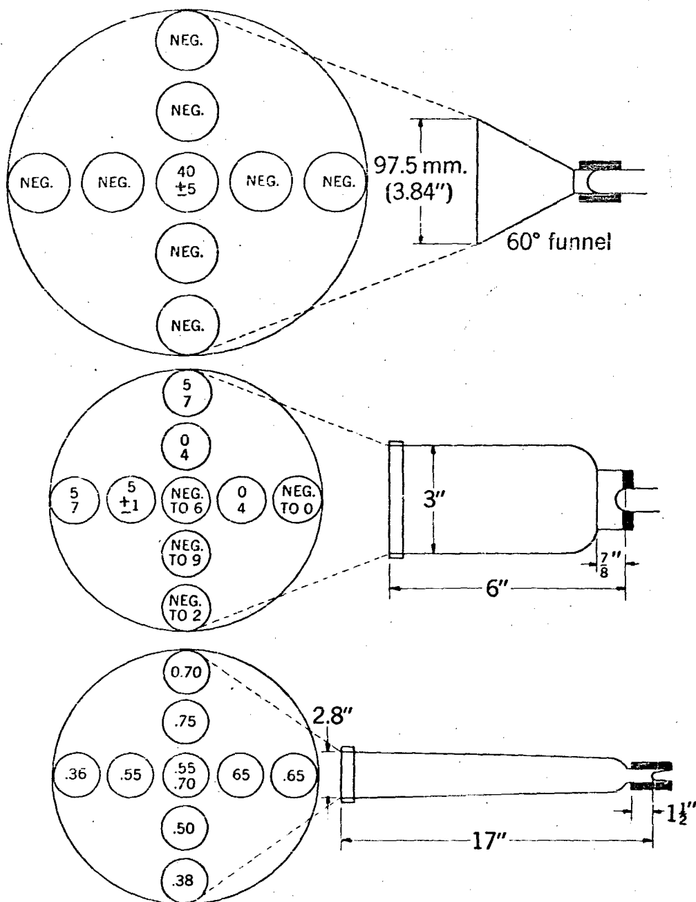
Figure 22. Total air velocities due to the primary air from a two fluid nozzle plus the entrained secondary air for three exit chambers attached to the nozzle, (large circles represent chamber outlets, numbers in small circles are velocities in hundreds of feet per minute).
