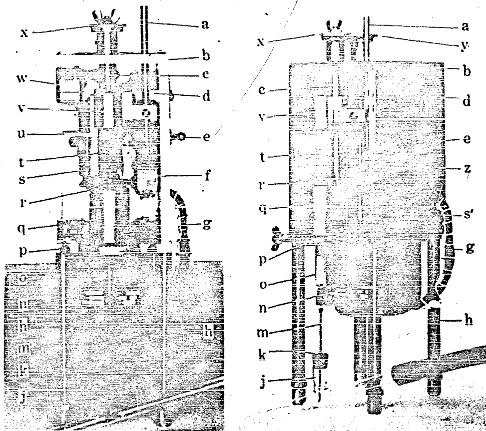
Figure 34a. - An improved model of of the liquid feed service used with the F-11 limit of flammability apparatus.
