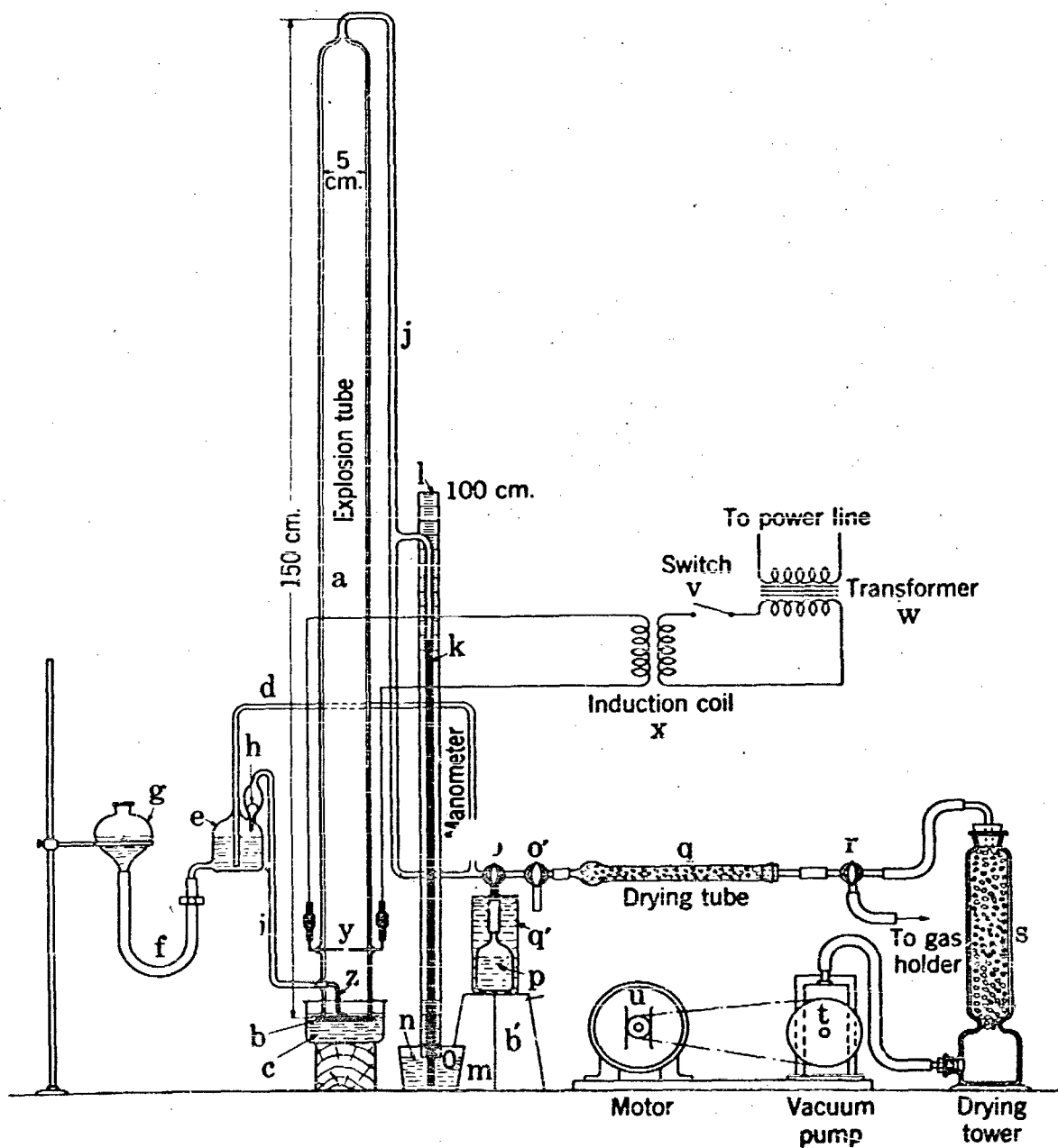
Figure 24. - Schematic diagram of the F-1 limit of flammability apparatus.
