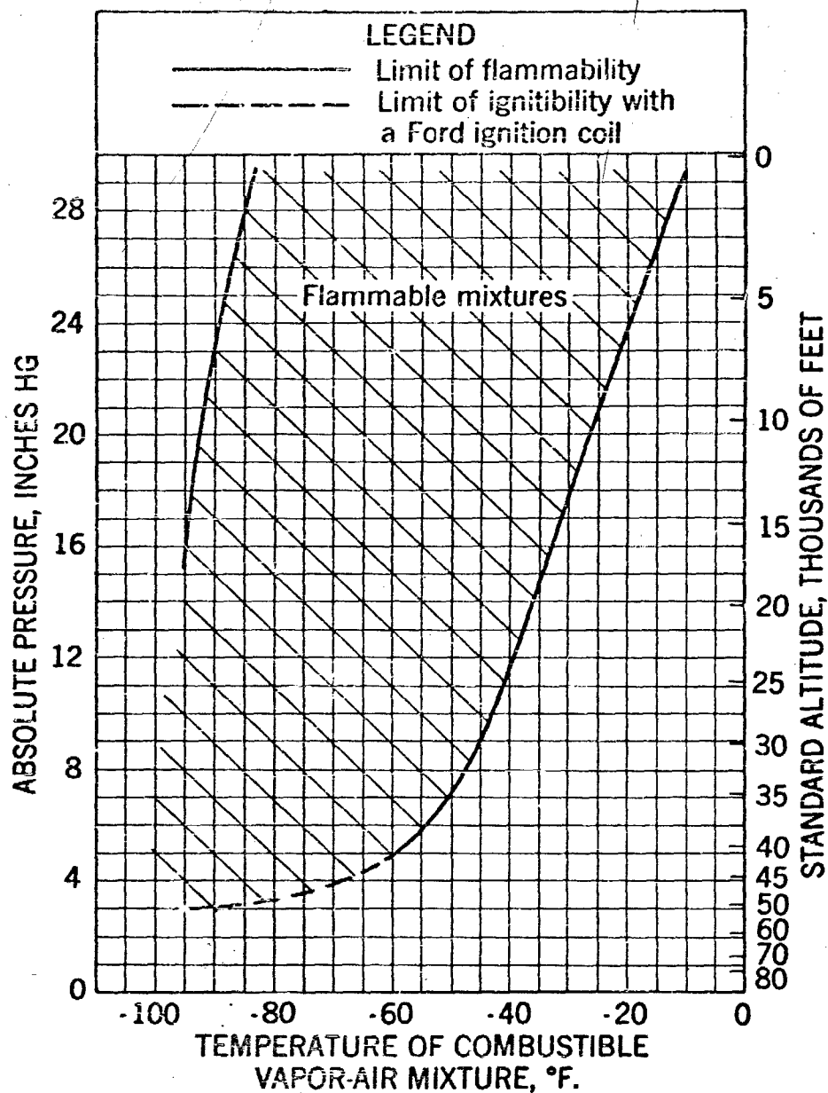
Figure 12 - Equilibrium concentration limits of flammability of the 0 to 10% fraction of aviation gasoline grade 115/145 vapor-air mixtures over the temperature range -100 to 0° F. (the 0 to 10% fraction of this fuel was distilled under the temperature and pressure conditions of each test)
