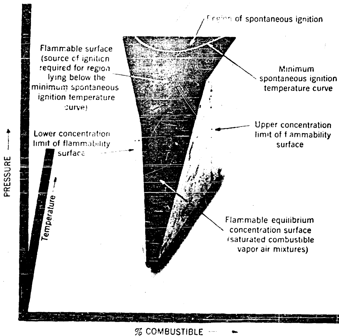
Figure 6. A general flammable volume of a combustible vapor air mixture.
