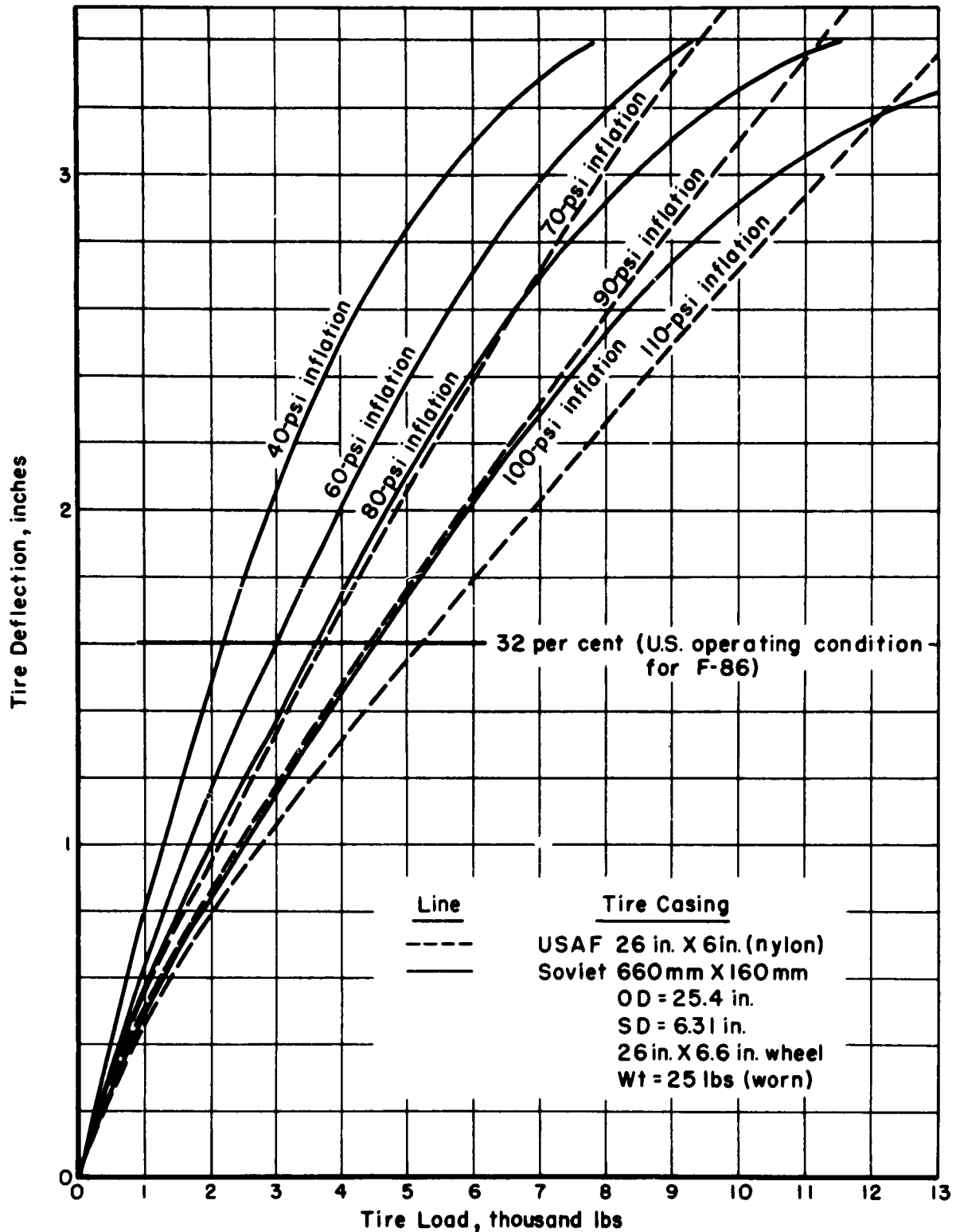
FIGURE 5. LOAD-DEFLECTION CURVES, COMPARING THE MIG-15 TIRE CASING WITH A U.S. TIRE CASING OF SIMILAR SIZE (WITH NYLON-CORD PLIES)
