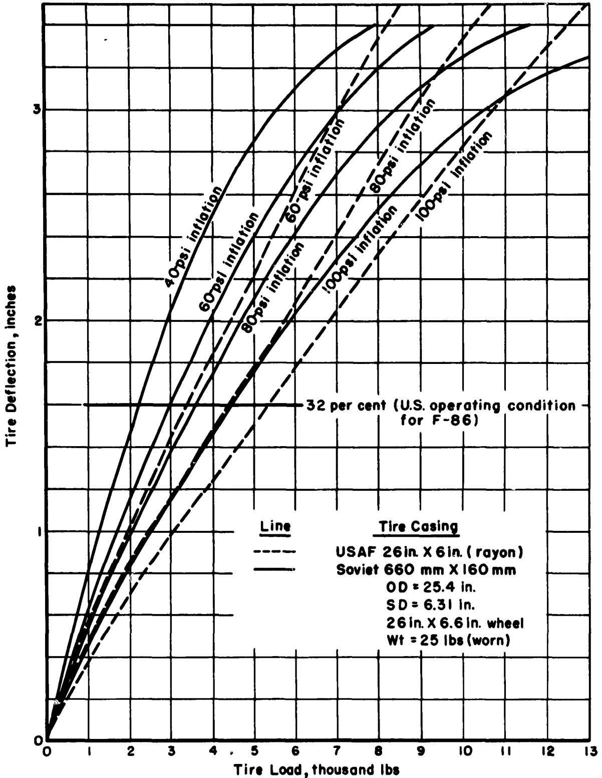
FIGURE 4. LOAD-DEFLECTION CURVES, COMPARING THE MIG-15 TIRE CASING WITH A U.S. TIRE CASING OF SIMILAR SIZE (WITH RAYON-CORD PLIES)
