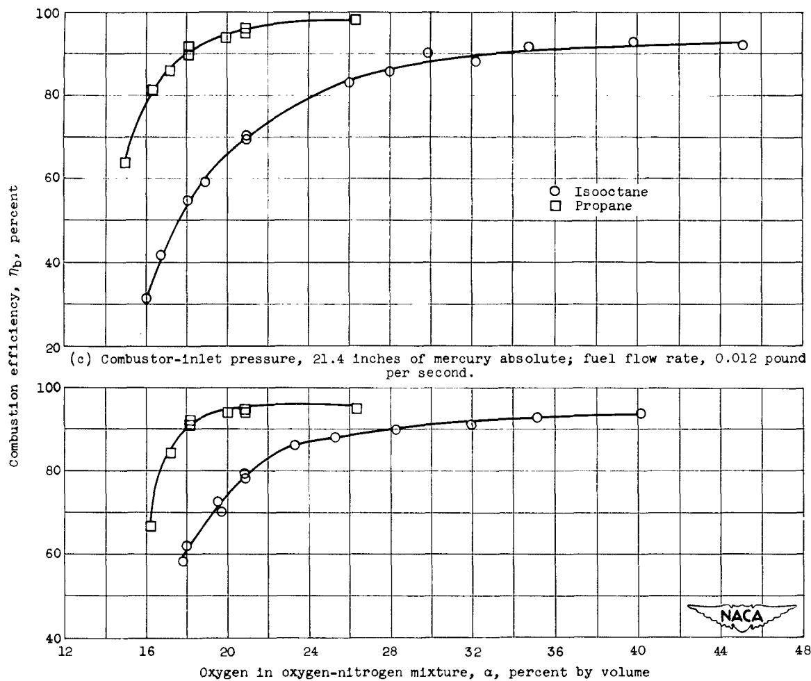
Figure 7. - Concluded. Comparison of combustion efficiency of single J33 combustor operating with propane and isooctane fuels. Combustor-inlet temperature, 40° F; weight flow rate of inlet oxygen-nitrogen mixture, 1.0 pound per second.
