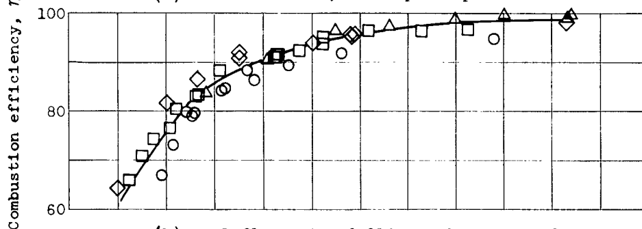
(b) Fuel flow rate, 0.012 pound per second.
