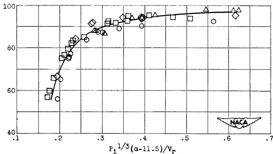
(c) Fuel flow rate, 0.016 pound per second.
