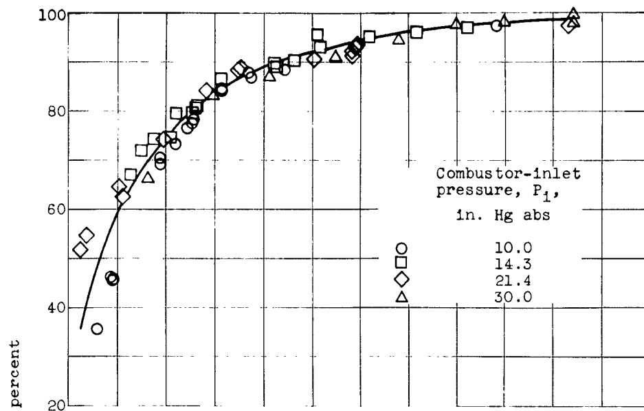
(a) Fuel flow rate, 0.008 pound per second.
