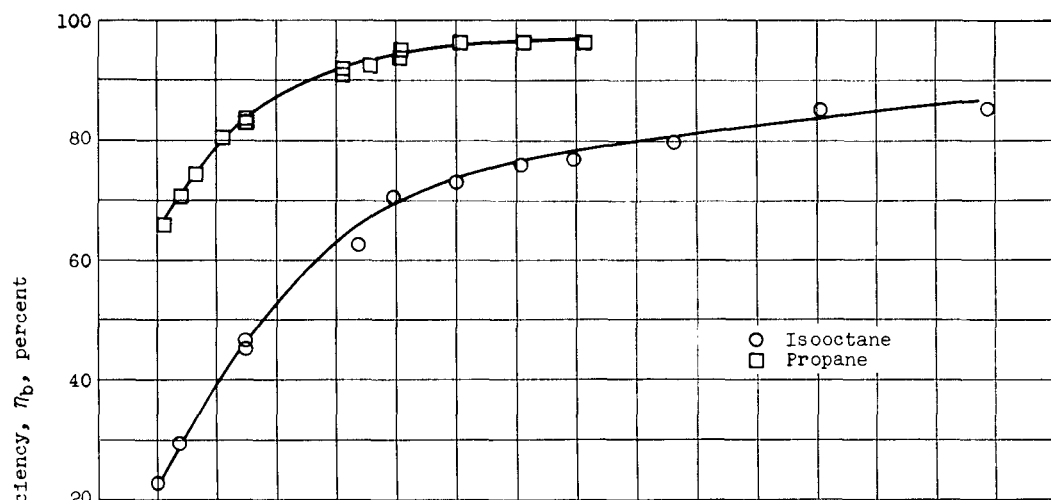
(a) Combustor-inlet pressure, 14.3 inches of mercury absolute; fuel flow rate, 0.012 pound per second.
