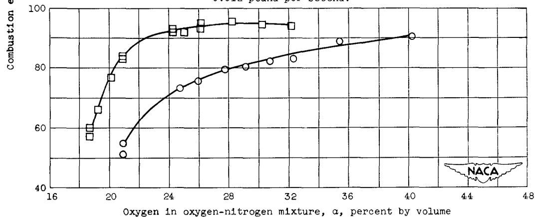
(b) Combustor-inlet pressure, 14.3 inches of mercury absolute; fuel flow rate, 0.016 pound per second.
