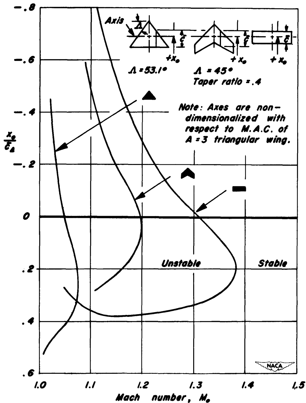
Figure 2. - Comparison of theoretical single-degree-of-freedom short-period pitching stability boundaries at supersonic speeds for three wings of aspect ratio 3, having triangular, swept, and rectangular plan forms.
