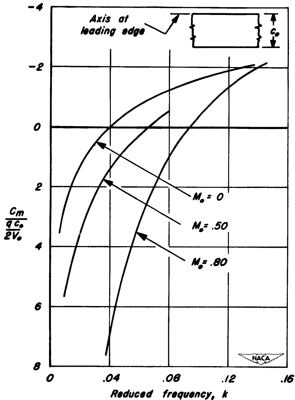
Figure 5.—The variation with reduced frequency of the single-degree-of-freedom rotary damping – moment coefficient for the two-dimensional wing at Mach numbers 0, 0.50, and 0.80. Axis at leading edge.
