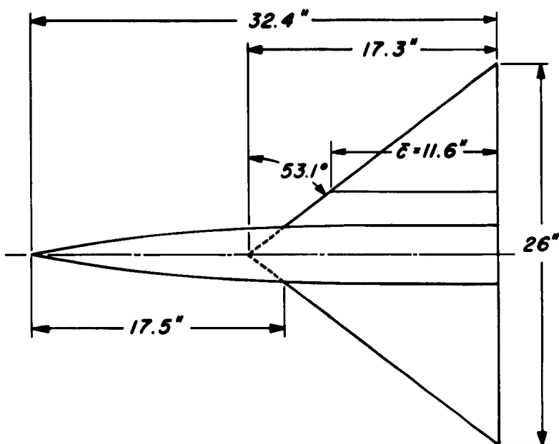
(b) A = 3 triangular wing (NACA 0003-63 sections).
