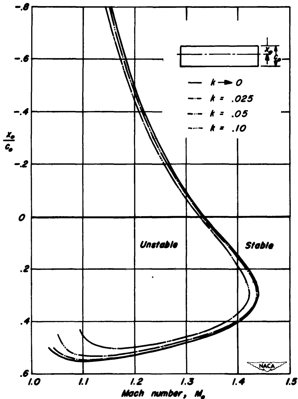
Figure 4. — The effect of frequency on the theoretical single-degree-of-freedom short-period pitching stability boundaries at supersonic speeds for a rectangular wing of aspect ratio 4.
