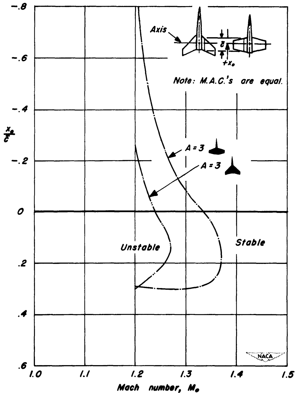
Figure 27.— Comparison of experimental single-degree-of-freedom short-period pitching stability boundaries for two wing-body combinations having swept and unswept wings of aspect ratio 3.
