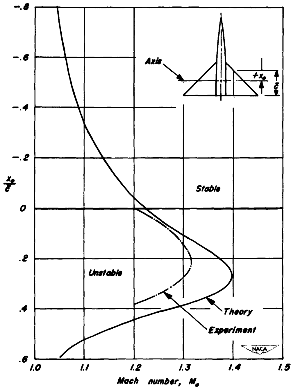
Figure 25.—Comparison of theoretical and experimental single-degree-of-freedom short-period pitching stability boundaries for a wing-body combination having a triangular wing of aspect ratio 4.
