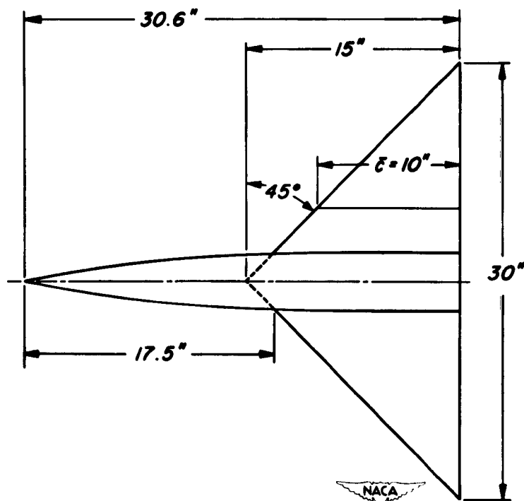
(c) A = 4 triangular wing (3% biconvex circular-arc sections).
