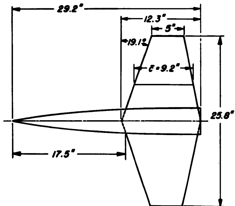
(e) A=3 unswept wing (3% biconvex circular-arc sections).
