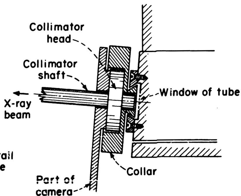
Fig. 2. Side section of shield with collimator in place.
