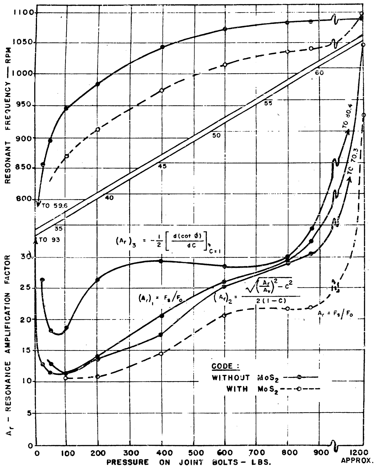
FIG.14. RESONANCE AMPLIFICATION FACTORS AND RESONANT FREQUENCIES OF JOINT WITH AND WITHOUT \text{MoS}_2 . A_r DETERMINED BY THREE METHODS.
