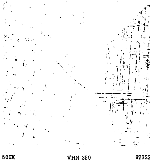
FIGURE 81. 2.35 PER CENT Cr ALLOY ISOTHERMALLY TRANSFORMED FOR 1 HOUR AT 1112 F Structure: Widmanstätten Alpha Plus TiCr 2 in a Beta Matrix
