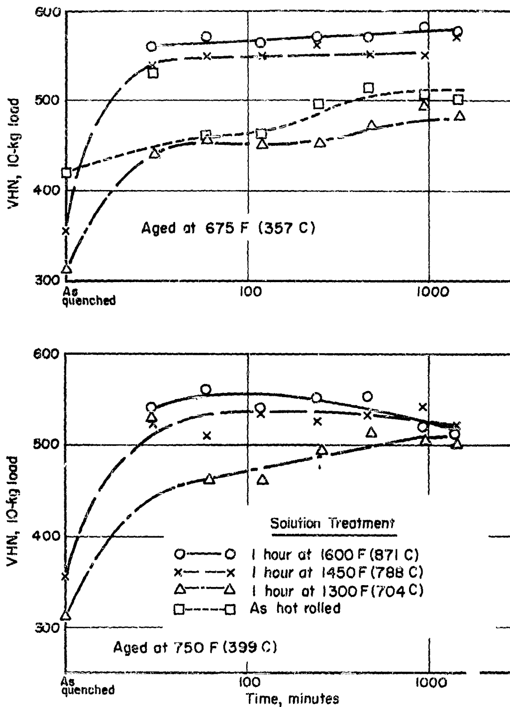
FIGURE 123. HARDNESS VERSUS AGING TIME FOR A Ti-2% Mn-5% Cr ALLOY SOLUTION TREATED AT VARIOUS TEMPERATURES
