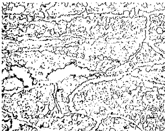
FIGURE 25. 20 PER CENT Cr ALLOY COLD ROLLED 30 PER CENT AND ANNEALED 6 HOURS AT 1112 F (600 C) Structure: TiCr_2 Plus Eutectoid in Beta Matrix, No Recrystallization
