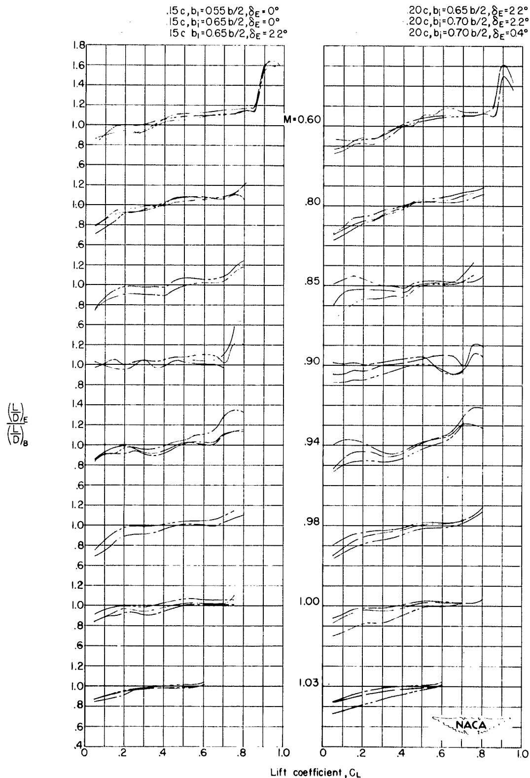
Figure 14.- Effect of leading-edge chord-extensions on the lift-drag ratio of the wing-normal configurations.
