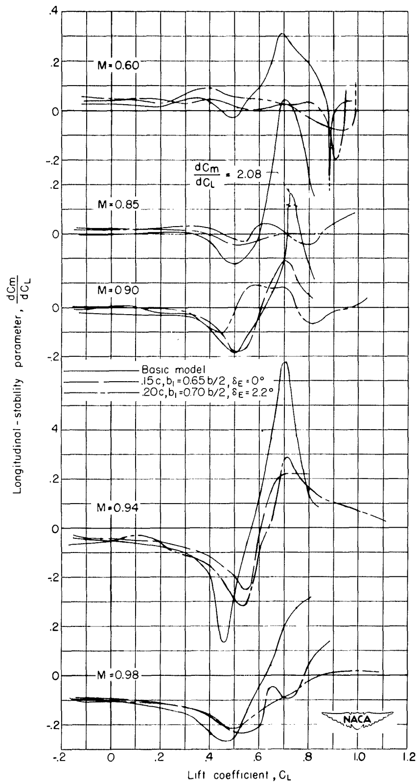
Figure 9.- Variation of longitudinal-stability parameter with lift coefficient at several Mach numbers for three wing-normal configurations.
