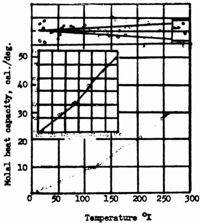
Fig. 1 - Heat capacities of dimethylhydrazine.
