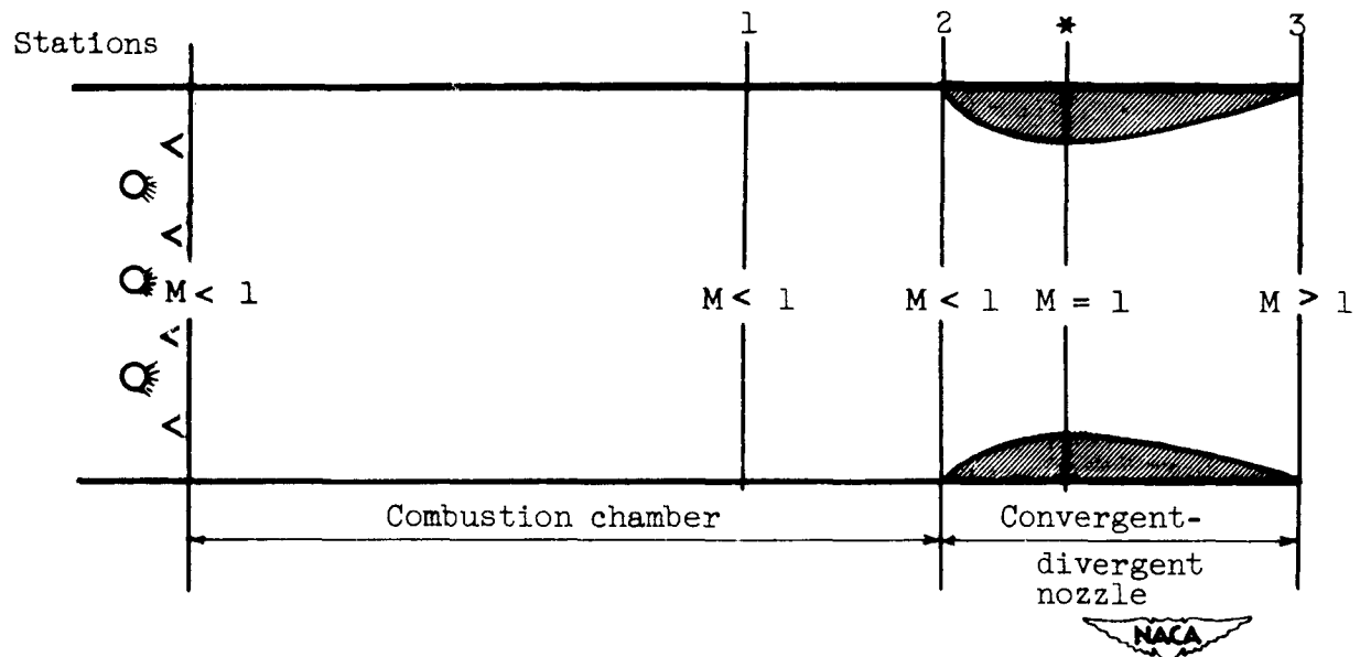
Figure 1. - Schematic diagram of typical convergent-divergent nozzle application.
