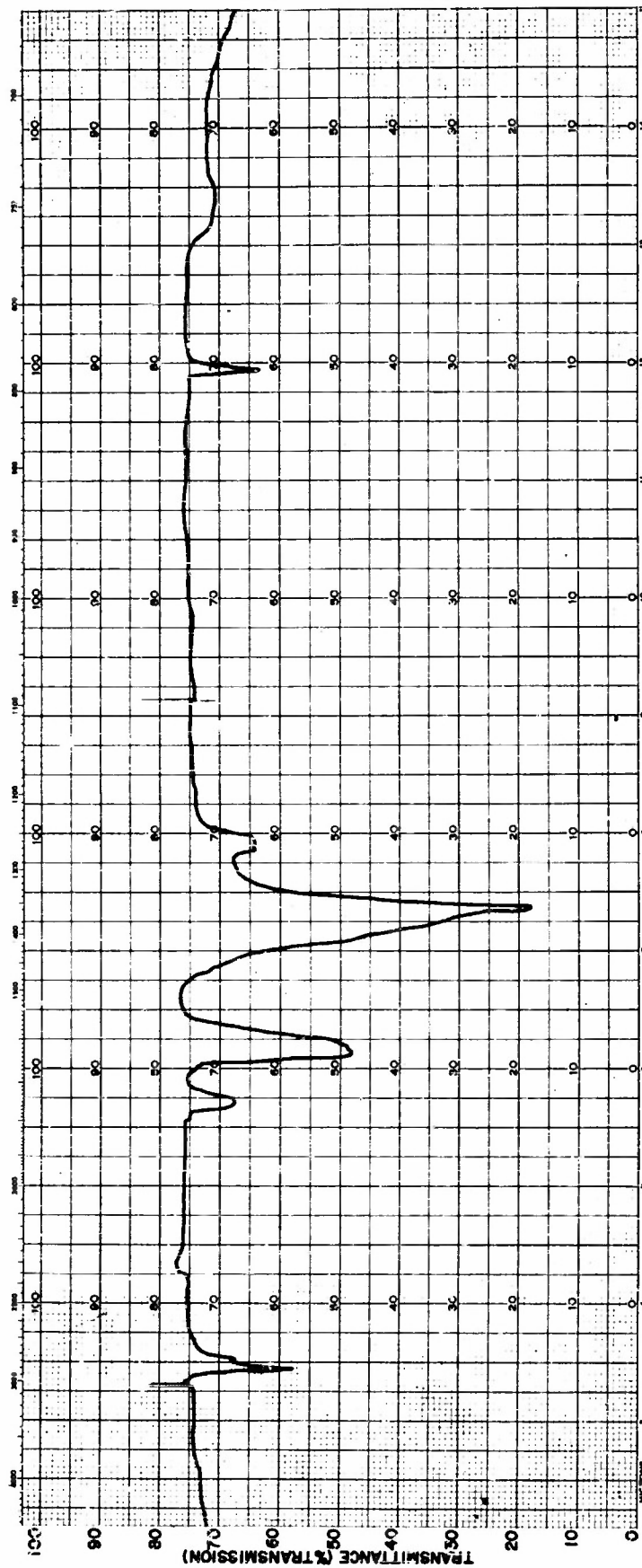
FIG. 5 NITROGEN DI-AND TETROXIDE
