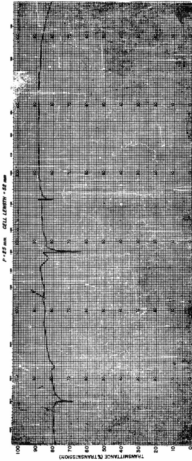
WAVELENGTH (MICRONS) FIG. 24 METHANE
