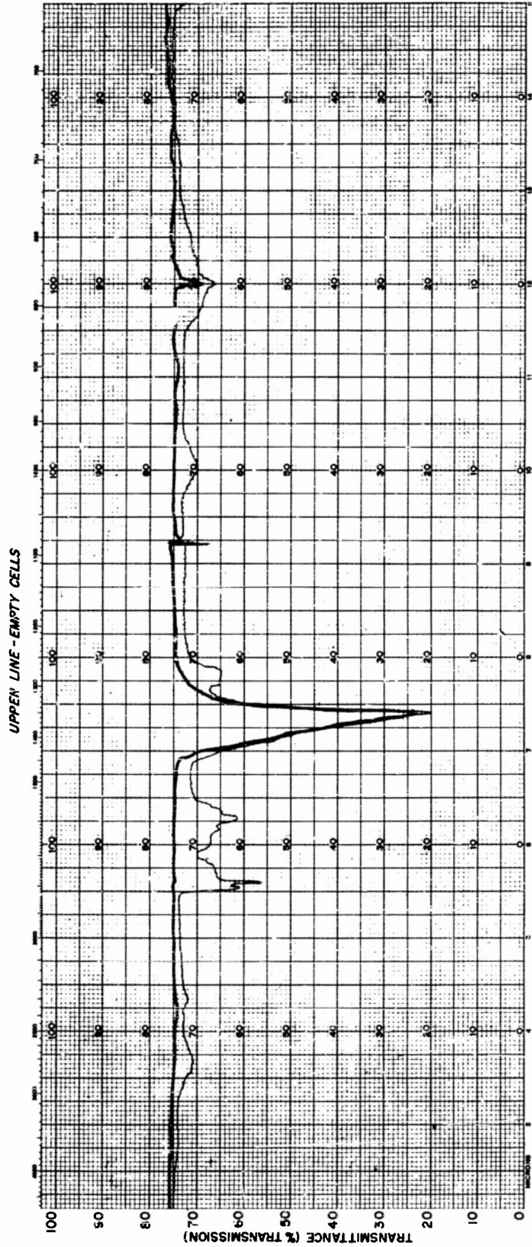
FIG 13 SPECTRUM OF 33.4% DECOMPOSITION MIXTURE ETHYL NITRATE AND ETHYL NITRITE BLANKED OUT
