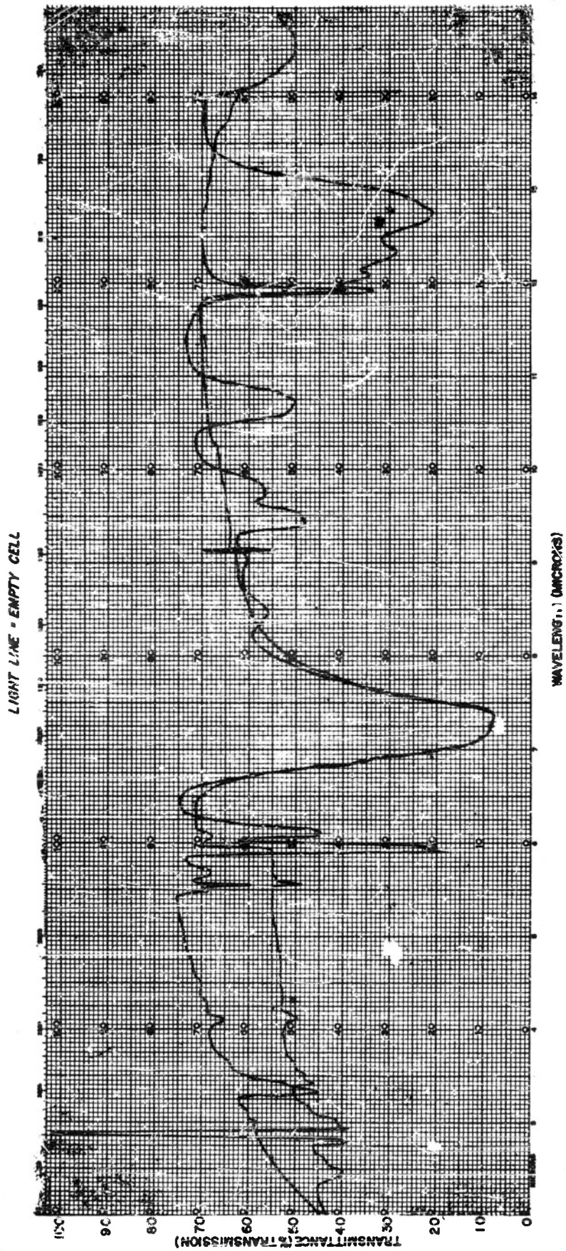
FIG. 33 THE PRODUCTS OF THE REACTION BETWEEN NITROGEN DIOXIDE AND ETHYL ALCOHOL
