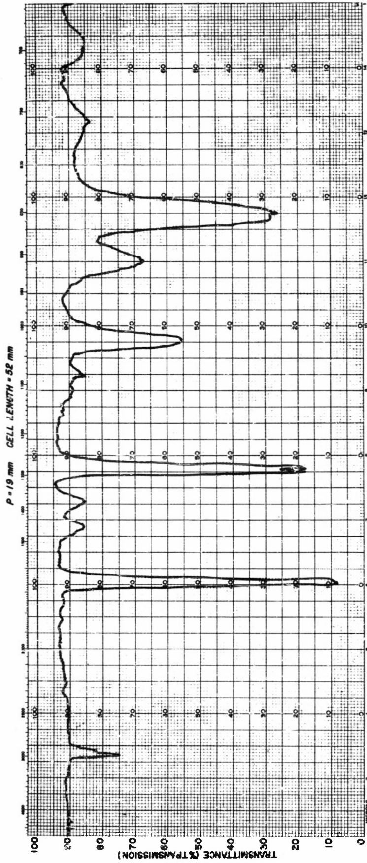
FIG. 3 ETHYL NITRATE
