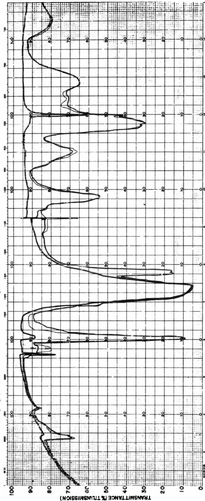
FIG. 10 DUPLICATION OF SPECTRUM OF PRODUCTS OF ETHYL NITRATE DECOMPOSITION 44.0 % DECOMPOSITION
