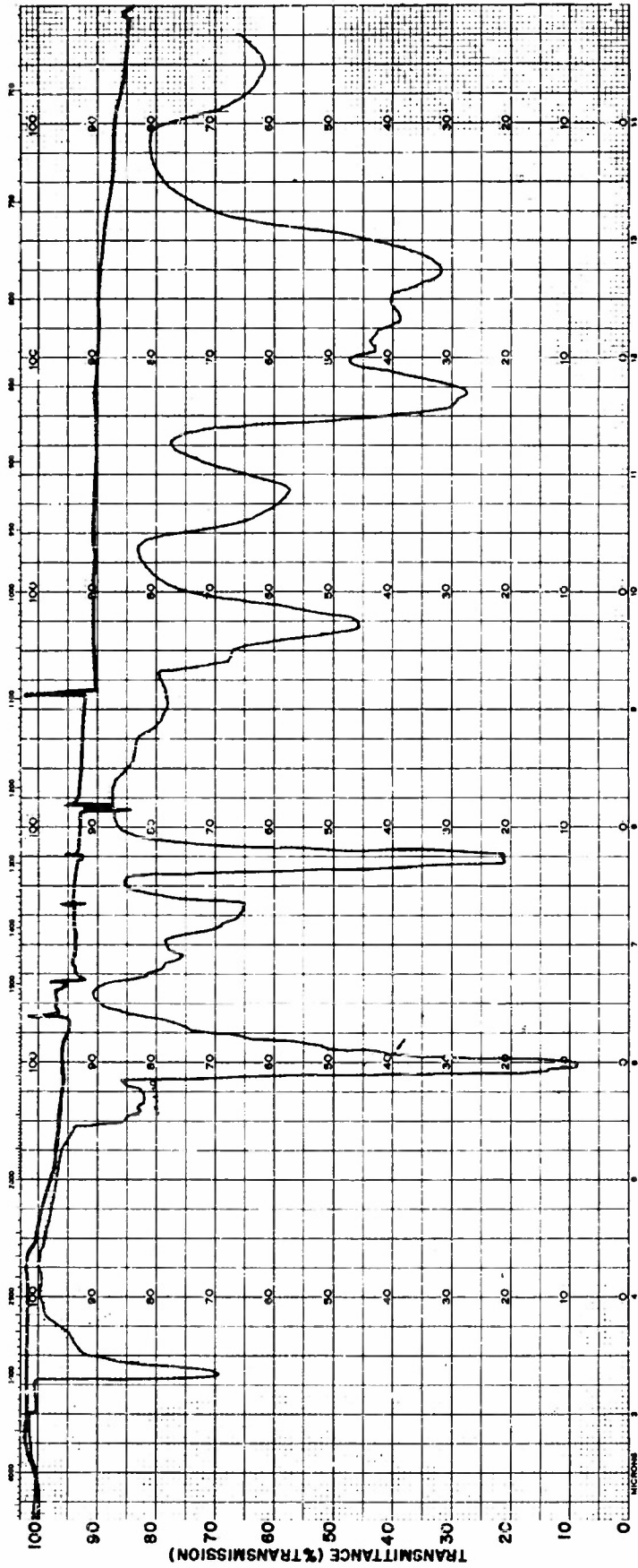
FIG. 1 PRODUCTS FROM 60% THERMAL DECOMPOSITION OF ETHYL NITRATE AT 181° C
