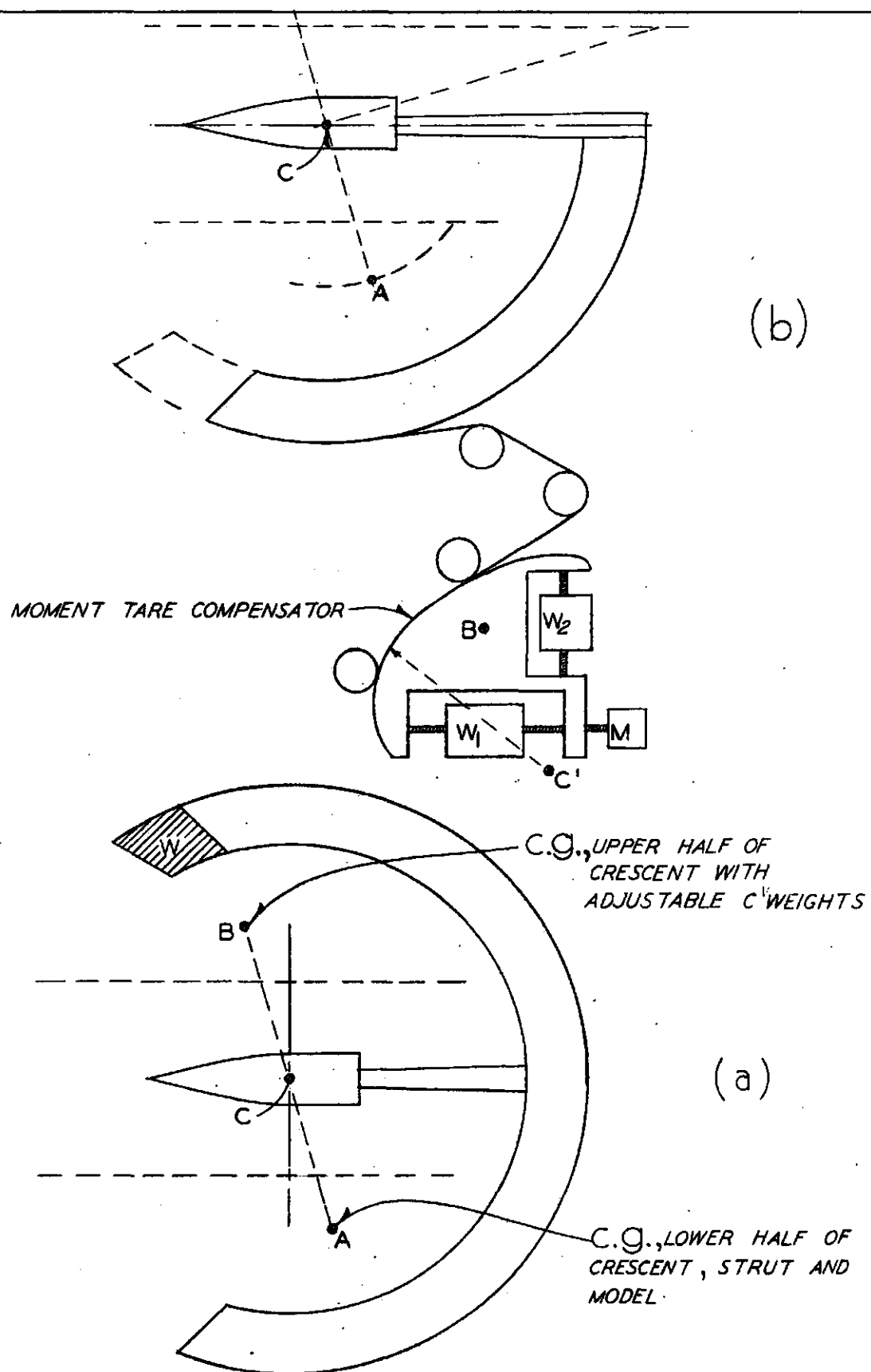
FIG. 2 MOMENT TARE COMPENSATOR
