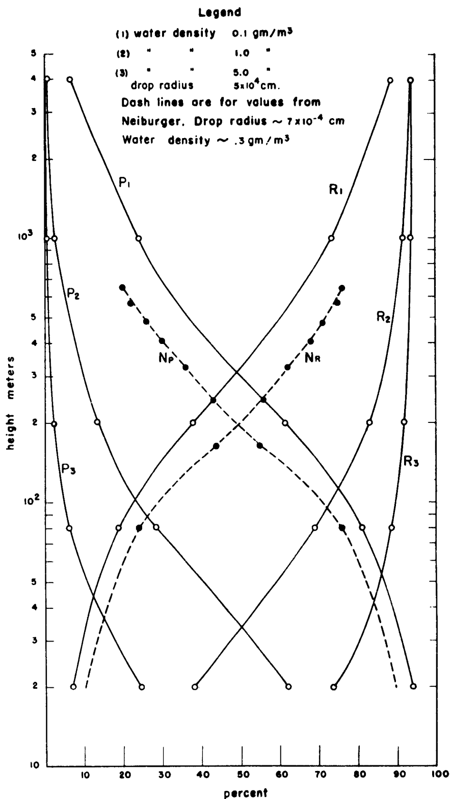
Fig. 16. Relationship between reflectivity (R), transmissivity (P) and cloud depth (after Hewson).
