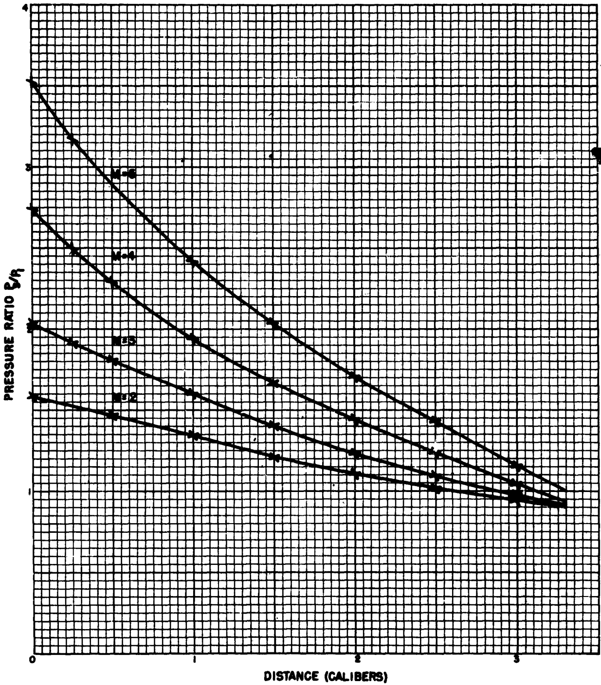
FIG. 1 PRESSURE DISTRIBUTION ON A 14 - CALIBER OGIVE
