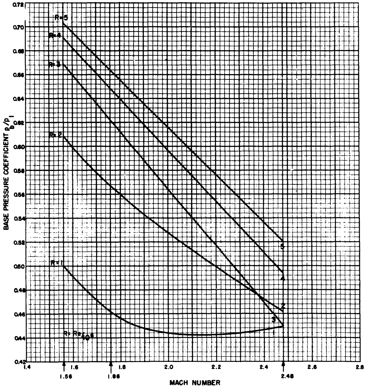
FIG. 9 BASE PRESSURE COEFFICIENT VS MACH NUMBER WITH REYNOLDS NUMBER, Re , AS PARAMETER
