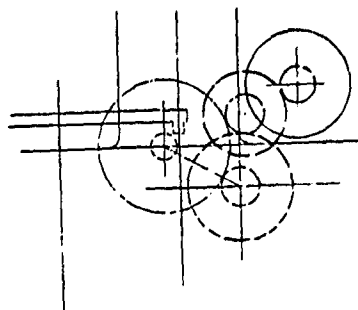
FIGURE 3-6 PRECISION MECHANISM - TWENTY-TURN HELIPOT MODEL 1 COMPUTER CONFIDENTIAL
