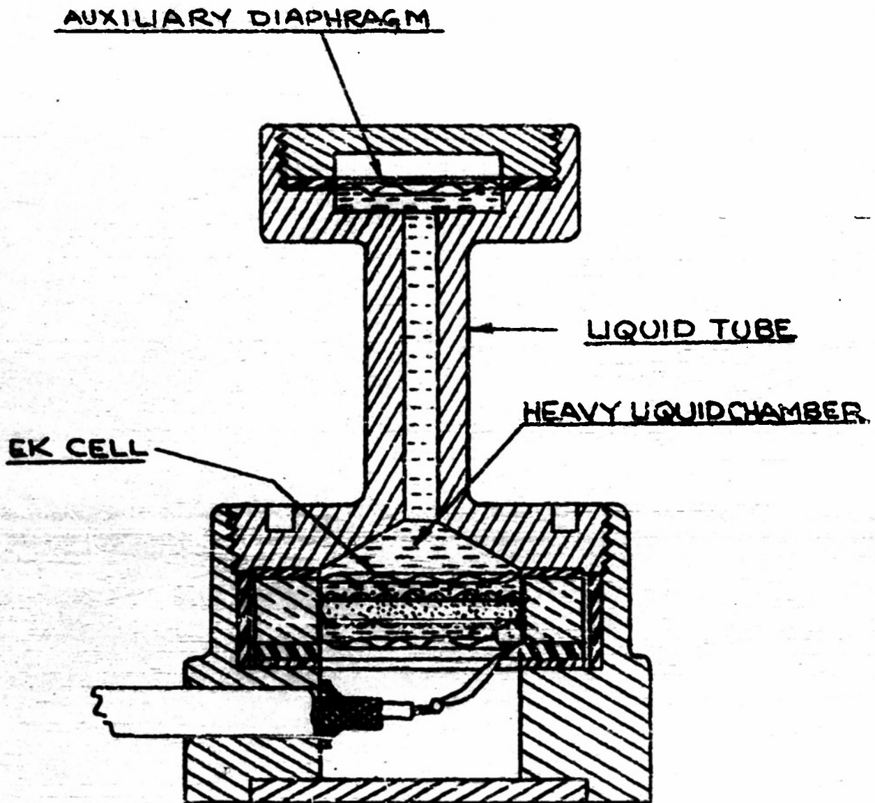
ELECTROKINETIC ACCELEROMETER
