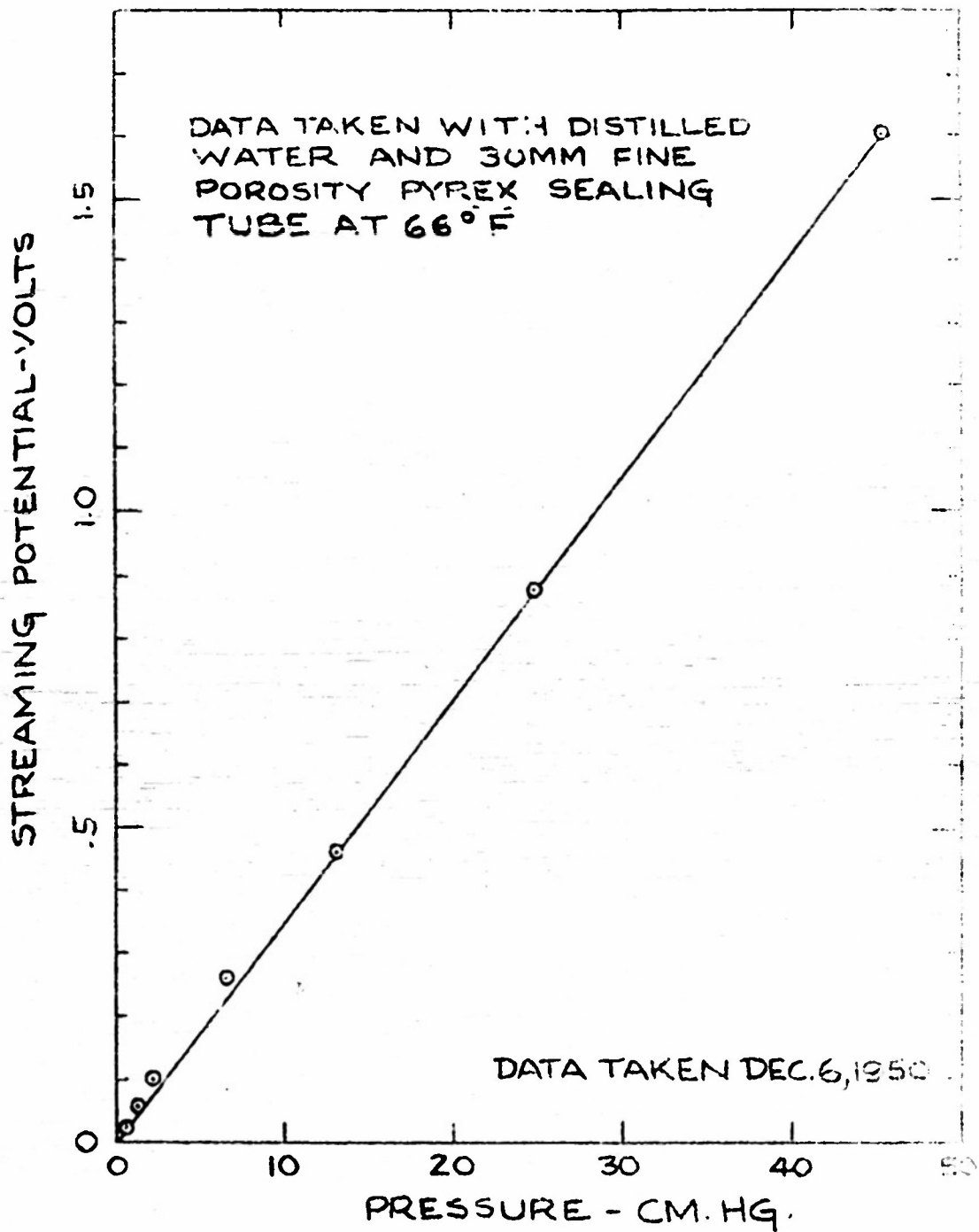
STREAM. POTENTIAL VS. PRESSURE
