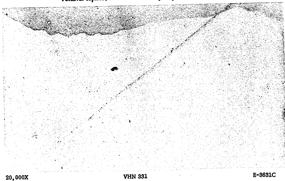
FIGURE 48. ELECTRON MICROGRAPH OF THE SAME SPECIMEN AS SHOWN IN FIGURE 47 AT HIGHER MAGNIFICATION AND USING SILICA REPLICA
