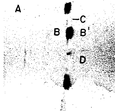
FIGURE 37. PORTION OF X-RAY DIFFRACTION PHOTOGRAPH OF Ti-7.72 Mn ALLOY TRANSFORMED 60 MINUTES AT 450 C
