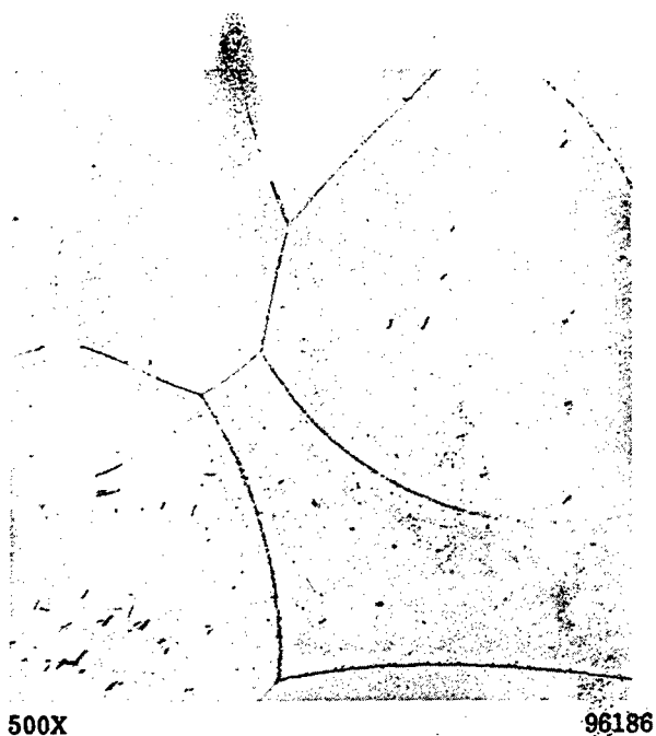
FIGURE 39. 12.3 PER CENT MANGANESE ALLOY ISOTHERMALLY TRANSFORMED AT 450 C FOR 30 MINUTES
