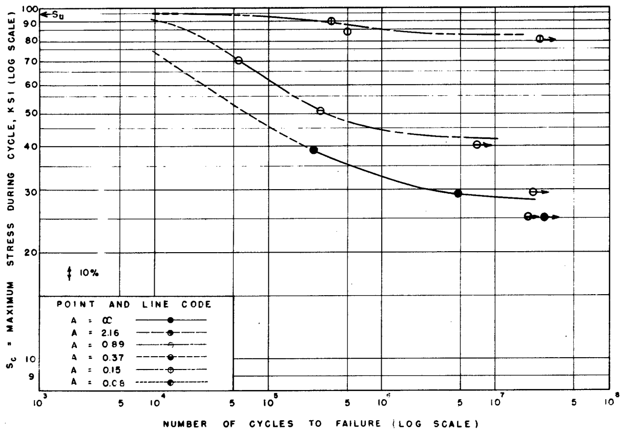
FIG.15. S-N FATIGUE DIAGRAMS AT VARIOUS STRESS RATIOS FOR K_t = 1.0 SPECIMENS OF ALUMINUM ALLOY 75S-T6 (EXTRUDED)
