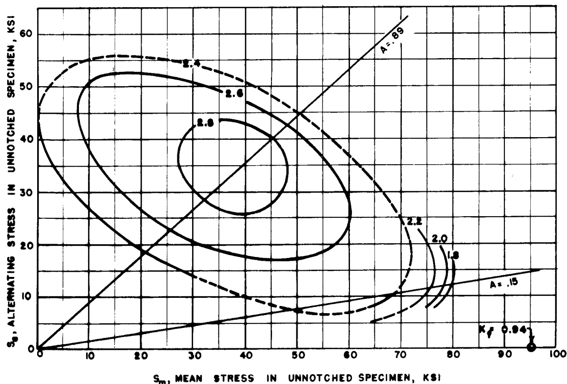
FIG.19. FATIGUE STRENGTH - REDUCTION "CONTOUR" CURVES FOR K_t = 3.4 SPECIMENS OF EXTRUDED ALUMINUM ALLOY 75S-T6 SHOWING K_t AS A FUNCTION OF S_a AND S_m OF THE UNNOTCHED SPECIMEN
