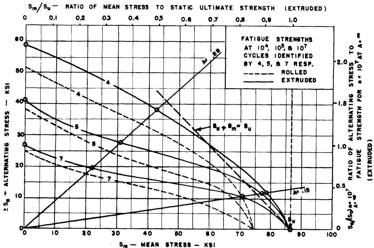
FIG.11. — STRESS RANGE FATIGUE DIAGRAM FOR K_f = 1.0 SPECIMENS OF EXTRUDED ALUMINUM ALLOY 24S-T6
