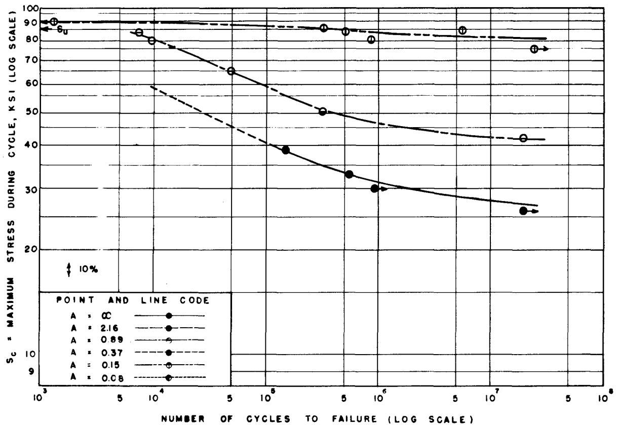
FIG.9. S-N FATIGUE DIAGRAMS AT VARIOUS STRESS RATIOS FOR K_t = 1.0 SPECIMENS OF ALUMINUM ALLOY 24S-T4 (EXTRUDED)
