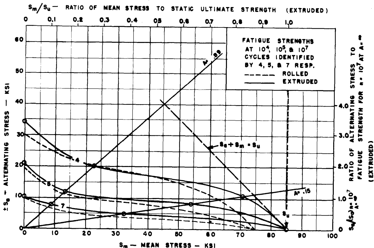
FIG.12. — STRESS RANGE FATIGUE DIAGRAM FOR K_f = 3.4 SPECIMENS OF EXTRUDED ALUMINUM ALLOY 24S-T6
