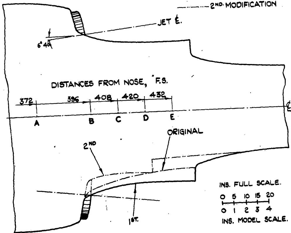
FIG.2. JET. EXIT FILLETS, SIDE & PLAN VIEWS.
