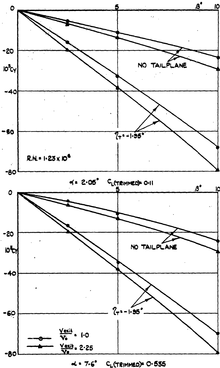
FIG. 17. SIDEFORCE COEFFICIENTS
