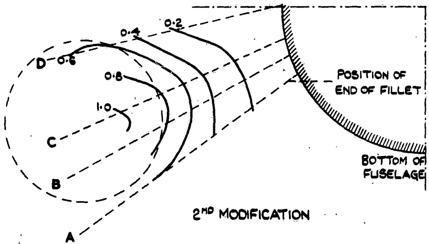
FIG. 5. VELOCITY DISTRIBUTION BEHIND THE MODIFIED JET EXIT FILLETS AT ZERO TUNNEL SPEED - EXIT VELOCITY - 210 FT/SEC.
