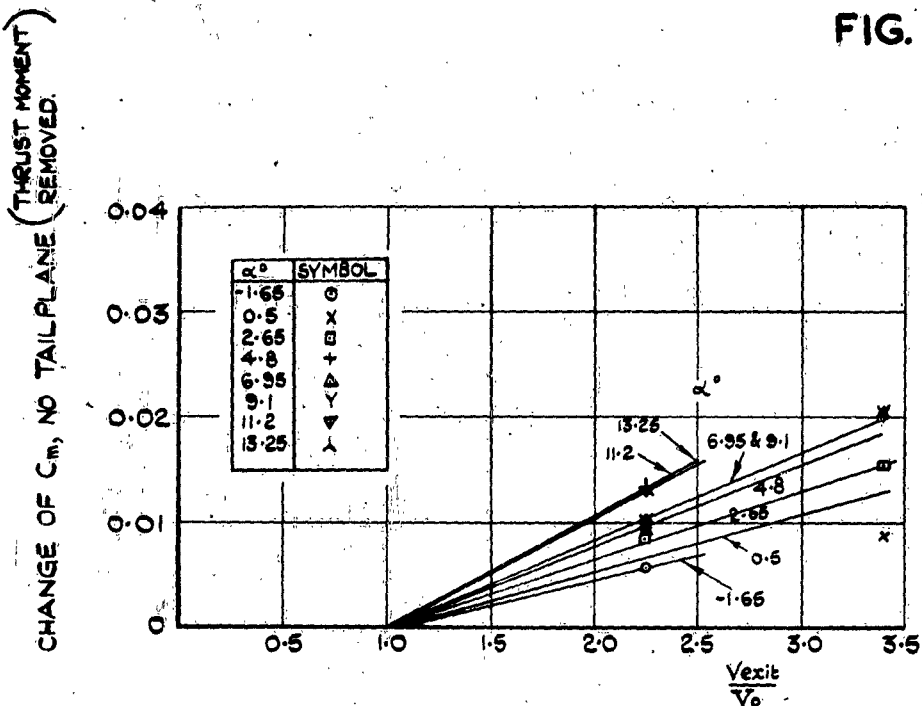
FIG. 9. EFFECT OF FLOW ON PITCHING MOMENT OF MODEL WITHOUT TAILPLANE. (PITCHING MOMENTS ARE GIVEN RELATIVE TO \frac{V_{exit}}{V_0} = 1.0 )
