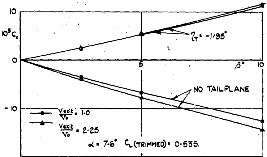
FIG. 15. YAWING MOMENT COEFFICIENTS.
