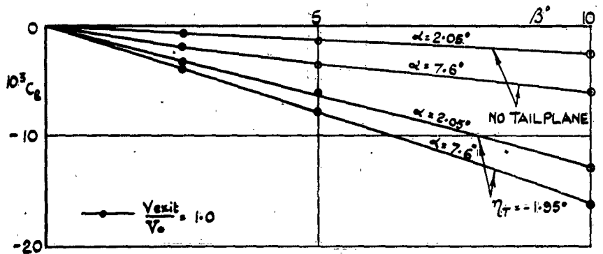
FIG. 16. ROLLING MOMENT COEFFICIENTS.
