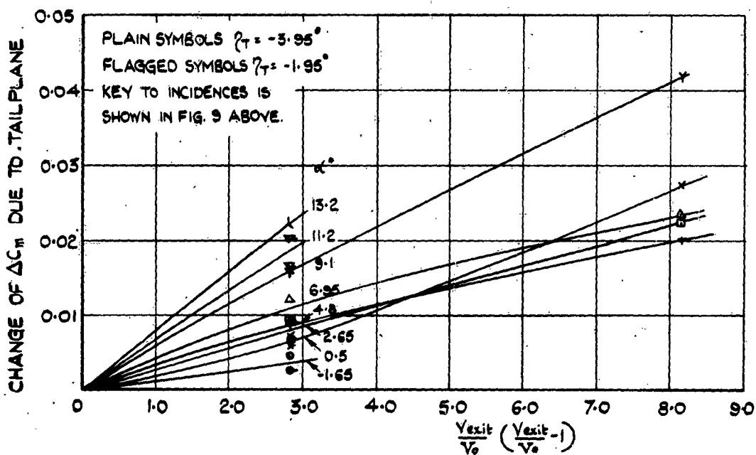
FIG. 10. EFFECT OF FLOW ON TAILPLANE CONTRIBUTION TO PITCHING MOMENT (PITCHING MOMENTS ARE GIVEN RELATIVE TO \frac{V_{exit}}{V_0} = 1.0 )
