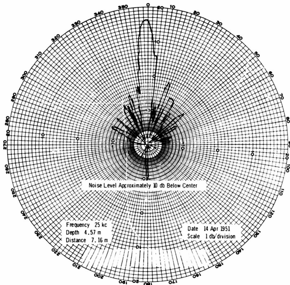
Figure 5 - Directivity of JT No. 231 Hydrophone, Frequency 25 kc
