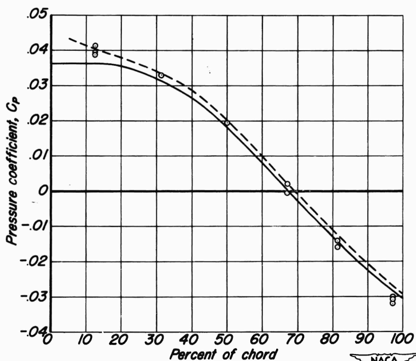
(b) M_o = 4.03 , Re = 2.88 \times 10^6
