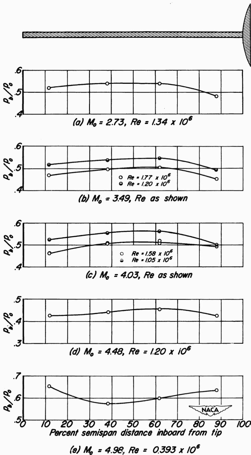
Figure 8.- Typical spanwise base-pressure distribution for airfoil 306-T with laminar boundary layer.
