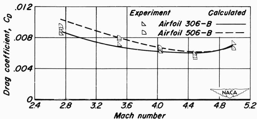
Figure 13.— Variation of drag coefficient with Mach number for airfoils 306-B and 506-B.
