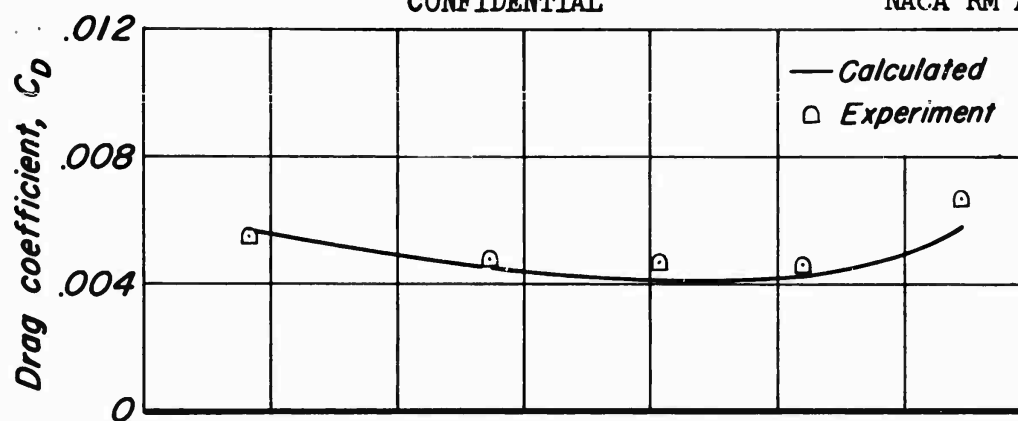
(g) Airfoil 304-B
