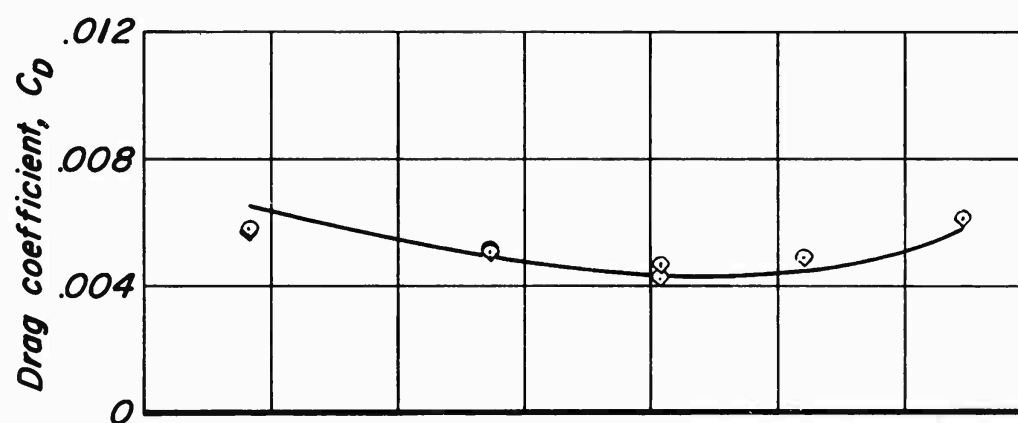
(h) Airfoil 504-B
