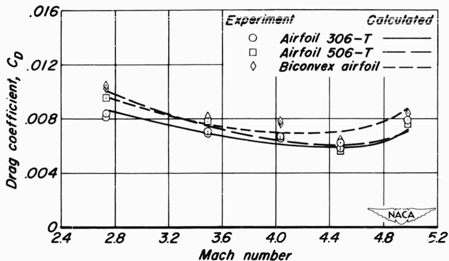
Figure 12.— Variation of drag coefficient with Mach number for airfoils 306-T, 506-T, and biconvex.
