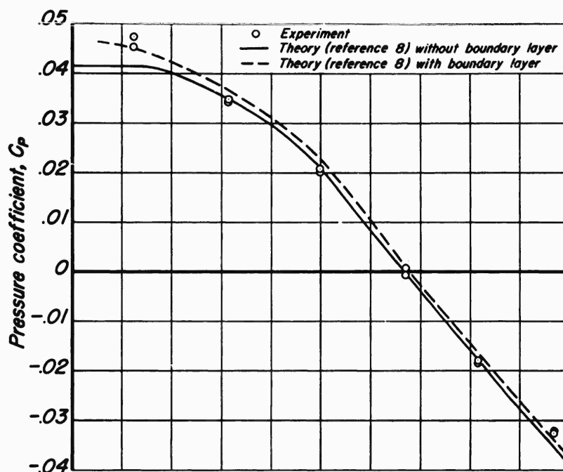
(a) M_o = 3.49 , Re = 3.63 \times 10^6
