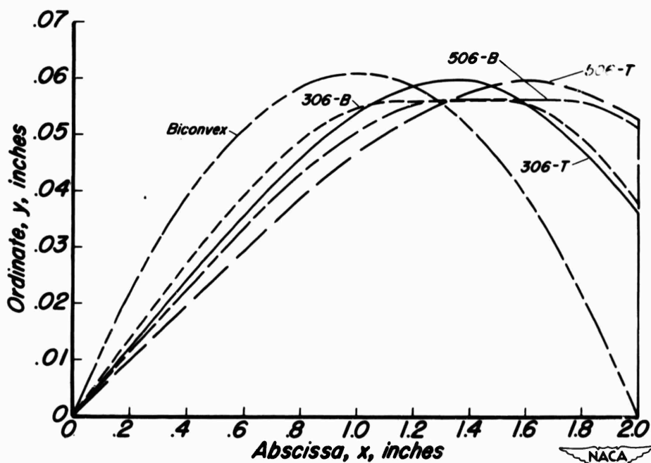
(b) Airfoils approximately 6 percent thick.
