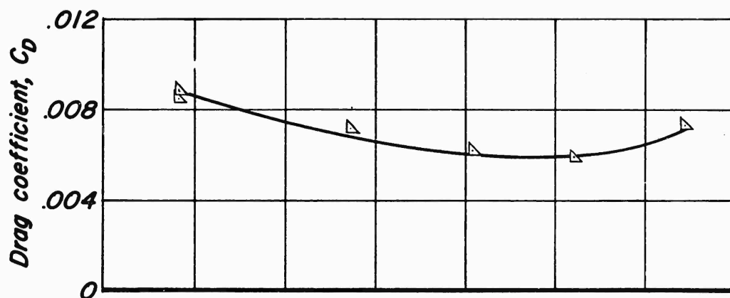
(e) Airfoil 306-B
