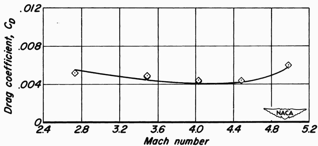
(c) Airfoil 304-T
