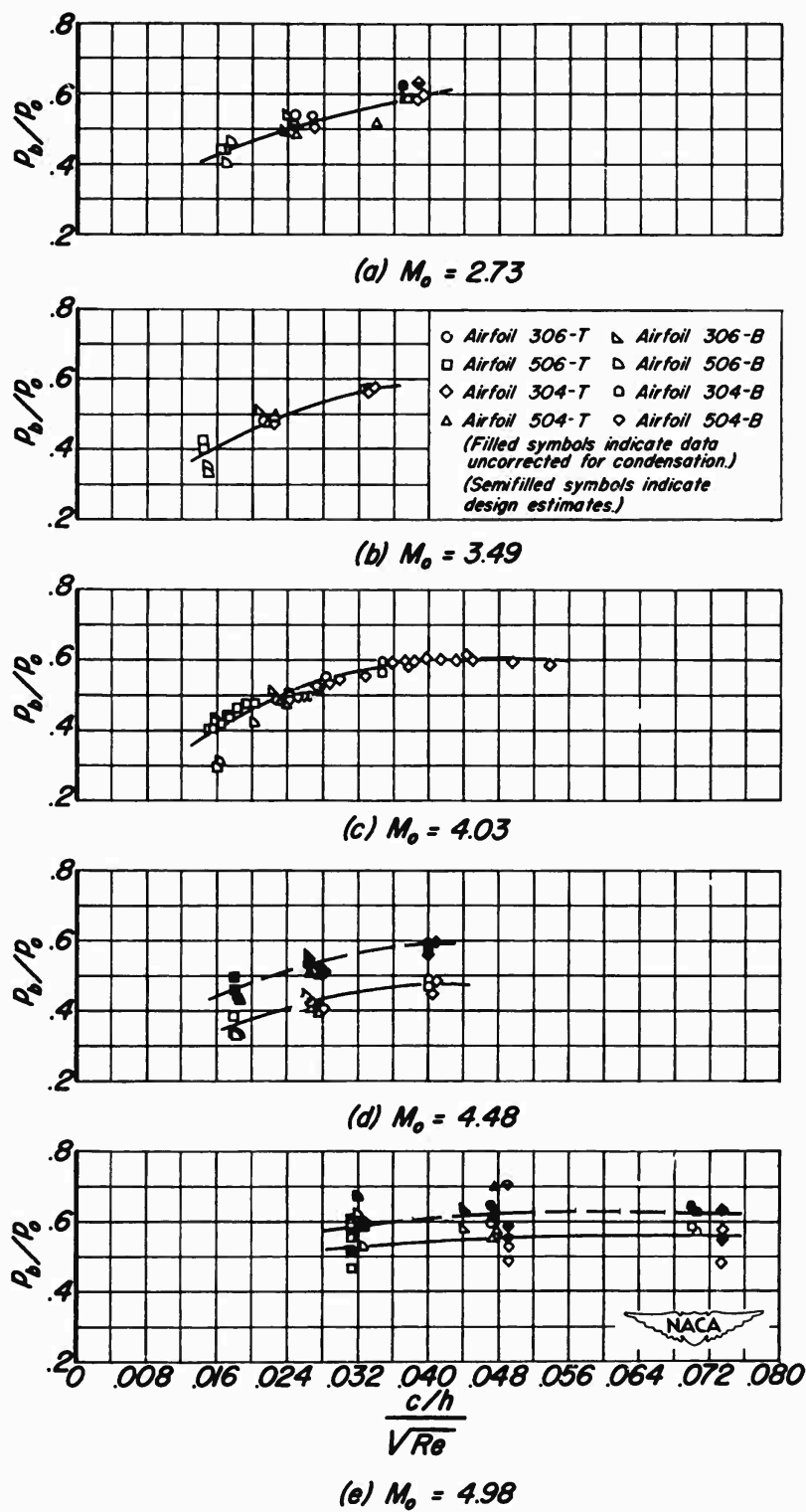
Figure 9.—Correlated base-pressure data.
