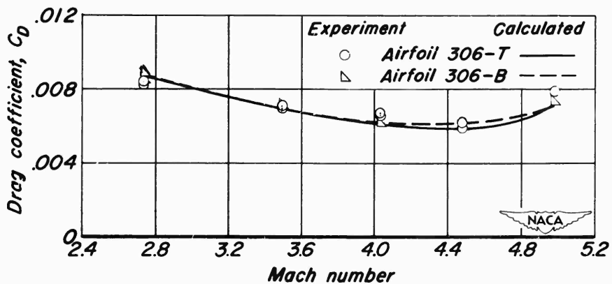
Figure 14.— Variation of drag coefficient with Mach number for airfoils 306-T and 306-B.
