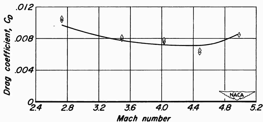
(i) Biconvex airfoil
