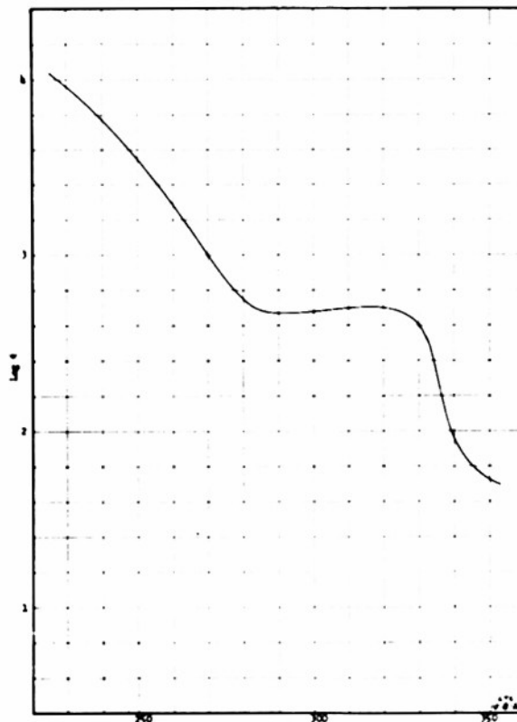
Ultraviolet Absorption Spectrum of 1,1,1,3,5,5-Hexamethyl-2-oxoheptane in Ethanol
