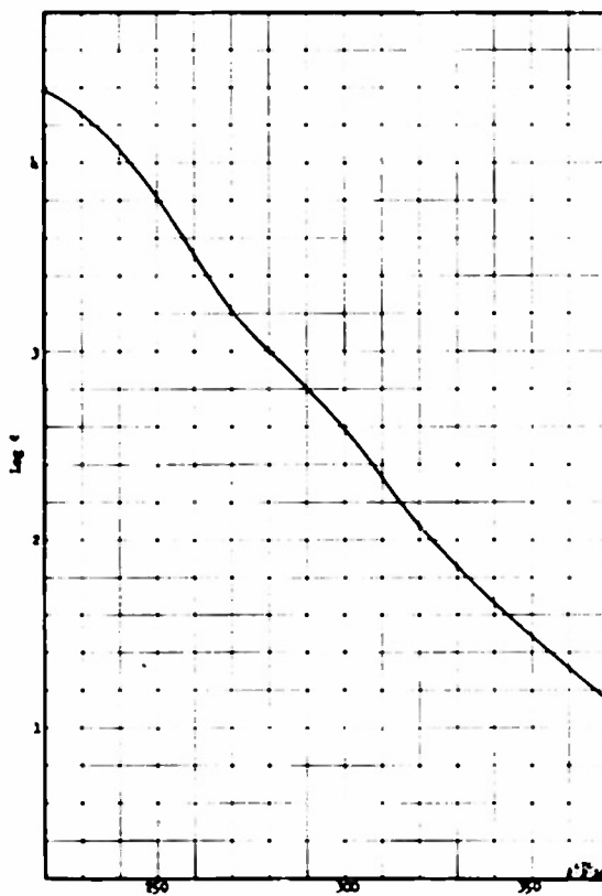
1,1,1,3,5,5,5,7,11,11,11-Trichloro-3,9-dioxo-undecane in Methanol
