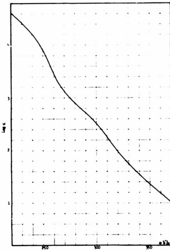
1,1,1,4,6,6,6,11,11,11-Dinitro-2,2-diazo-undecane in Ethanol
