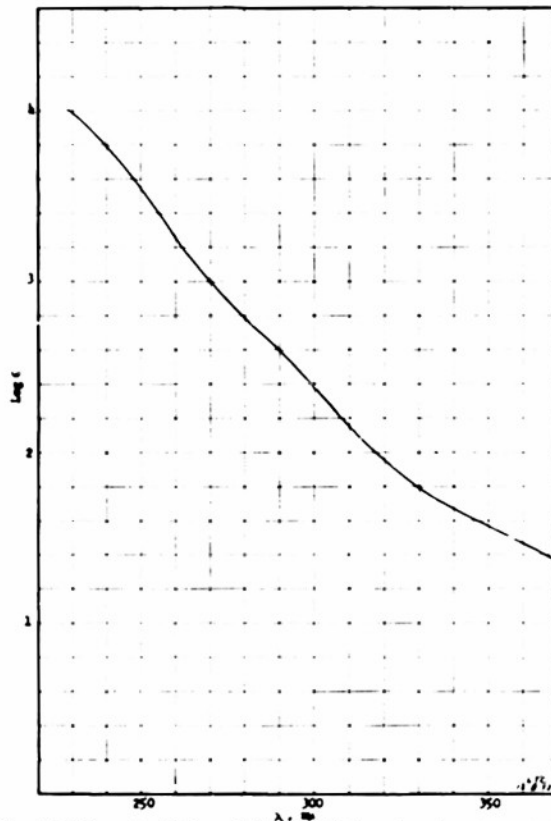
Ultraviolet absorption spectrum of 1,1,1,3,6,6,6-Heptafluoro-3-oxo-hexane in Ethanol
