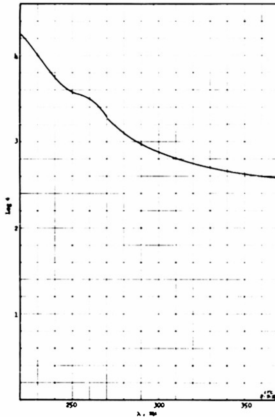
1,1,1,3,5,7,7-Heptafluoro-3,5-dicycloheptane in Ethanol
