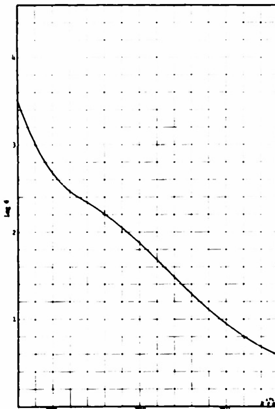
1,1'-Dinitropropyl Amine Nitrate in Benzene
