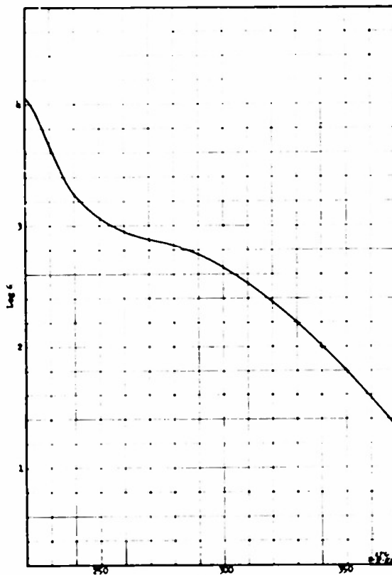
n-D, D, D'-Trinitropropyl-1,3,5,5-tetraazobipiperidine in Ethanol
