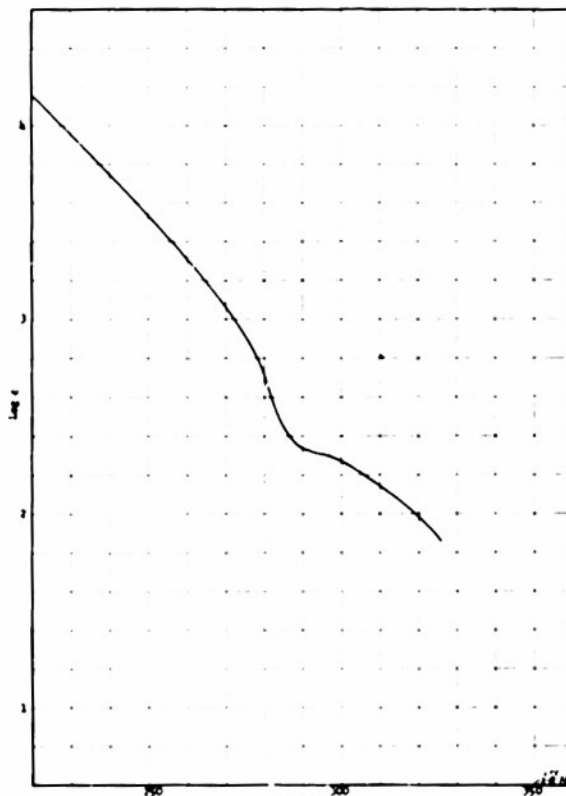
Ultraviolet Absorption Spectrum of 1,1,1,1,5,5,5-Heptafluoro-2,2,2-propylamine in Benzene
