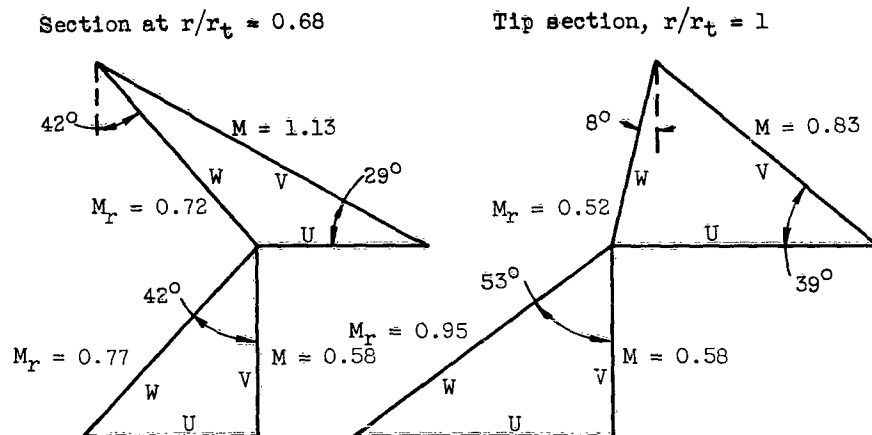
(a) Velocity diagrams.
