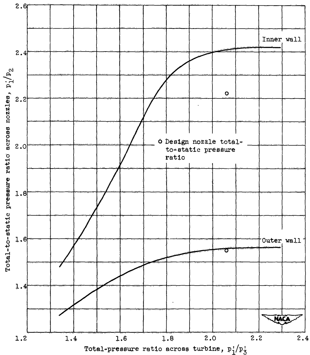
Figure 6. - Effect of total-pressure ratio across turbine on total-to-static pressure ratio across nozzle at design speed.
