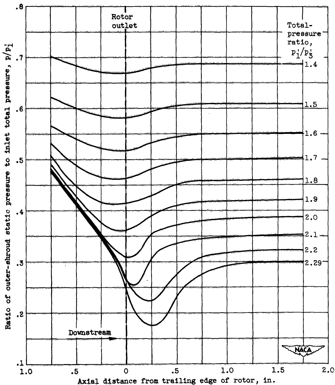
Figure 8. - Effect of total-pressure ratio on outer wall static pressure across rotor tip at design speed.
