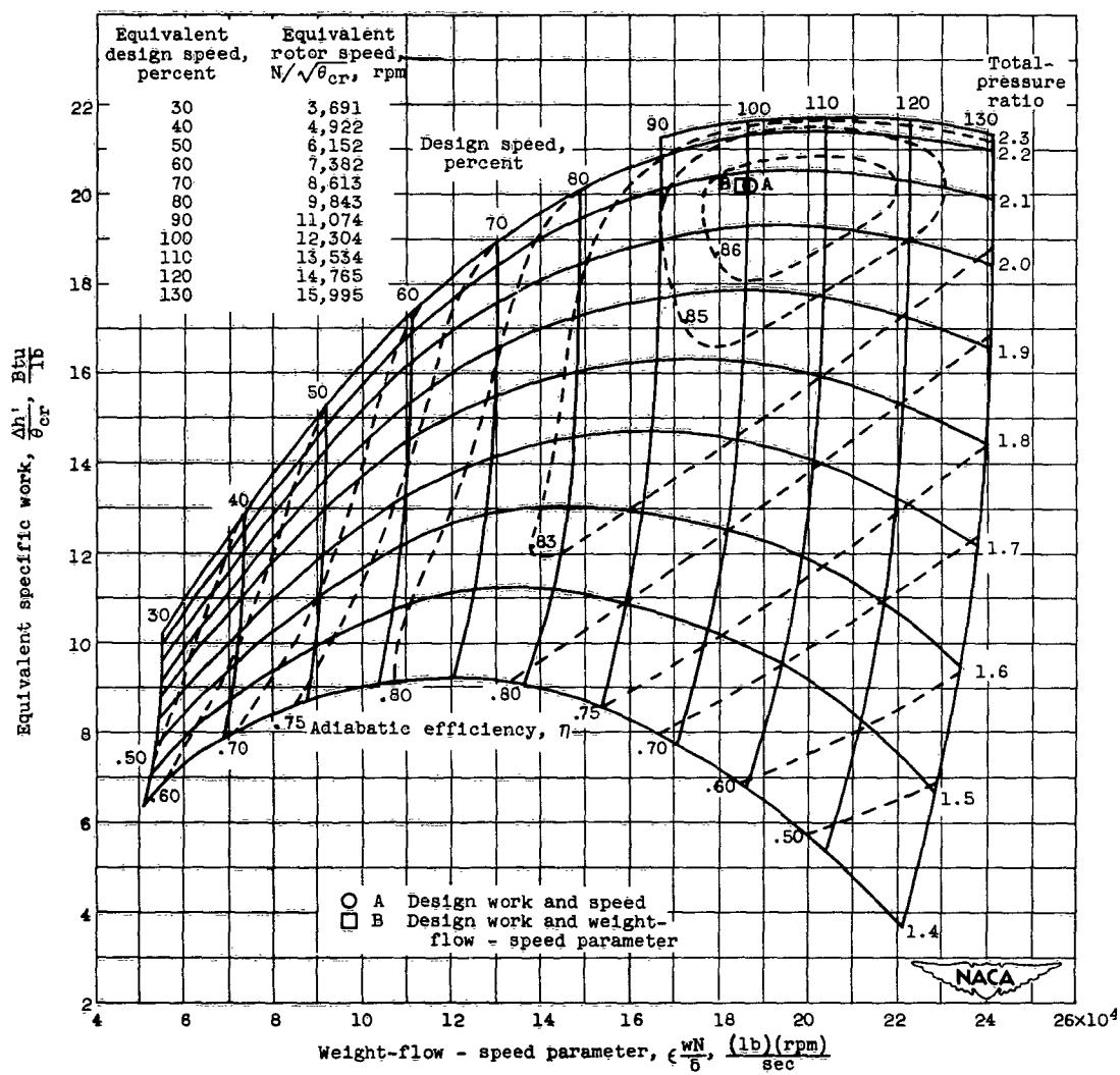
Figure 5. - Over-all performance of turbine.
