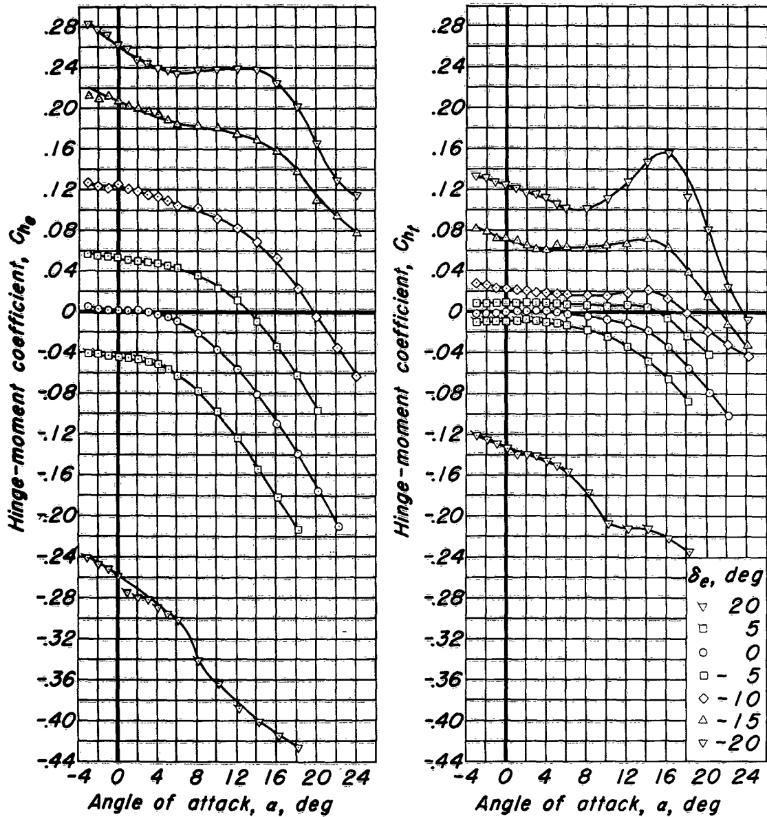
(b) C_{h_e} vs a , C_{h_i} vs a
