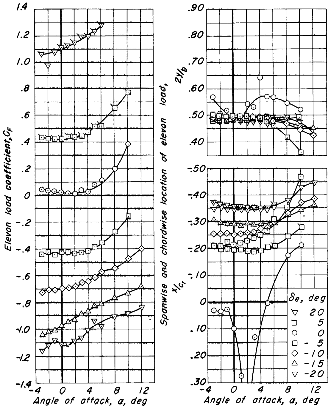
(c) C_F vs a , 2y/b vs a , x/c_r vs a
