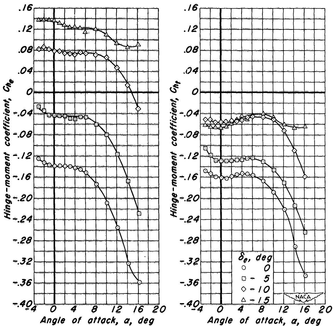
(b) C_{h_e} vs \alpha , C_{h_f} vs \alpha
