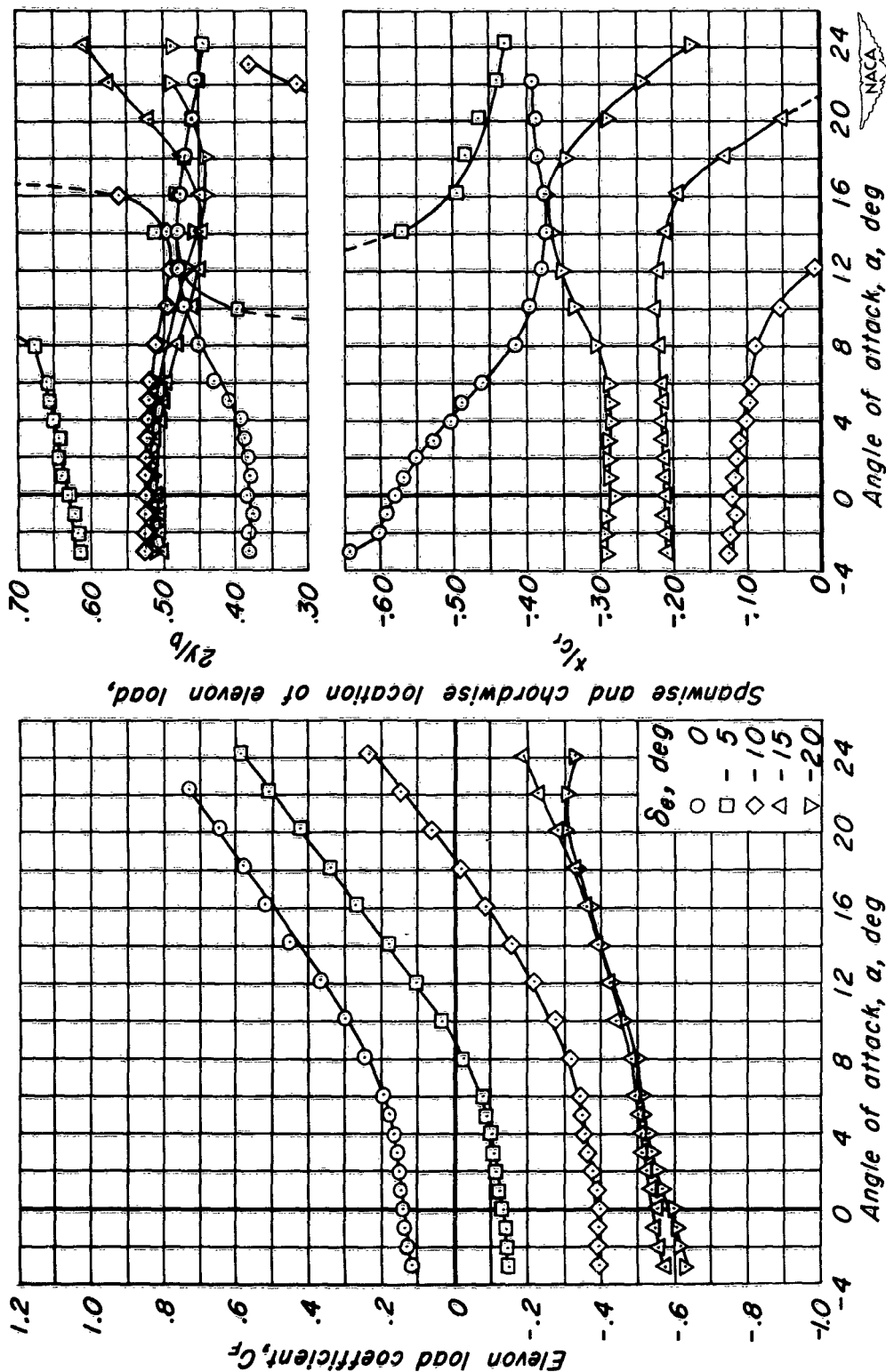
(c) C_F vs a , 2y/b vs a , x/c_i vs a
