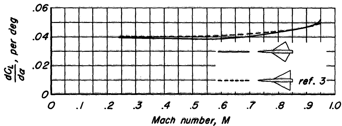
(a) \frac{dC_L}{d\alpha} vs M
