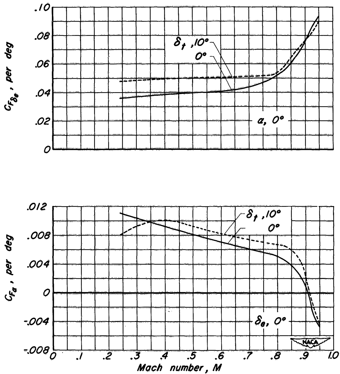
Figure 45.- The effect of Mach number on the elevon load parameters, C_{F\delta_e} and C_{F_a} . R, 3.0 million.
