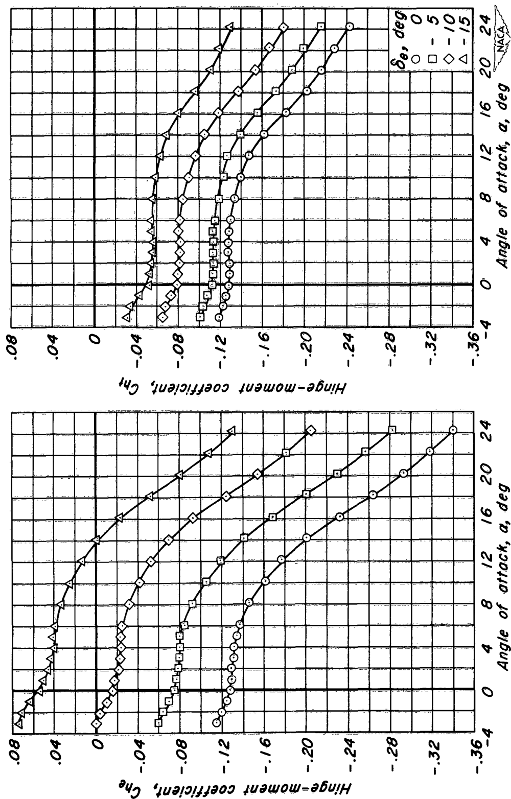
(b) C_{H_e} vs \alpha , C_{H_t} vs \alpha
