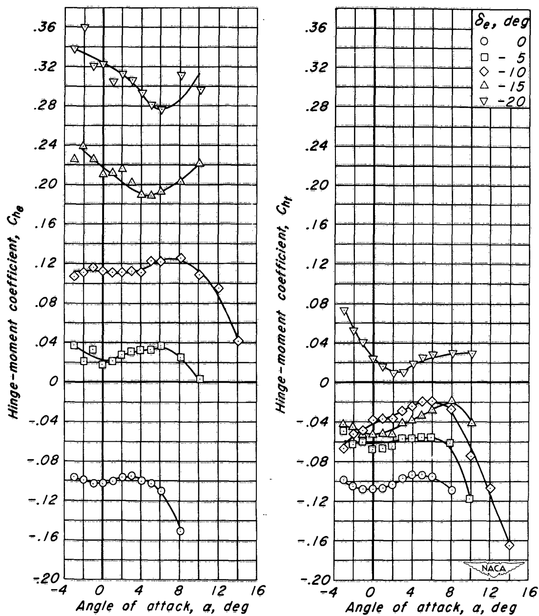
(b) C_{he} vs \alpha , C_{ht} vs \alpha
