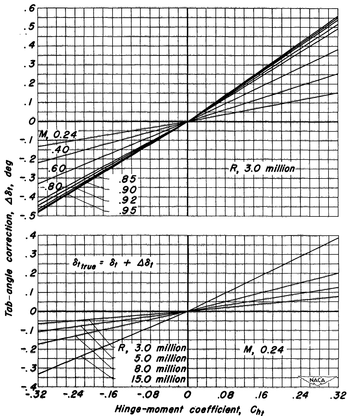
(b) \Delta\delta_t vs C_{hf}
