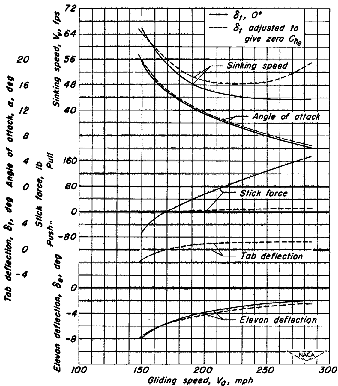
Figure 47.— The gliding characteristics of the assumed airplane with two different longitudinal control systems. Altitude, sea level; wing loading, 40 pounds per square foot; wing area, 450 square feet; center of gravity at 0.25 \bar{c} ; control gearing, 2.0° per inch of stick travel.
