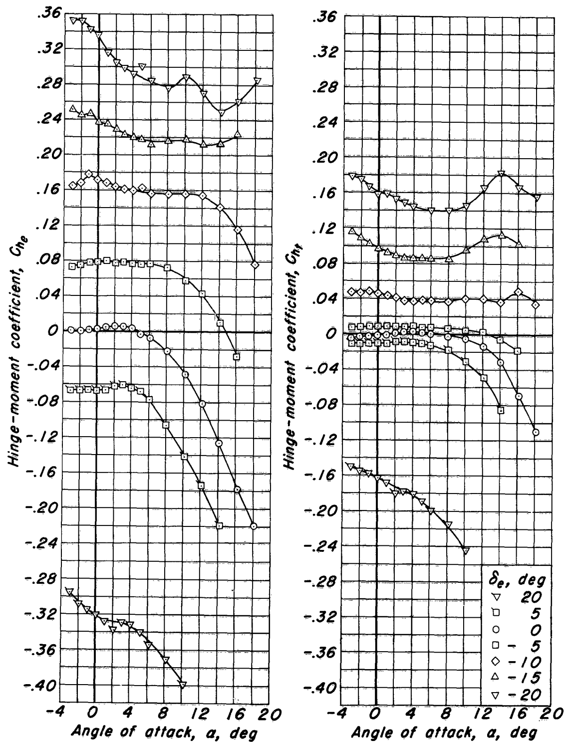
(b) C_{H_e} vs \alpha , C_{H_t} vs \alpha
