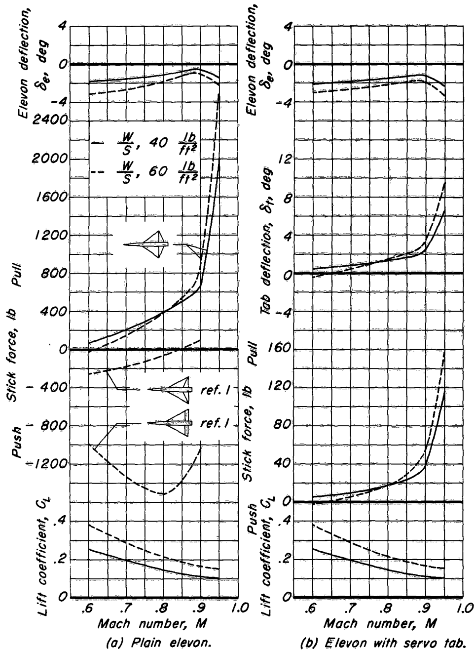
Figure 48.- The effect of wing loading on the level-flight characteristics of the assumed airplane with two different longitudinal control systems. Altitude, 30,000 feet; wing area, 450 square feet; center of gravity at 0.25 \bar{c} ; control gearing, 2.0^\circ per inch of stick travel.
