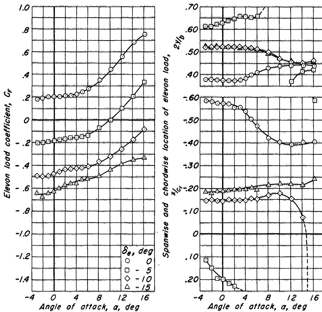
(c) C_F vs \alpha , 2y/b vs \alpha , x/c vs \alpha
