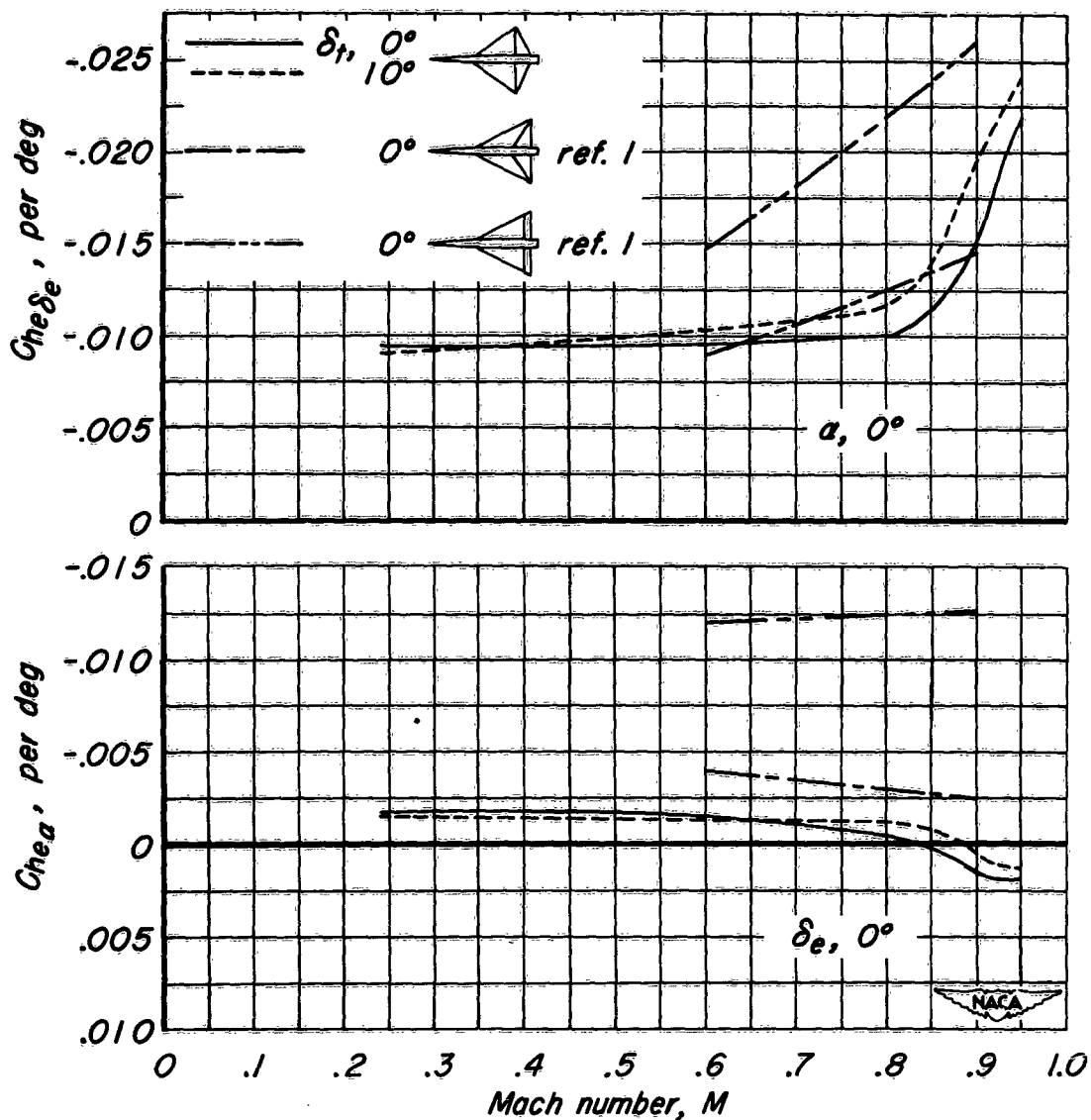
Figure 43.-The variation with Mach number of the elevon-hinge-moment parameters, C_{he\delta_e} and C_{he\alpha} , for various elevon plan forms. R , 3.0 million.
