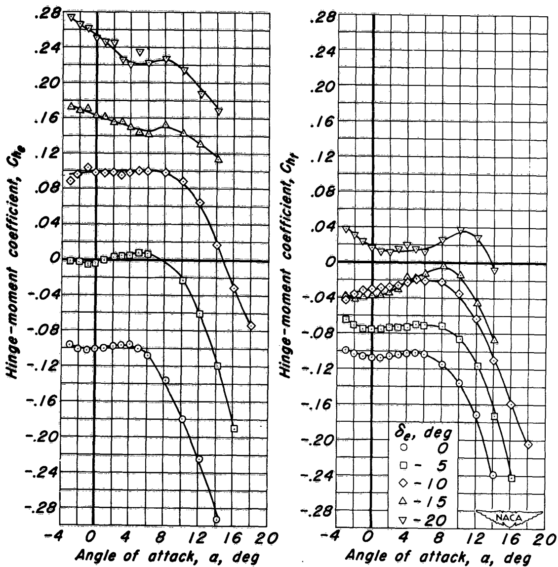
(b) C_{h_e} vs \alpha , C_{h_f} vs \alpha
