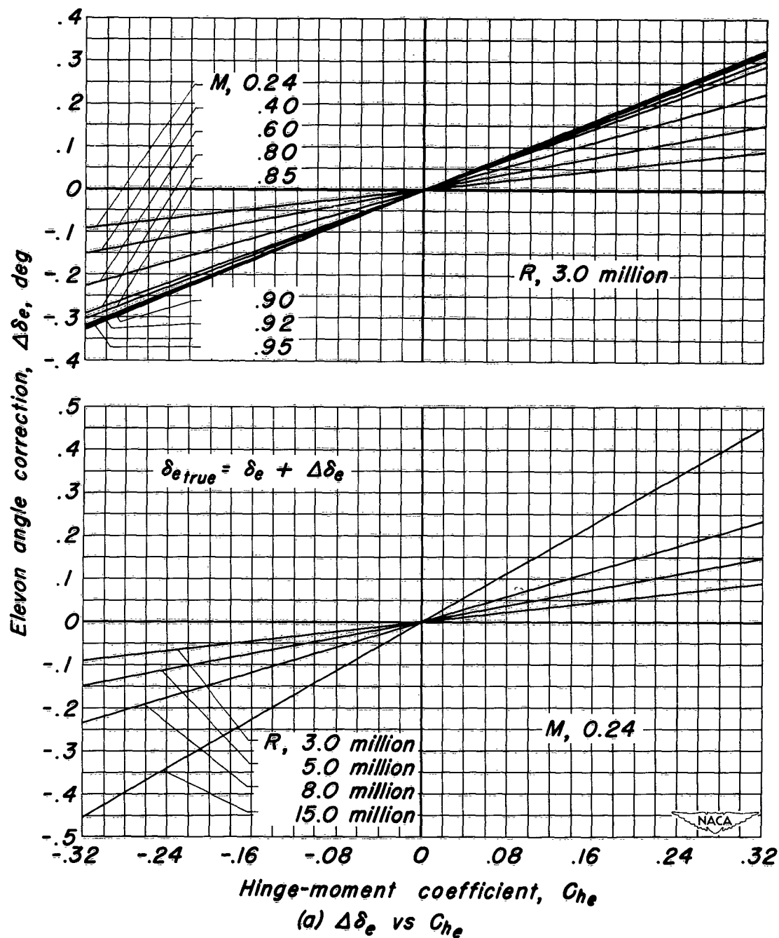
Figure 3.- The variation with hinge-moment coefficient of the elevon and tab-angle corrections, \Delta\delta , at various Mach numbers and Reynolds numbers.
