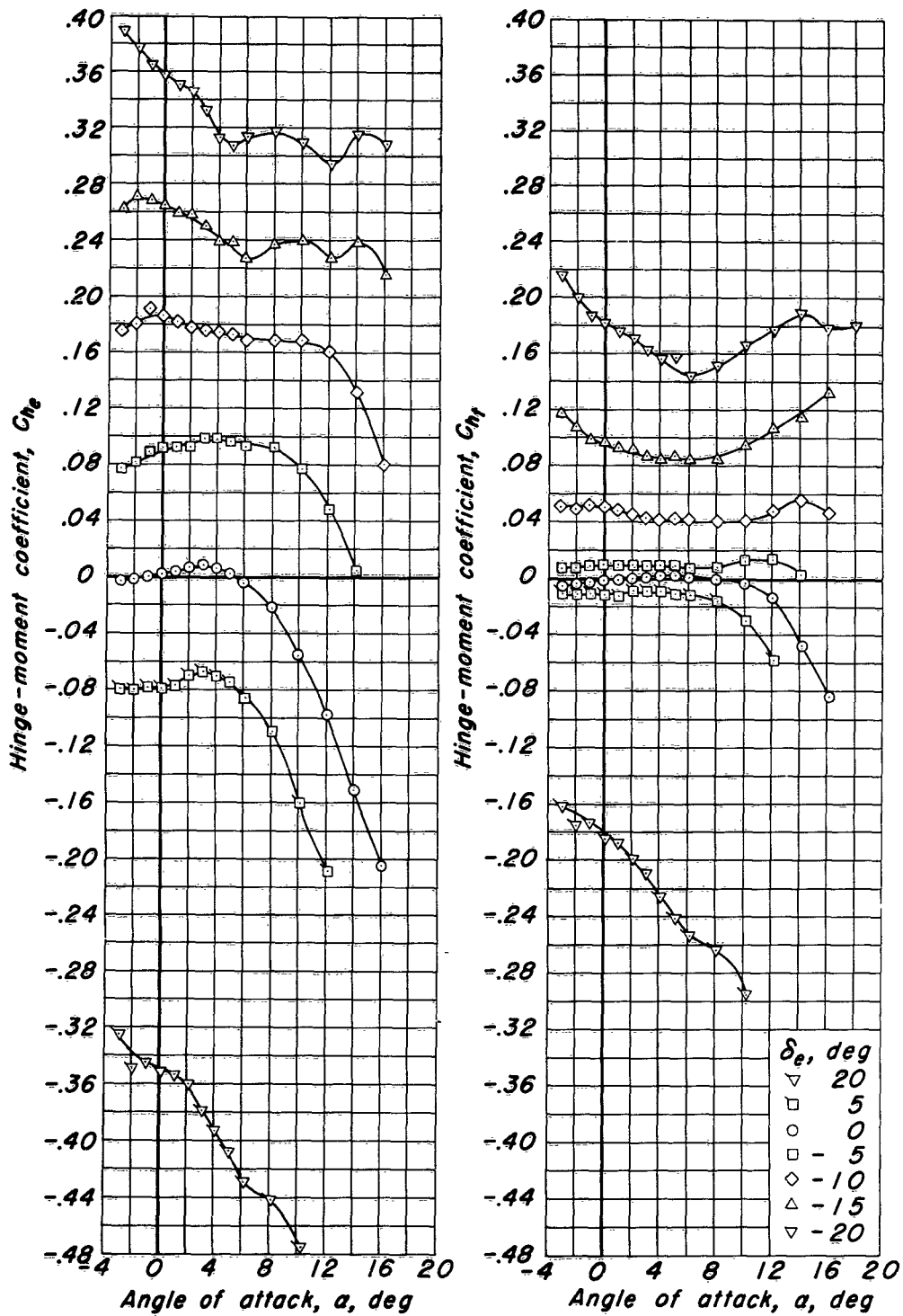
(b) C_{H_e} vs \alpha , C_{H_f} vs \alpha Figure 10.- Continued.
