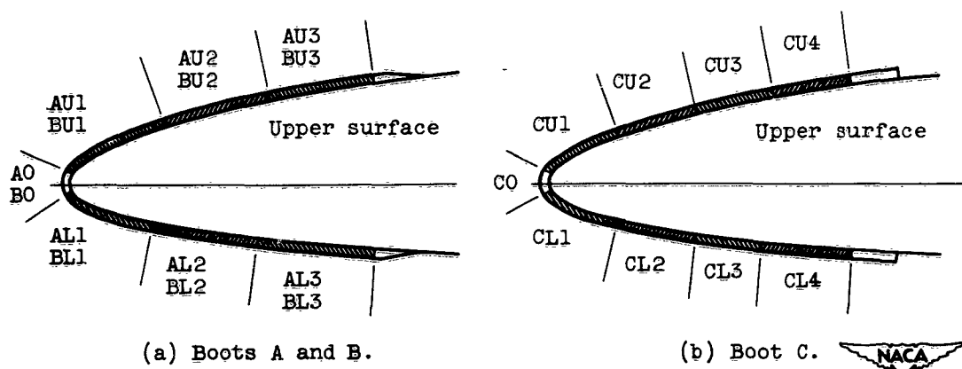
Figure 3. - Segment notation for de-icing boots used in investigation.
