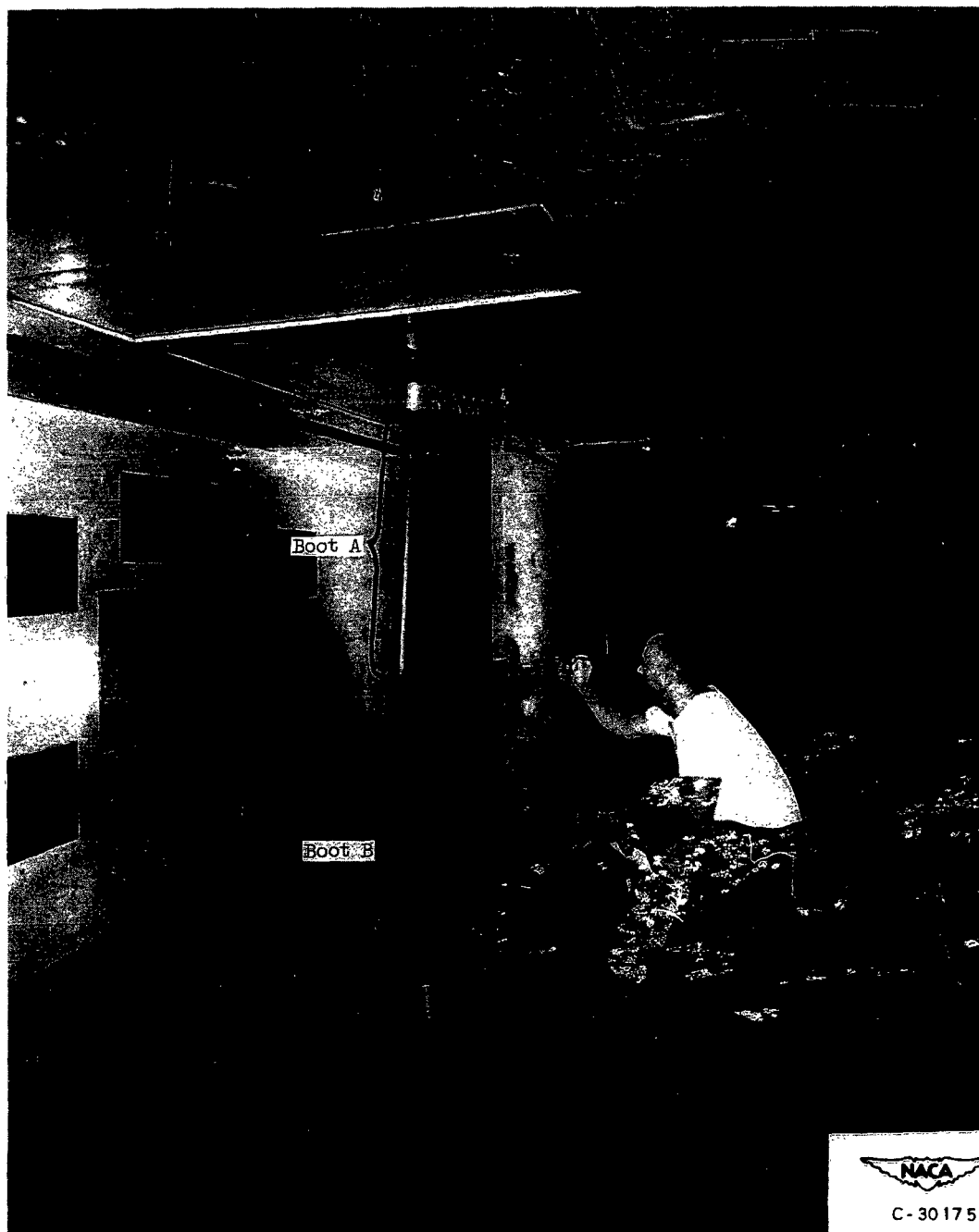
Figure 1. - Installation of airfoil model in test section of icing research tunnel.
