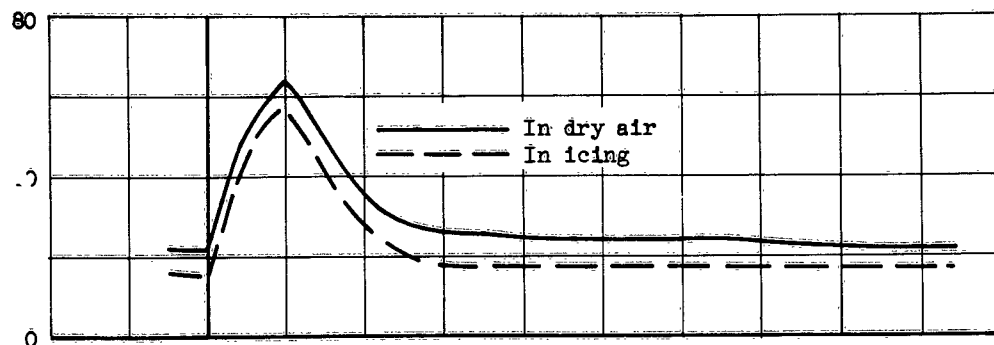
(a) Boot segment AU1. Surface distance/chord length, 3.63 percent.
