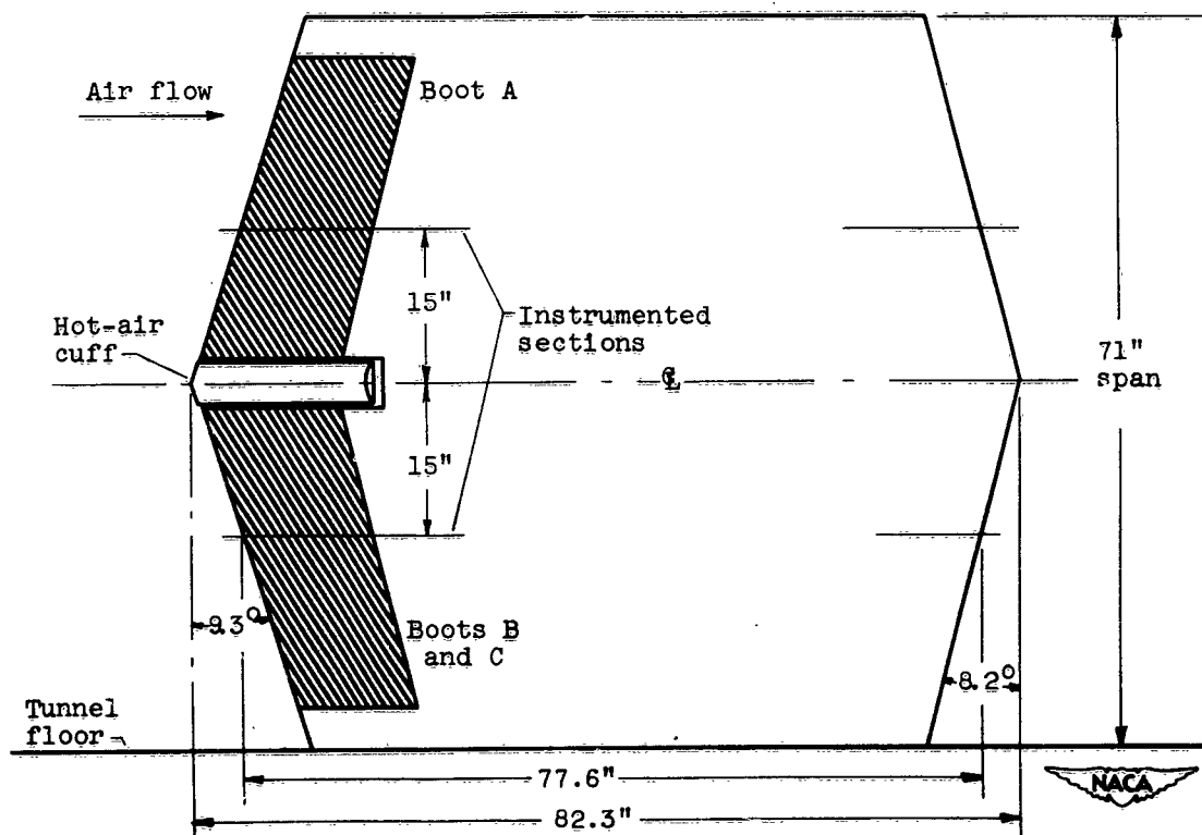
Figure 6. - Airfoil model employed in investigation.
