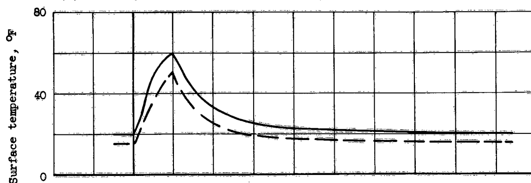
(b) Boot segment BU1. Surface distance/chord length, 3.54 percent.
