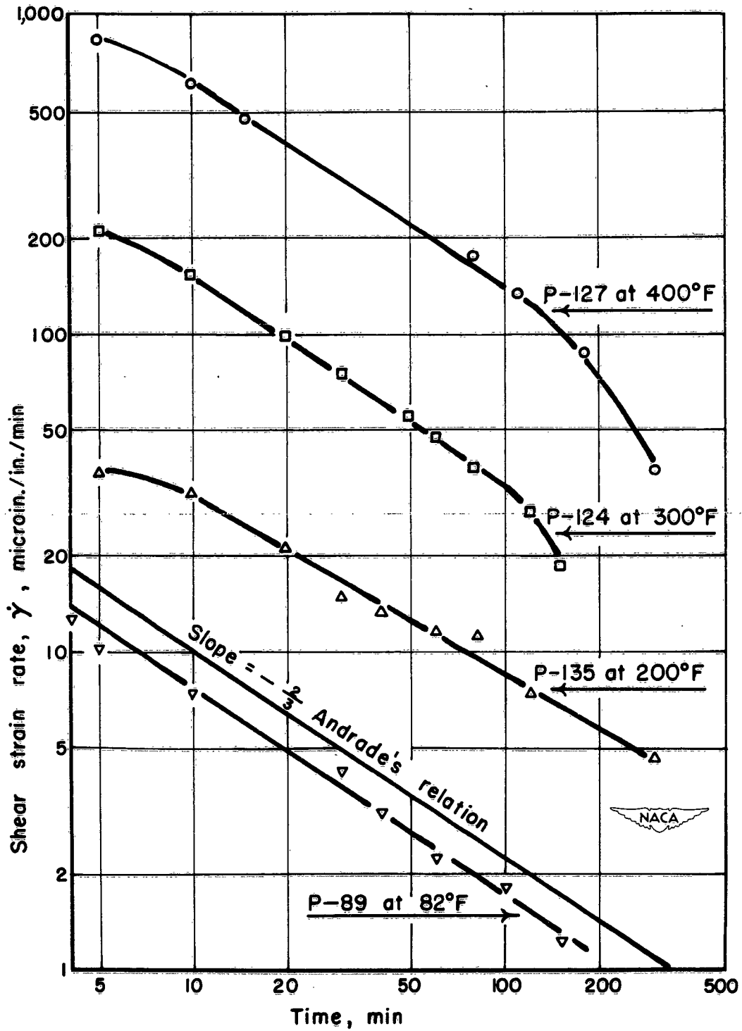
(b) 300-psi resolved shear stress.
