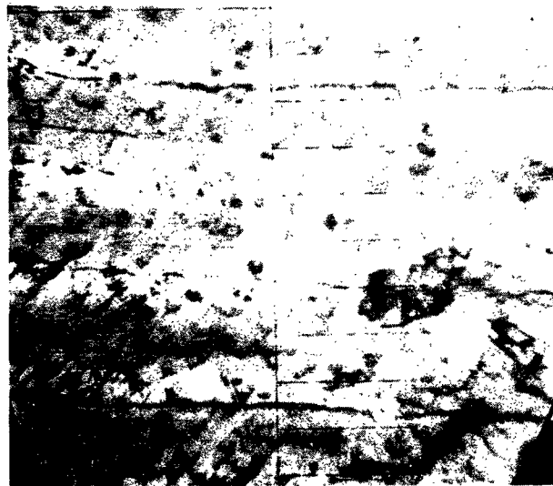
(a) Specimen P-115; test, 300-psi resolved shear stress at 200° F; surface, chemically polished; total extension, 0.6 percent.
