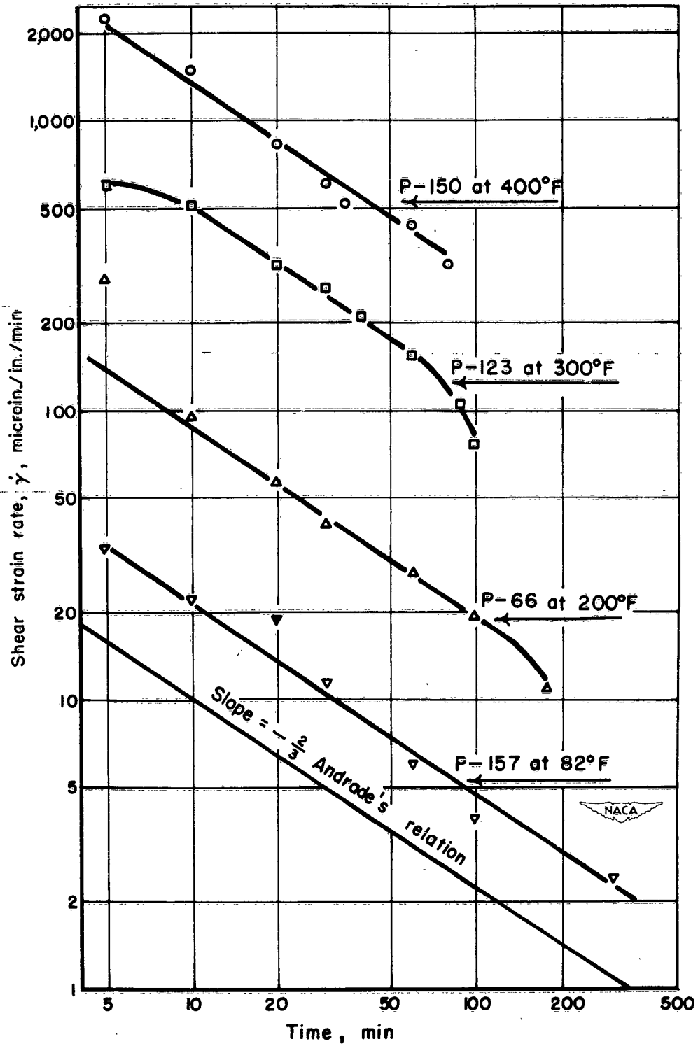
(c) 400-psi resolved shear stress.
