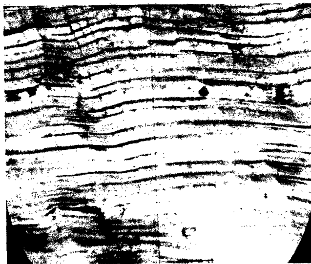
(a) Specimen P-163; test, constant-load-rate at 200° F; surface, chemically polished; total extension, 18 percent; taken approximately parallel to \theta -direction of slip plane; X400.
